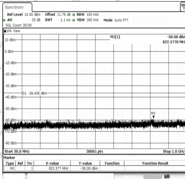
11N40SISO-Ant1-2422-30~1000-PASS
