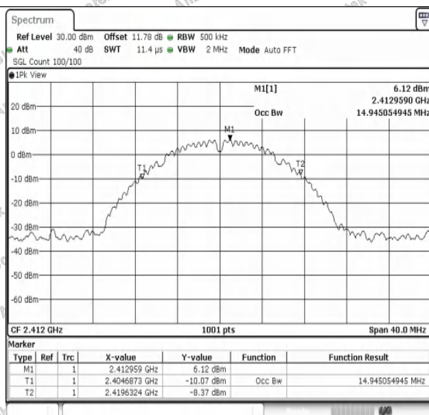
11B-Ant1-2412
