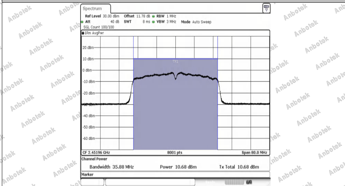
11N40SISO-Ant1-2452-PASS
