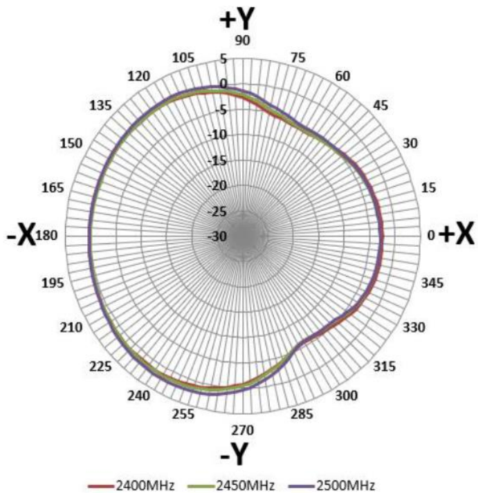
X-Y PLANE
