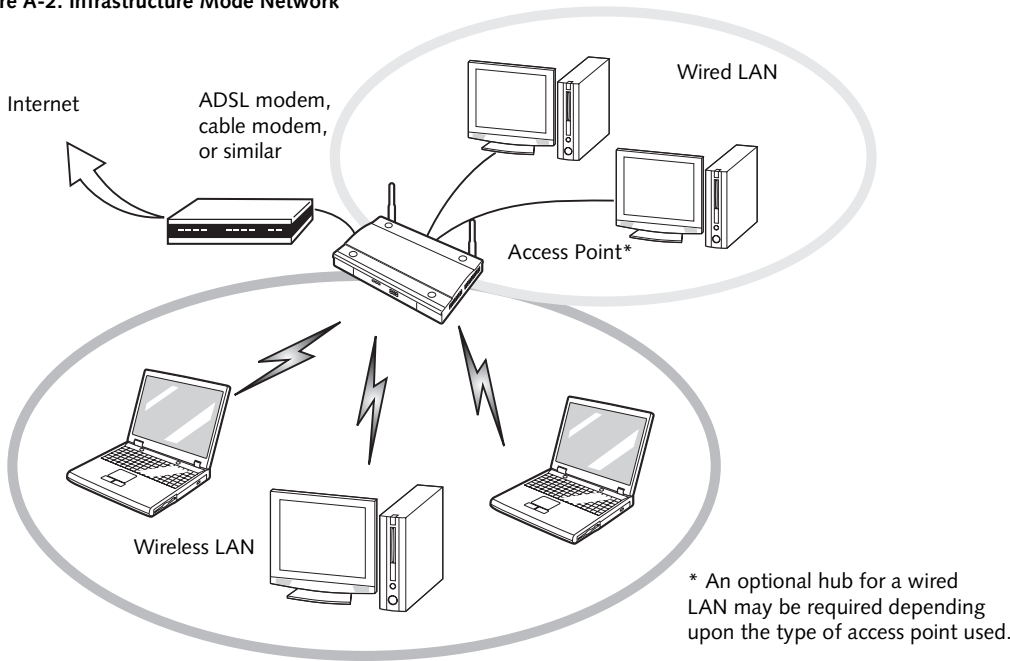
Figure A-2. Infrastructure Mode Network
