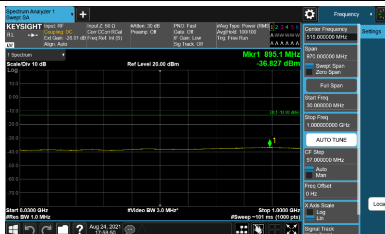
Band41-10MHz-256QAM-40620-E-TM3.1A-30~1000
