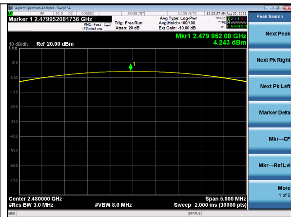
Output Power, BT Classic, QPSK Channel 79
