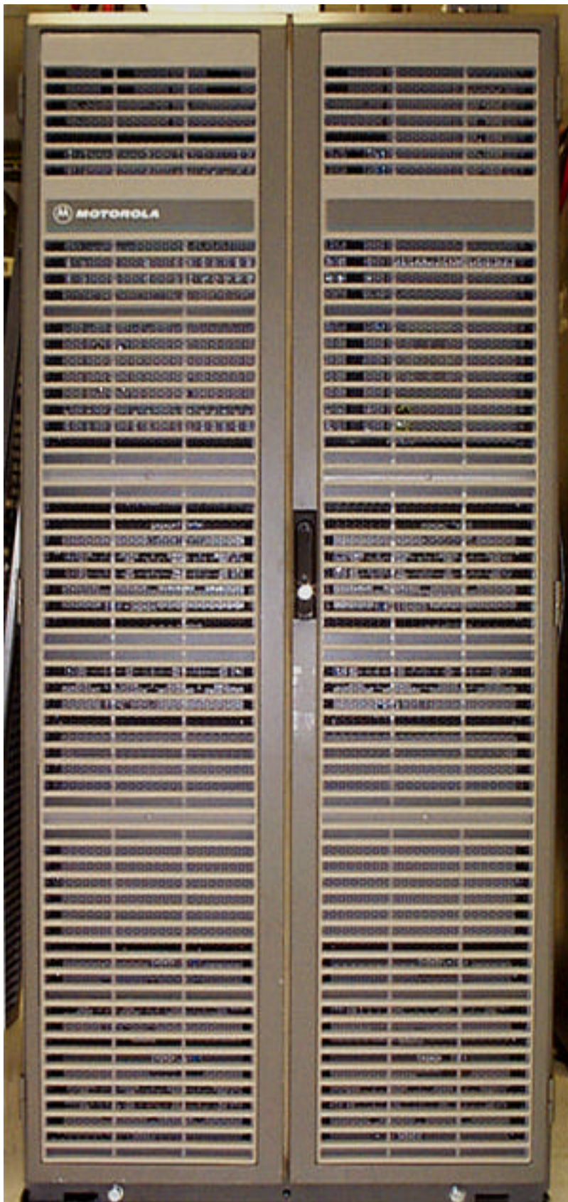
IRET5BL1 SC4812T @ 800 MHz Front View Door Closed
