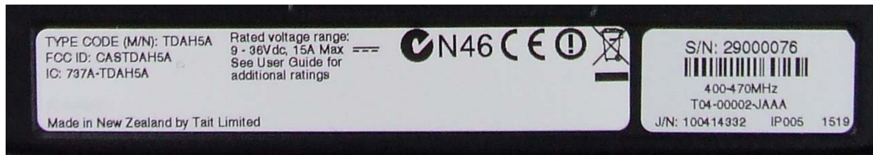
Photograph 01: Compliance Label
