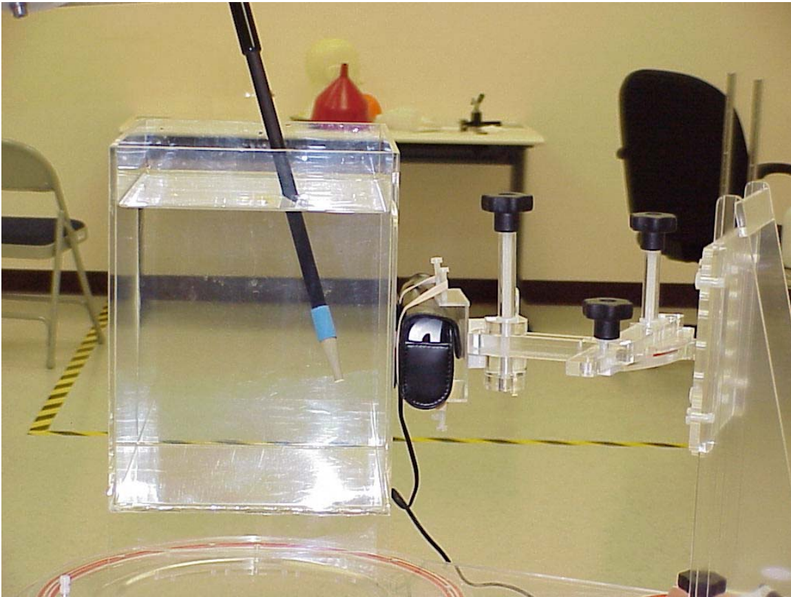
Photo 7. Body SAR with headset
