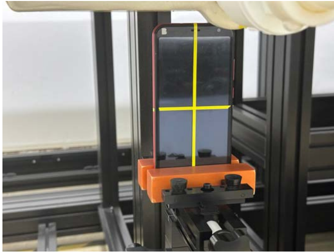
Top Side (Test distance: 10mm)
