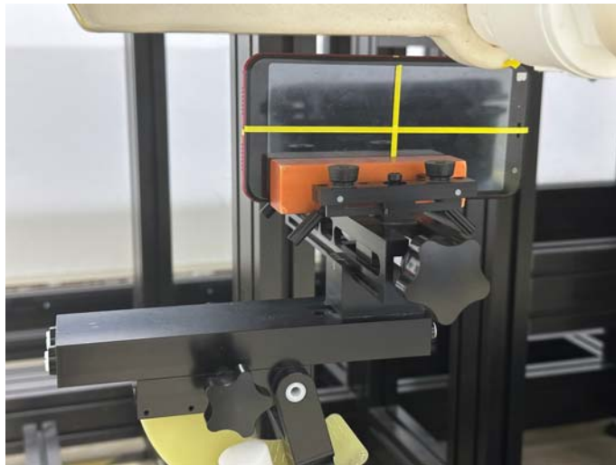
Left Side (Test distance: 10mm)
