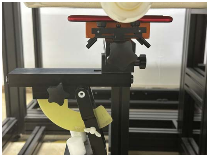
Back Side (Test distance: 10mm)
