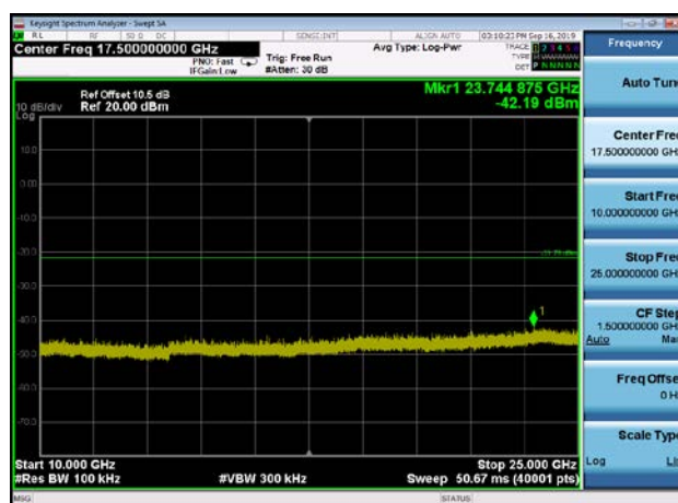
,Plot 5,10000MHz~25000MHz-802.11n(HT4 0),2452MHz,Ant1
