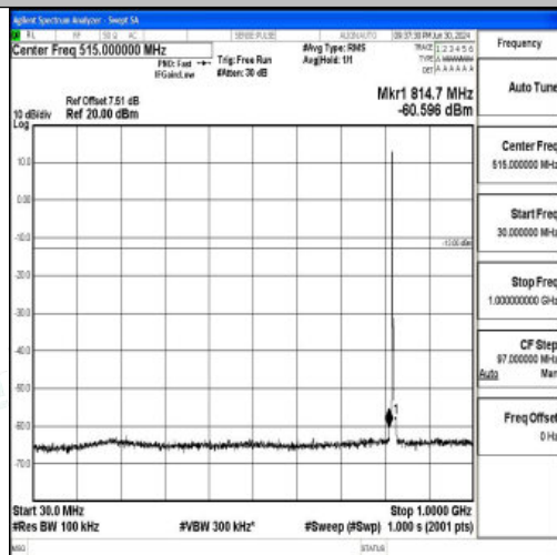
Band26_3MHz_QPSK_26775_1RB#0_30~1000_30~1000
