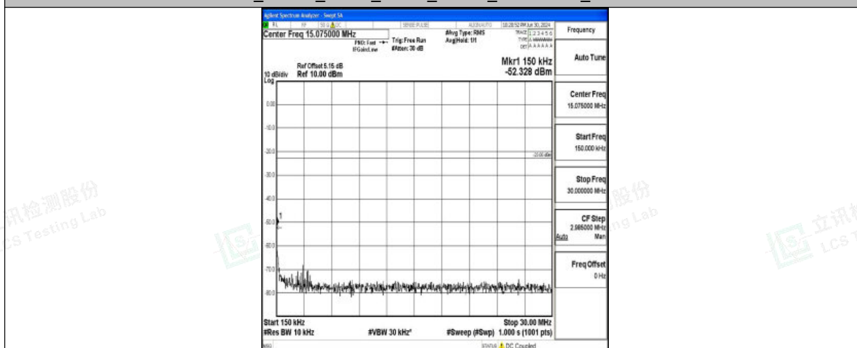
Band26_10MHz_QPSK_26740_1RB#0_0.15~30_0.15~30
