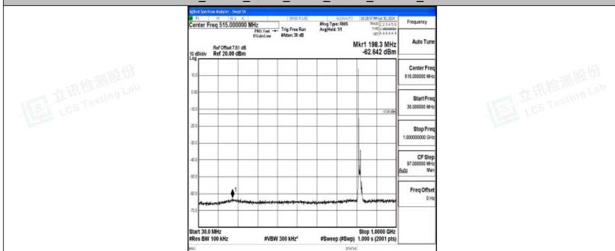
Band26_10MHz_QPSK_26740_1RB#0_30~1000_30~1000
