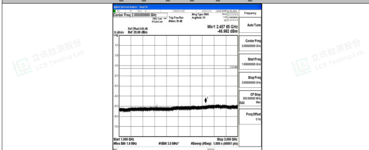
Band26_5MHz_QPSK_26765_1RB#0_1000~3000_1000~3000
