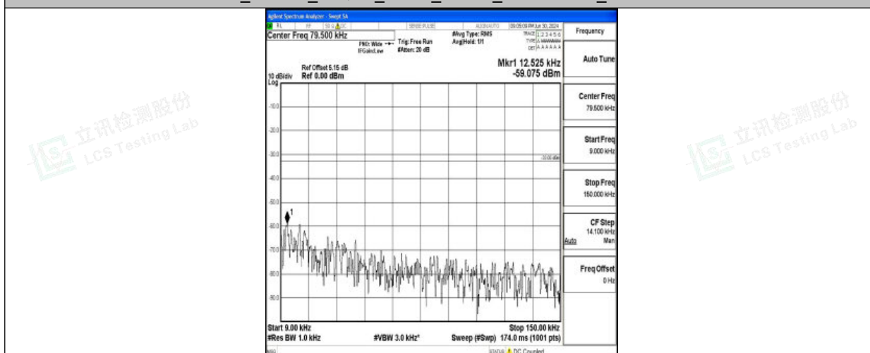
Band26_1.4MHz_QPSK_26783_1RB#0_0.009~0.15_0.009~0.15
