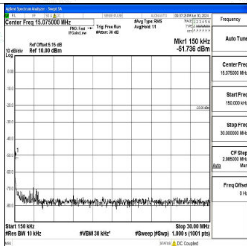
Band26_3MHz_QPSK_26775_1RB#0_0.15~30_0.15~30
