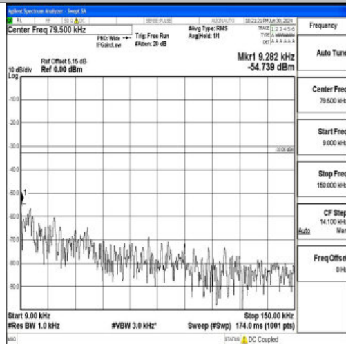
Band26 10MHz 16QAM 26740 1RB#0 0.009~0.15 0.009~0.15
