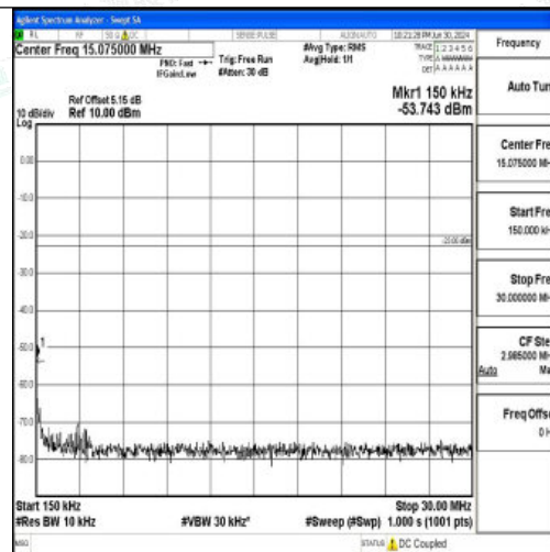
Band26_10MHz_16QAM_26740_1RB#0_0.15~30_0.15~30
