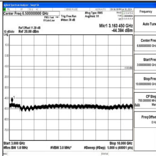
Band26_3MHz_QPSK_26740_1RB#0_3000~10000_3000~10000
