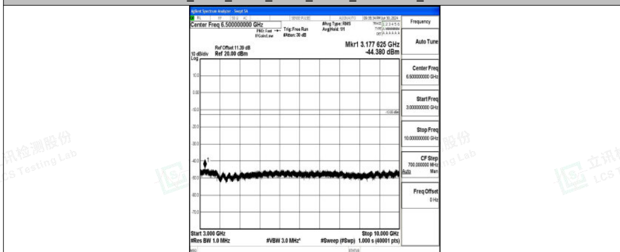
Band26_3MHz_QPSK_26705_1RB#0_3000~10000_3000~10000
