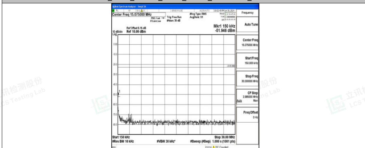
Band26_5MHz_16QAM_26740_1RB#0_0.15~30_0.15~30
