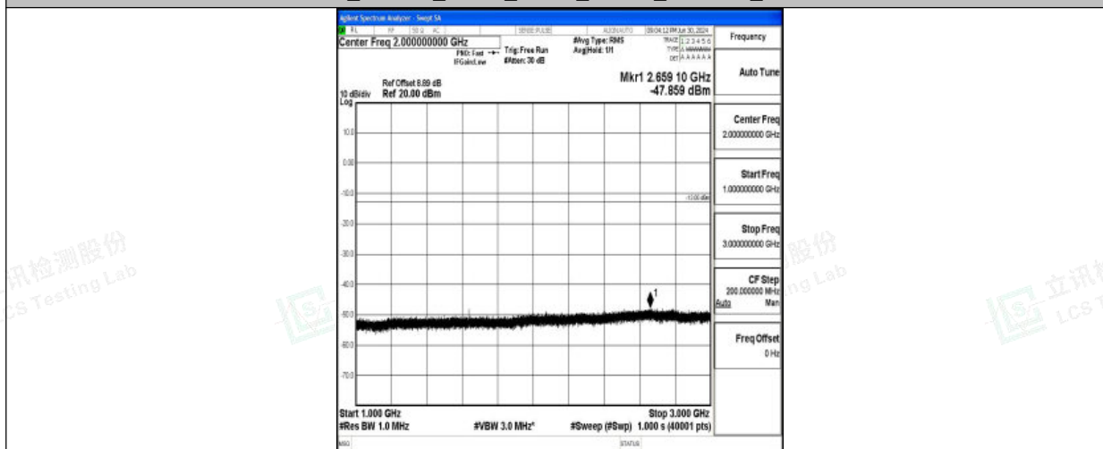
Band26_1.4MHz_QPSK_26740_1RB#0_1000~3000_1000~3000
