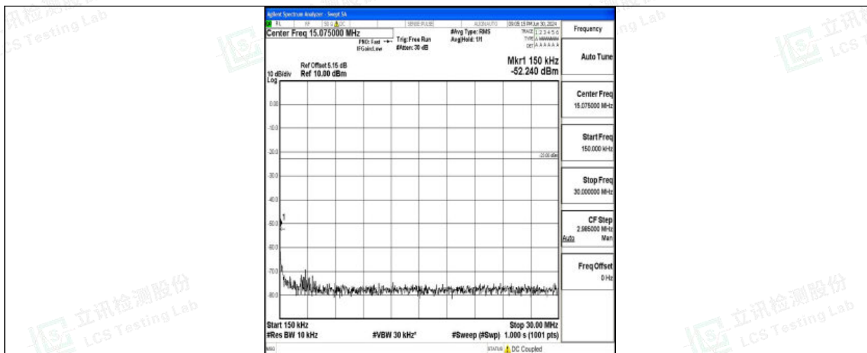
Band26_1.4MHz_QPSK_26783_1RB#0_0.15~30_0.15~30
