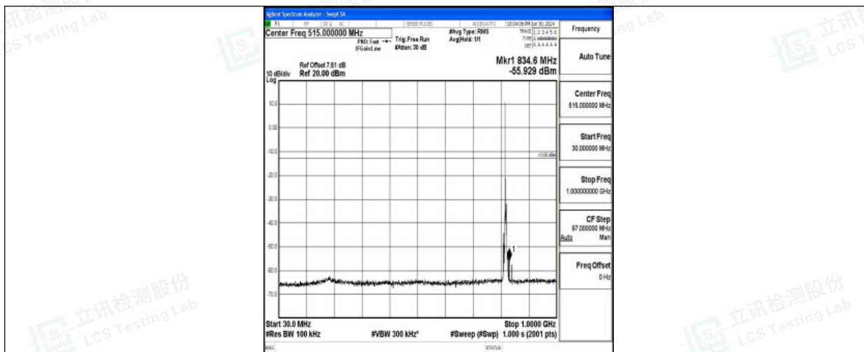
Band26_5MHz_16QAM_26765_1RB#0_30~1000_30~1000
