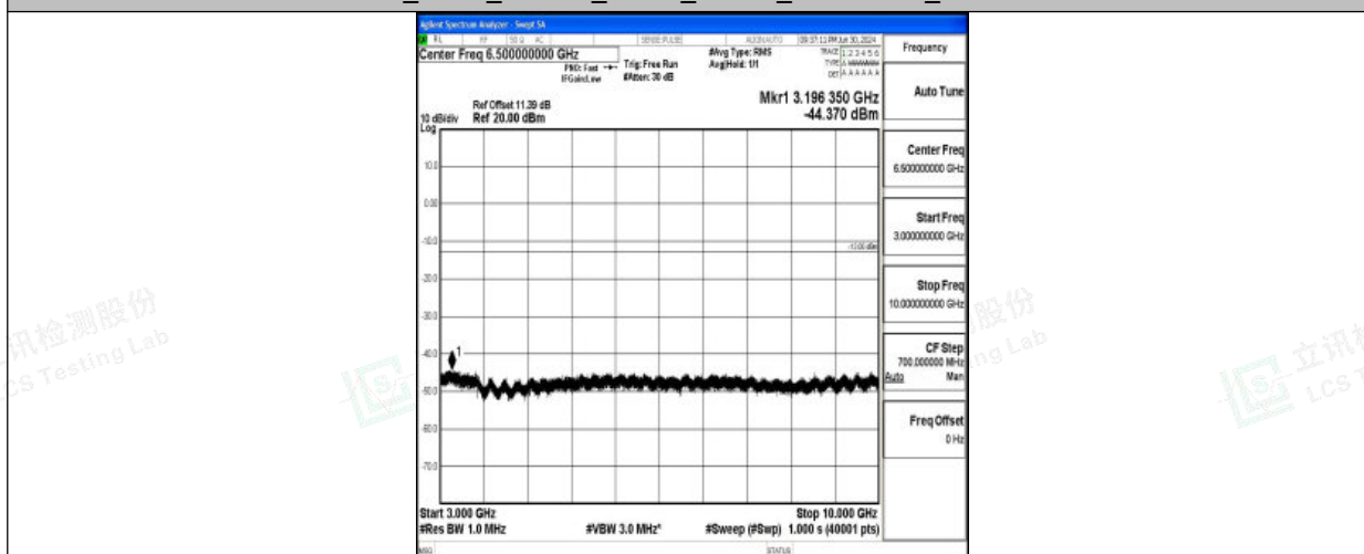
Band26_3MHz_16QAM_26740_1RB#0_3000~10000_3000~10000
