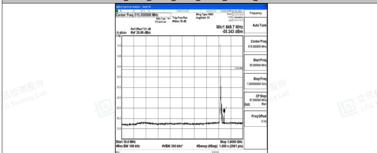
Band26_5MHz_QPSK_26765_1RB#0_30~1000_30~1000
