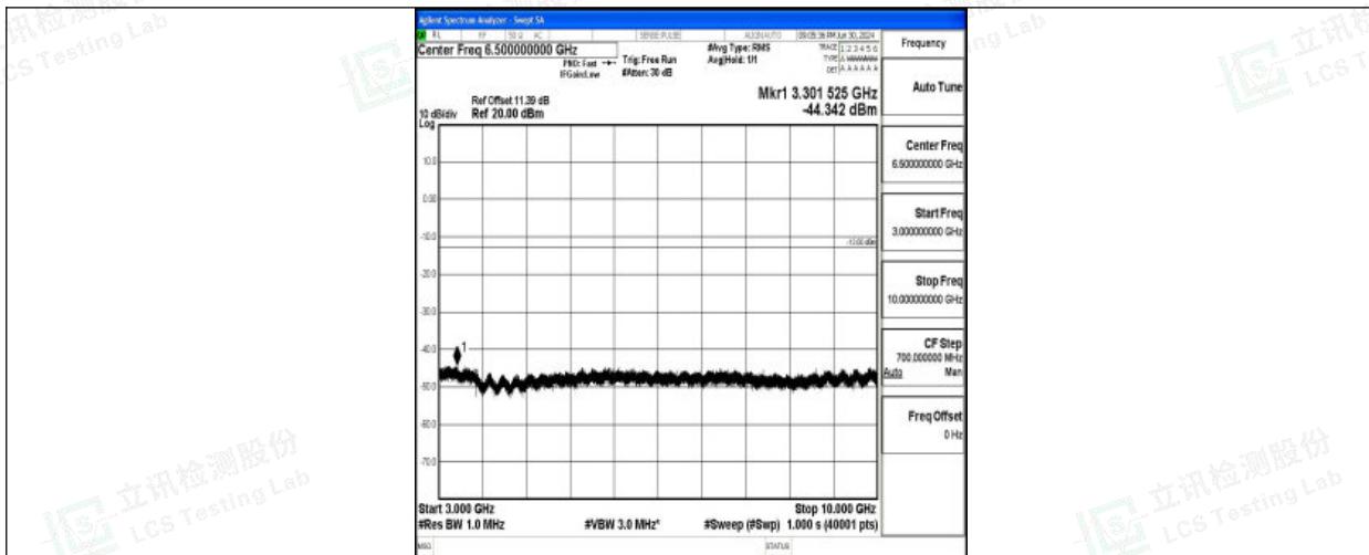
Band26_1.4MHz_QPSK_26783_1RB#0_3000~10000_3000~10000
