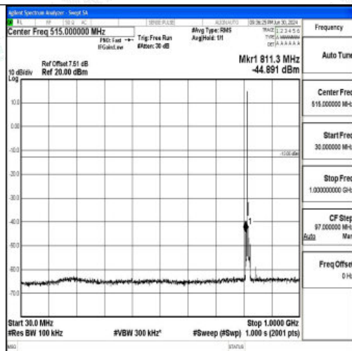
Band26_3MHz_QPSK_26740_1RB#0_30~1000_30~1000
