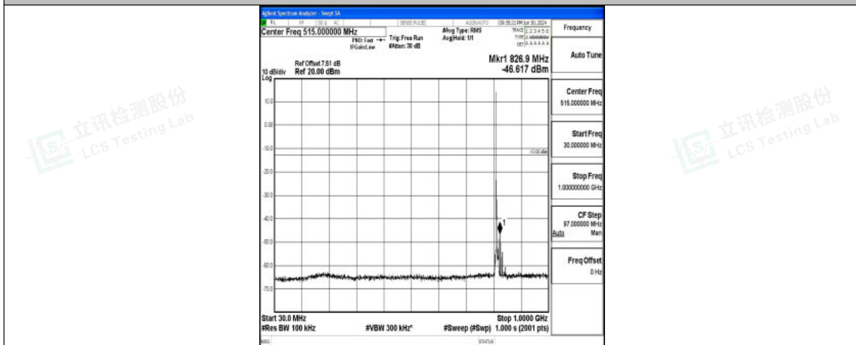
Band26_3MHz_QPSK_26705_1RB#0_30~1000_30~1000
