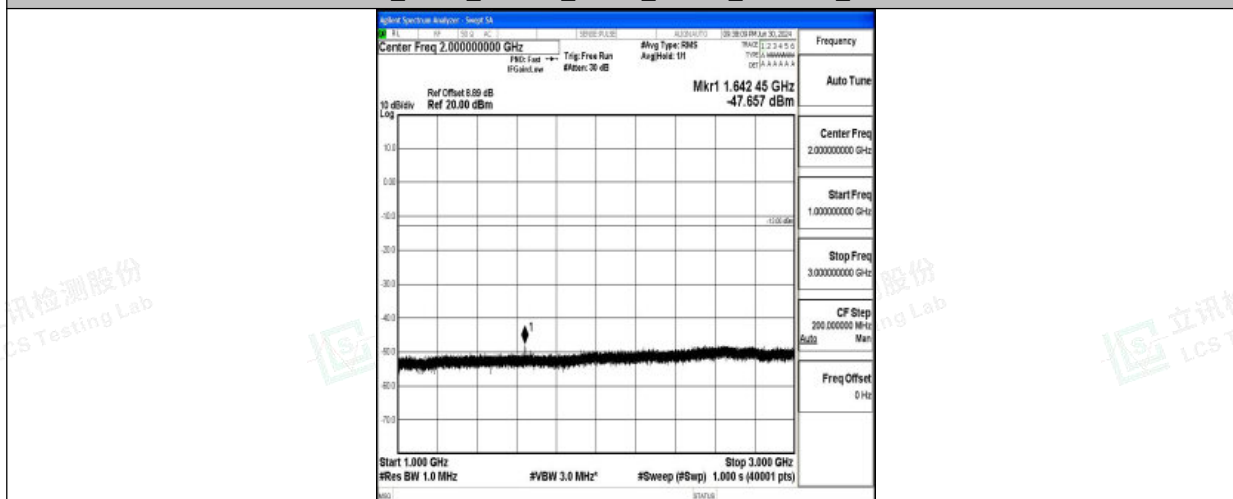
Band26_3MHz_16QAM_26775_1RB#0_1000~3000_1000~3000
