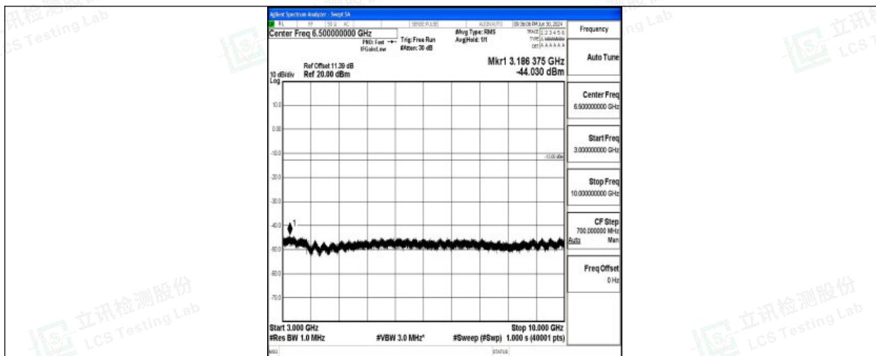
Band26_3MHz_16QAM_26705_1RB#0_3000~10000_3000~10000
