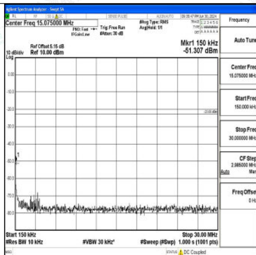
Band26_3MHz_16QAM_26705_1RB#0_0.15~30_0.15~30
