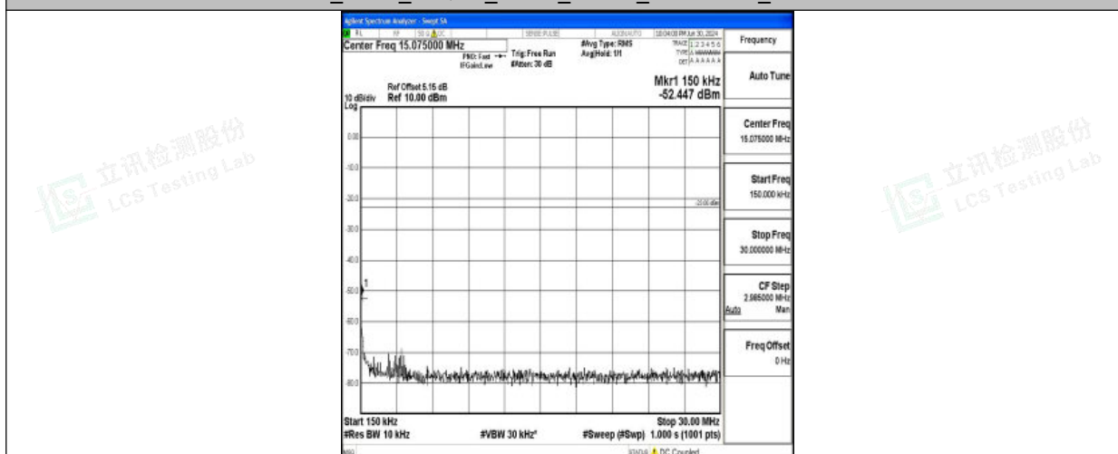
Band26_5MHz_16QAM_26765_1RB#0_0.15~30_0.15~30
