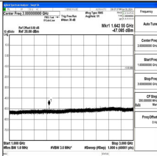
Band26_3MHz_QPSK_26775_1RB#0_1000~3000_1000~3000
