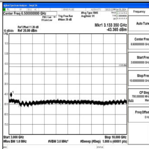
Band26 10MHz QPSK 26740 1RB#0 3000~10000 3000~10000
