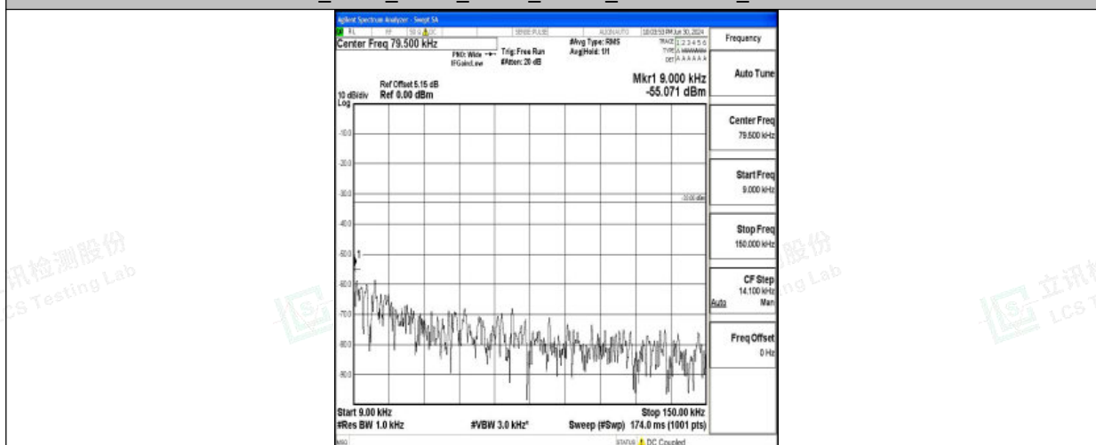
Band26_5MHz_16QAM_26765_1RB#0_0.009~0.15_0.009~0.15
