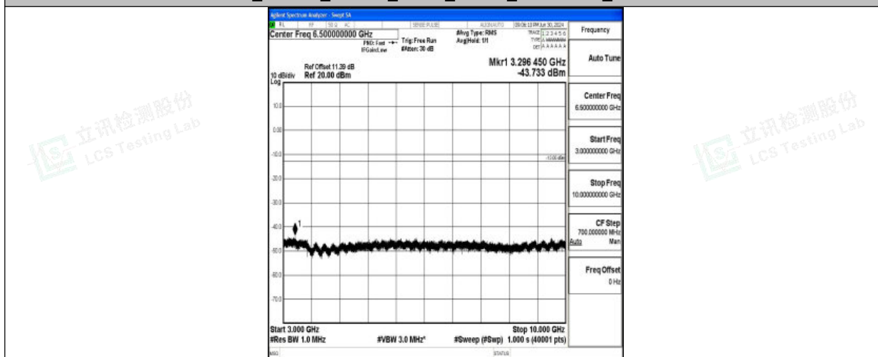
Band26_1.4MHz_16QAM_26783_1RB#0_3000~10000_3000~10000
