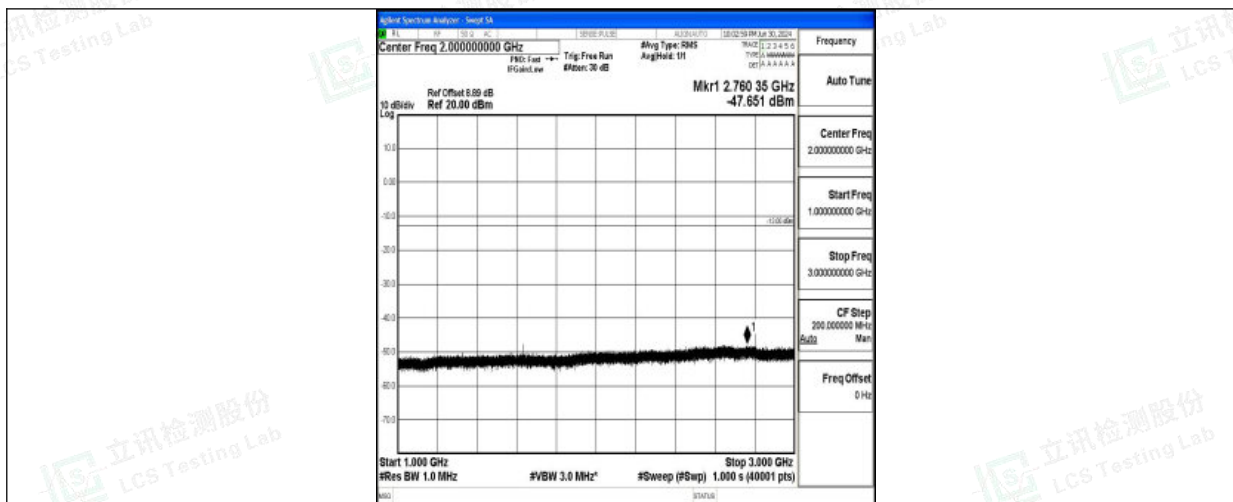
Band26_5MHz_16QAM_26740_1RB#0_1000~3000_1000~3000
