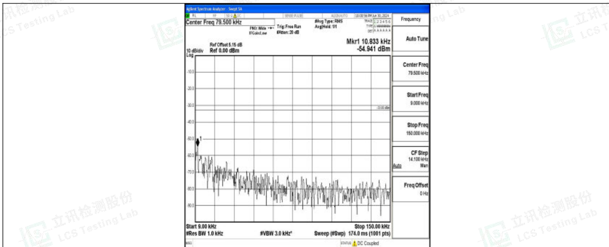
Band26_5MHz_QPSK_26715_1RB#0_0.009~0.15_0.009~0.15
