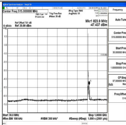
Band26_3MHz_16QAM_26705_1RB#0_30~1000_30~1000
