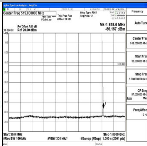
Band26_1.4MHz_16QAM_26697_1RB#0_30~1000_30~1000
