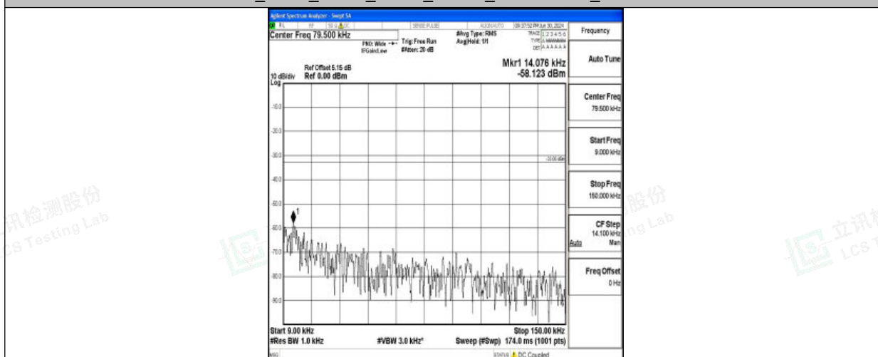
Band26_3MHz_16QAM_26775_1RB#0_0.009~0.15_0.009~0.15
