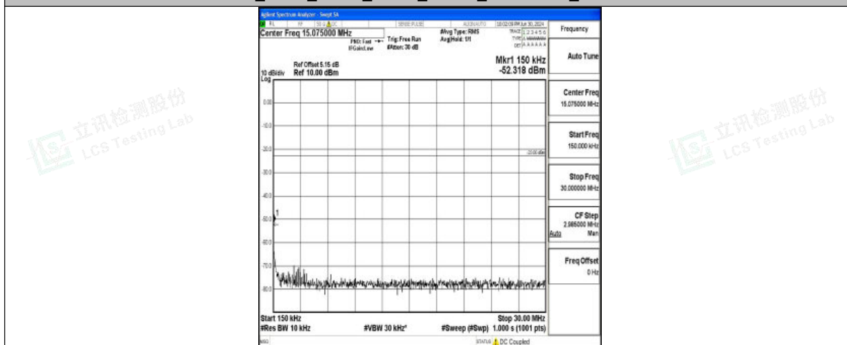
Band26_5MHz_QPSK_26740_1RB#0_0.15~30_0.15~30
