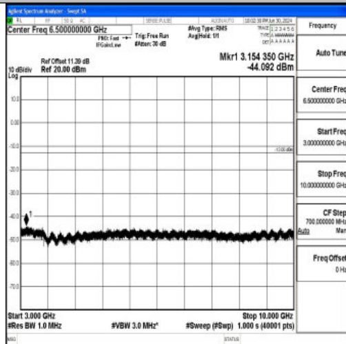
Band26_5MHz_QPSK_26740_1RB#0_3000~10000_3000~10000
