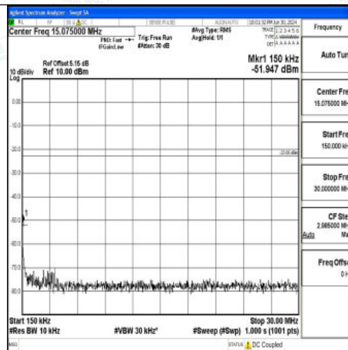
Band26_5MHz_16QAM_26715_1RB#0_0.15~30_0.15~30
