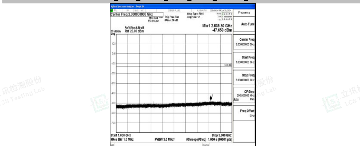
Band26_5MHz_16QAM_26765_1RB#0_1000~3000_1000~3000
