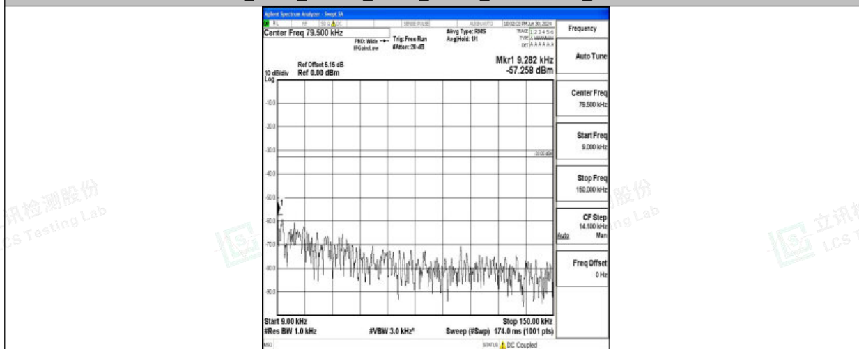
Band26_5MHz_QPSK_26740_1RB#0_0.009~0.15_0.009~0.15
