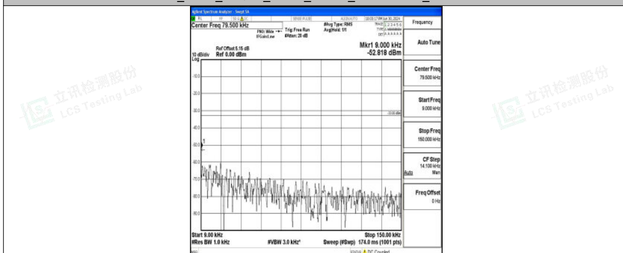
Band26_5MHz_QPSK_26765_1RB#0_0.009~0.15_0.009~0.15
