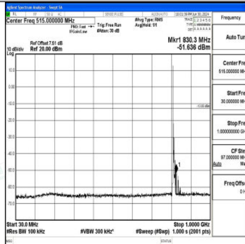
Band26_5MHz_16QAM_26715_1RB#0_30~1000_30~1000
