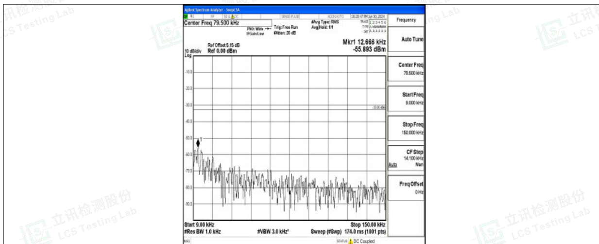
Band26_10MHz_QPSK_26740_1RB#0_0.009~0.15_0.009~0.15
