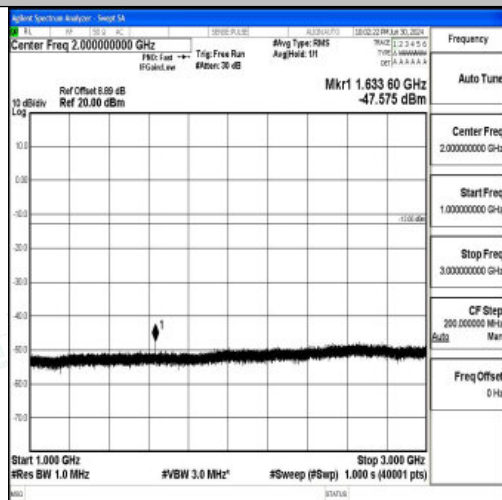
Band26_5MHz_QPSK_26740_1RB#0_1000~3000_1000~3000
