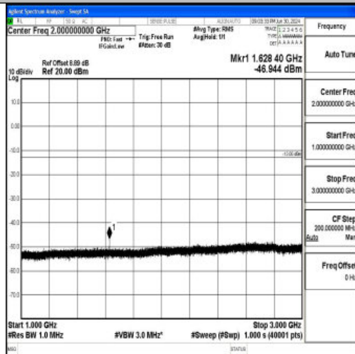
Band26_1.4MHz_16QAM_26697_1RB#0_1000~3000_1000~3000
