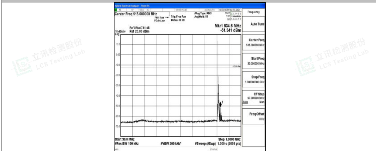
Band26_5MHz_QPSK_26715_1RB#0_30~1000_30~1000
