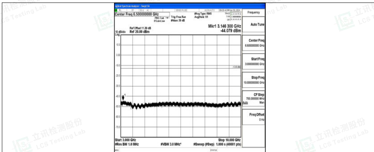
Band26_1.4MHz_16QAM_26697_1RB#0_3000~10000_3000~10000
