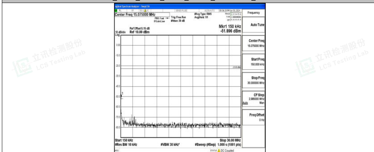
Band26_3MHz_QPSK_26740_1RB#0_0.15~30_0.15~30
