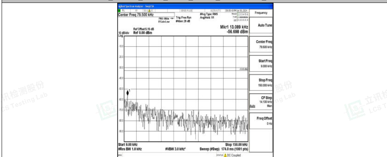
Band26_1.4MHz_16QAM_26783_1RB#0_0.009~0.15_0.009~0.15
