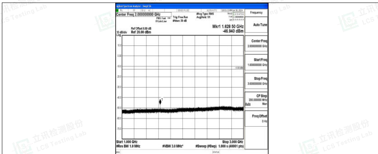
Band26_5MHz_QPSK_26715_1RB#0_1000~3000_1000~3000
