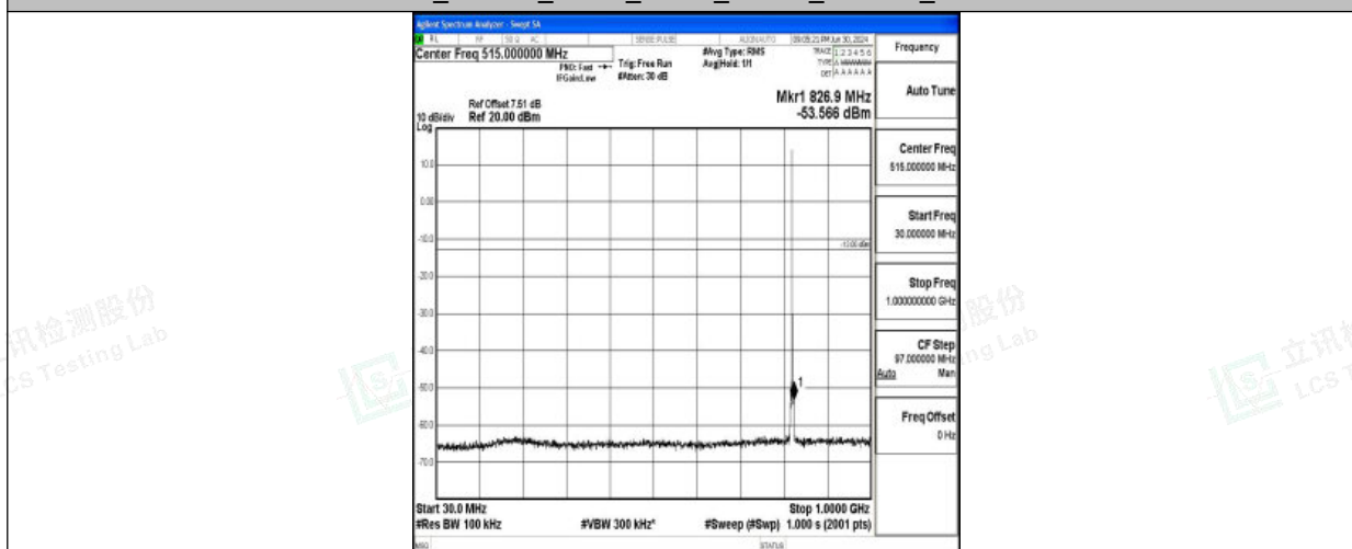
Band26_1.4MHz_QPSK_26783_1RB#0_30~1000_30~1000
