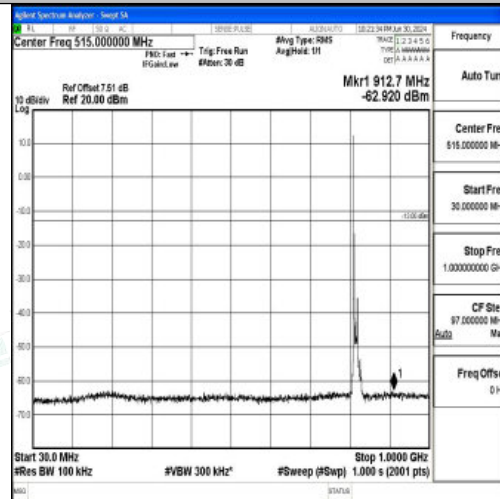
Band26_10MHz_16QAM_26740_1RB#0_30~1000_30~1000
