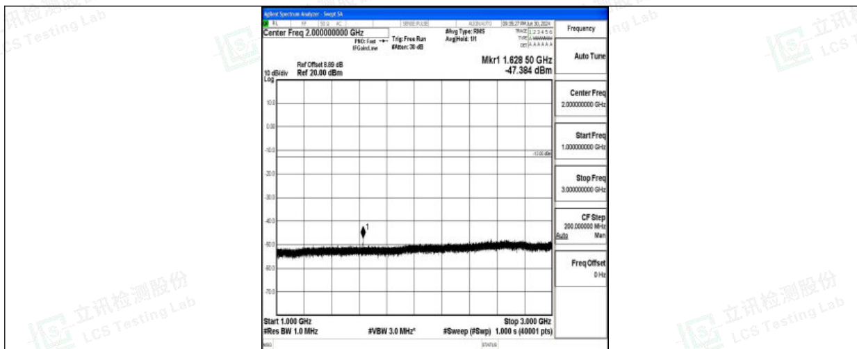
Band26_3MHz_QPSK_26705_1RB#0_1000~3000_1000~3000
