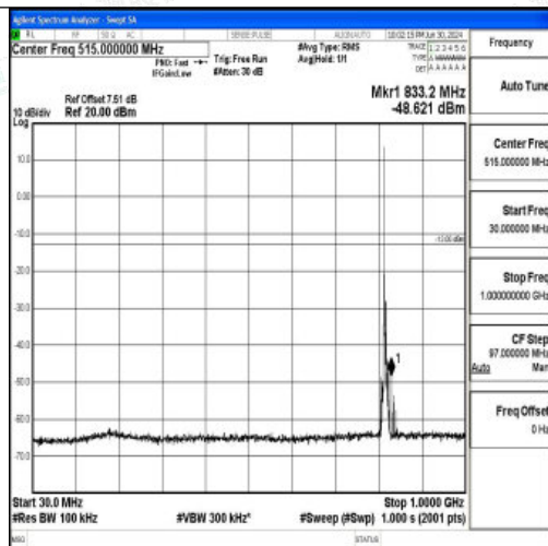
Band26_5MHz_QPSK_26740_1RB#0_30~1000_30~1000
