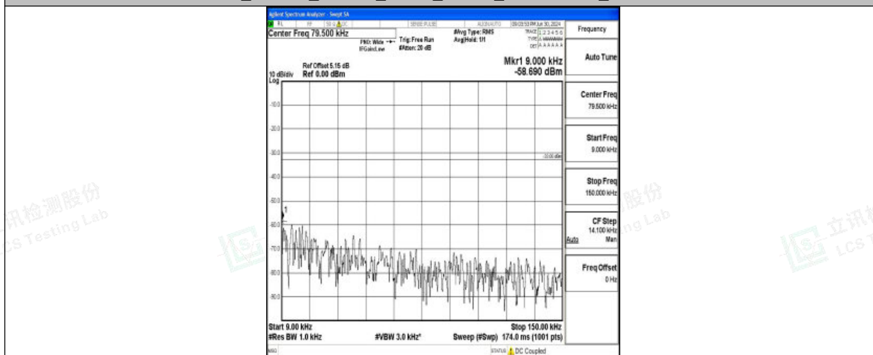
Band26_1.4MHz_QPSK_26740_1RB#0_0.009~0.15_0.009~0.15
