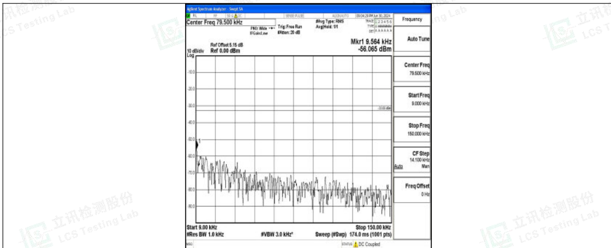
Band26_1.4MHz_16QAM_26740_1RB#0_0.009~0.15_0.009~0.15
