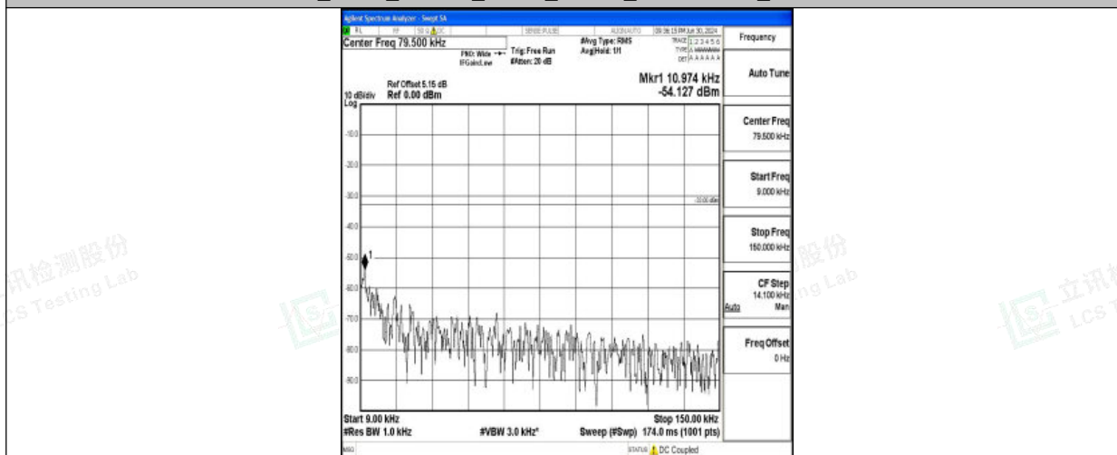
Band26_3MHz_QPSK_26740_1RB#0_0.009~0.15_0.009~0.15
