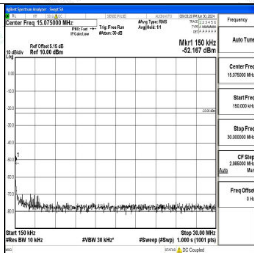
Band26_1.4MHz_16QAM_26697_1RB#0_0.15~30_0.15~30
