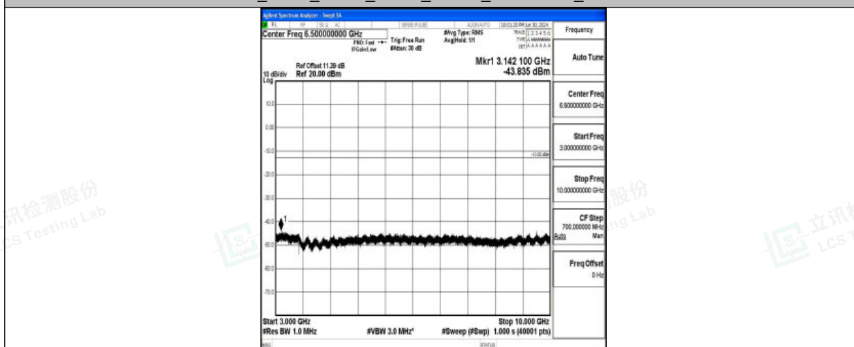
Band26_5MHz_QPSK_26715_1RB#0_3000~10000_3000~10000
