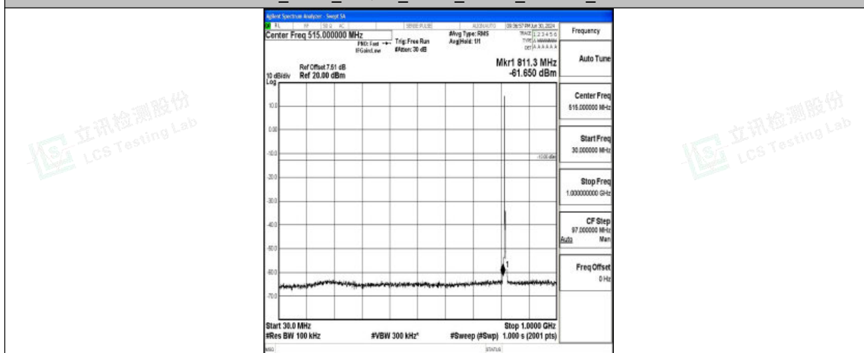
Band26_3MHz_16QAM_26740_1RB#0_30~1000_30~1000
