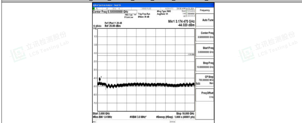
Band26_3MHz_16QAM_26775_1RB#0_3000~10000_3000~10000
