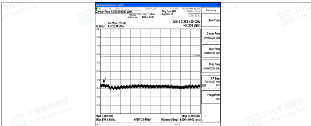
Band26_3MHz_QPSK_26775_1RB#0_3000~10000_3000~10000
