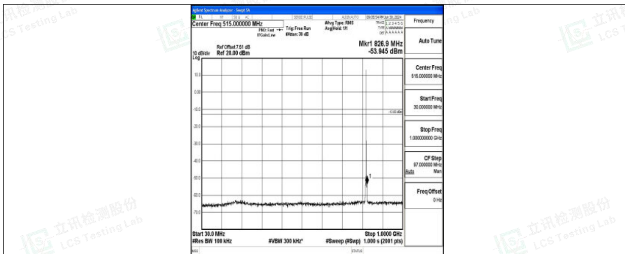
Band26_1.4MHz_16QAM_26783_1RB#0_30~1000_30~1000
