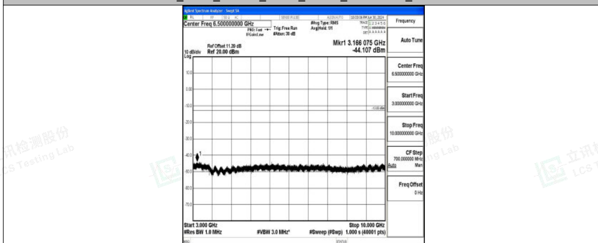
Band26_5MHz_16QAM_26740_1RB#0_3000~10000_3000~10000
