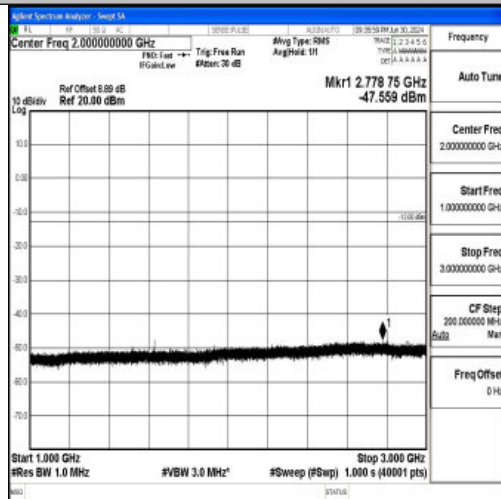
Band26_3MHz_16QAM_26705_1RB#0_1000~3000_1000~3000
