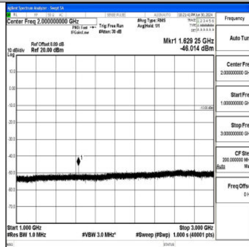
Band26_10MHz_16QAM_26740_1RB#0_1000~3000_1000~3000
