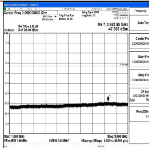
Band26_5MHz_16QAM_26715_1RB#0_1000~3000_1000~3000
