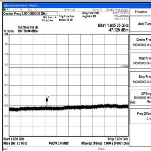
Band26_3MHz_QPSK_26740_1RB#0_1000~3000_1000~3000
