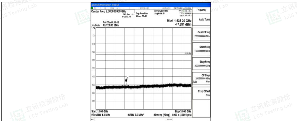
Band26_3MHz_16QAM_26740_1RB#0_1000~3000_1000~3000
