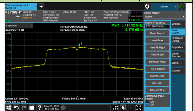
Channel 142 (5710MHz)
