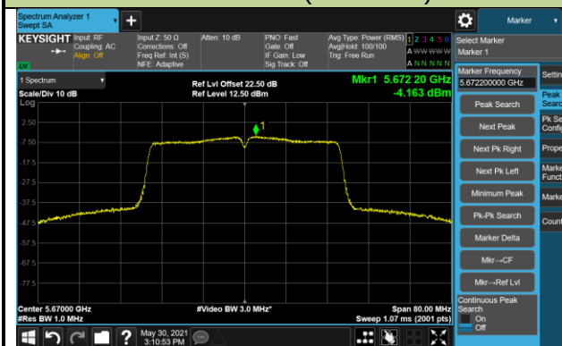
Channel 134 (5670MHz)
