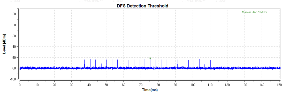
Radar Signal 4
