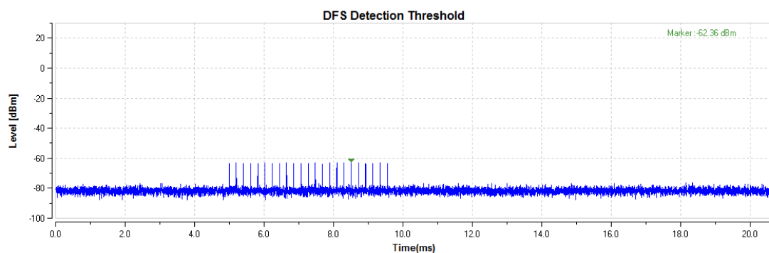
Radar Signal 2
