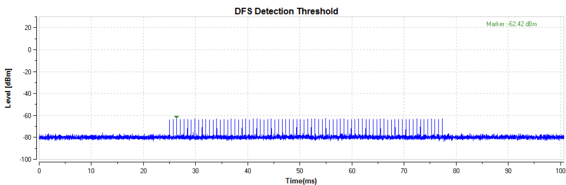
Radar Signal 1
