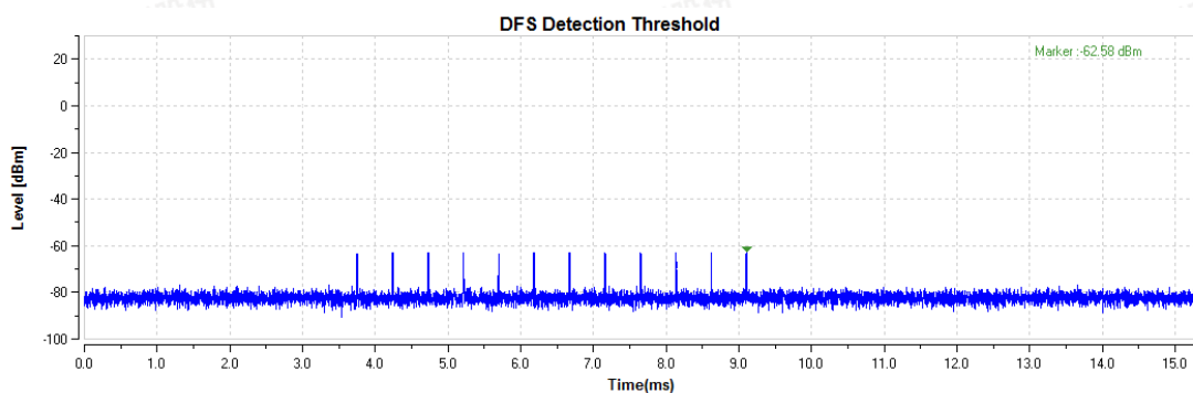
Radar Signal 4
