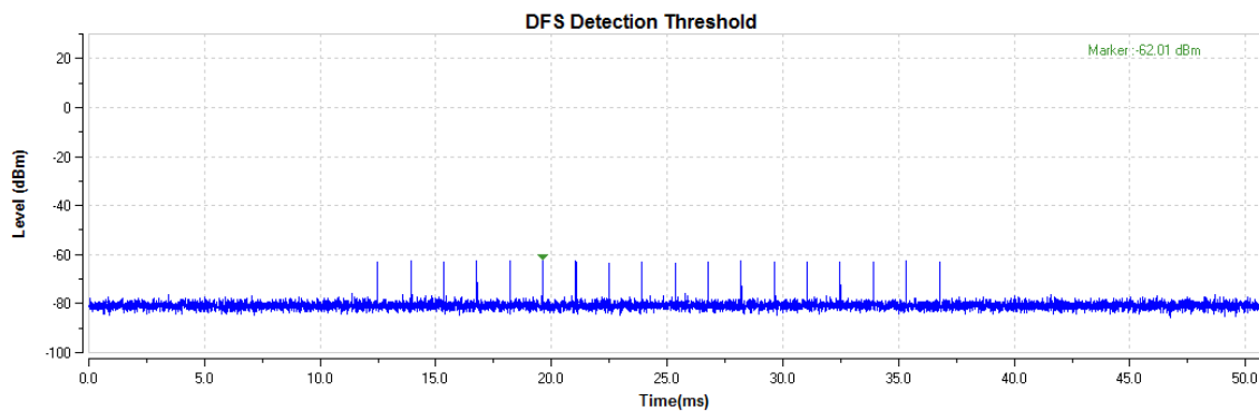
Radar Signal 0
