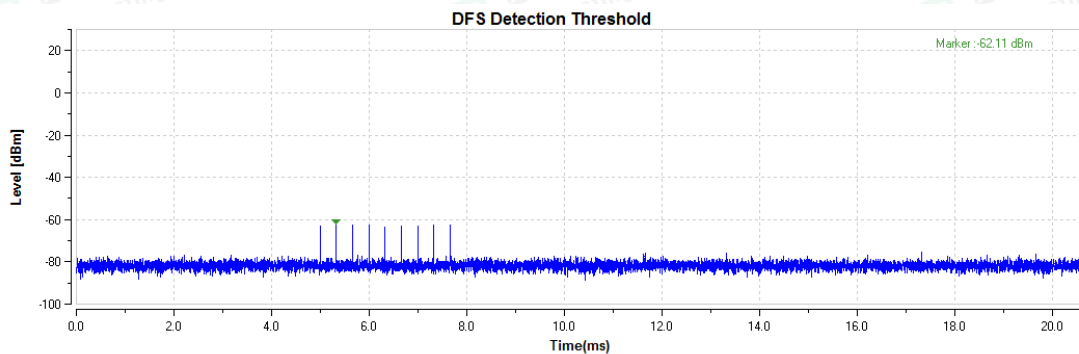
Radar Signal 6
