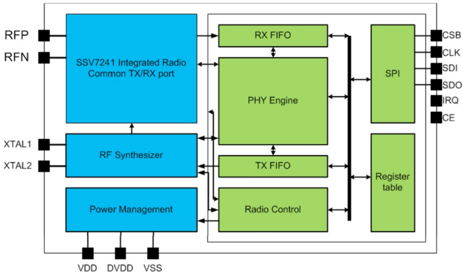
Figure 1: Block diagram of SSV7241
