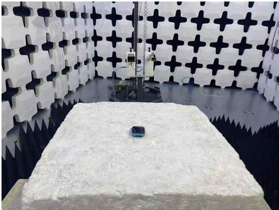
6. Radiated Emissions (Part 15C,18GHz -26.5GHz)
