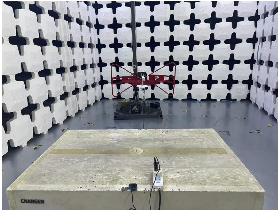
1. Radiated Emissions (Part 15B Camera, 30MHz-1GHz)
