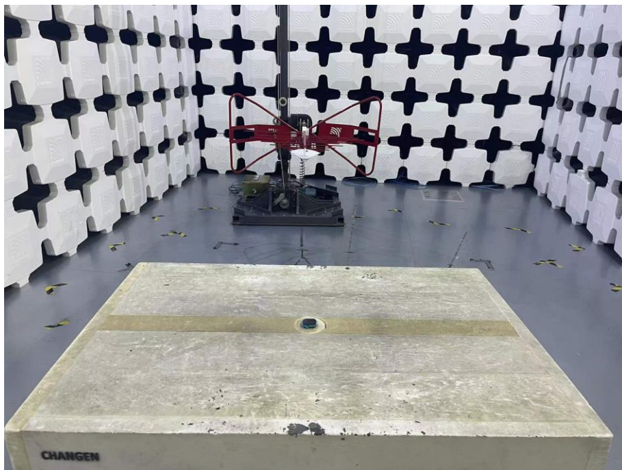
4. Radiated Emissions (Part 15C, 30MHz-1GHz)
