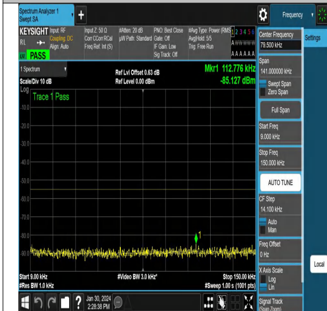
NTNV_N38_PC3_30_15_H_TID1_NS_01_0.009_0.15_#1
