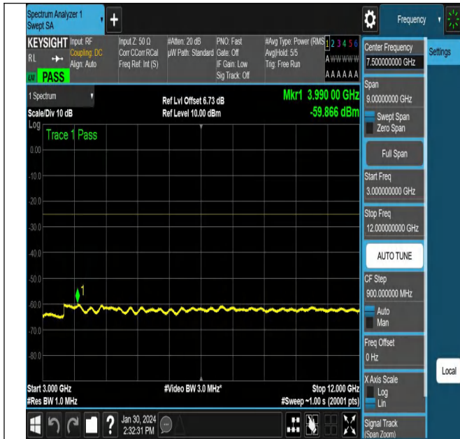
NTNV_N38_PC3_30_15_H_TID4_NS_01_3000_12000_#1
