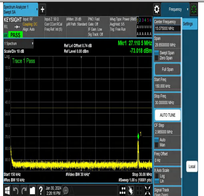
NTNV_N38_PC3_30_15_M_TID5_NS_01_0.15_30_#1
