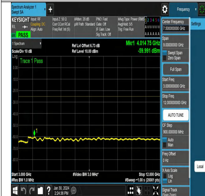
NTNV_N38_PC3_30_15_M_TID3_NS_01_3000_12000_#1
