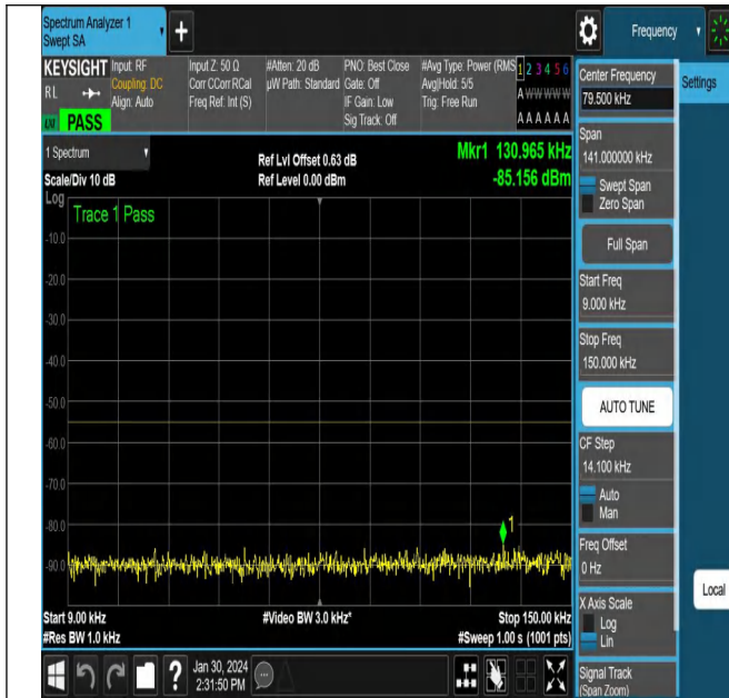
NTNV_N38_PC3_30_15_H_TID4_NS_01_0.009_0.15_#1
