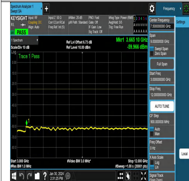
NTNV_N38_PC3_30_15_H_TID3_NS_01_3000_12000_#1
