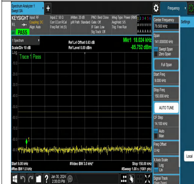
NTNV_N38_PC3_30_15_H_TID7_NS_01_0.009_0.15_#1
