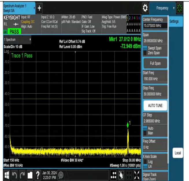
NTNV_N38_PC3_30_15_M_TID2_NS_01_0.15_30_#1
