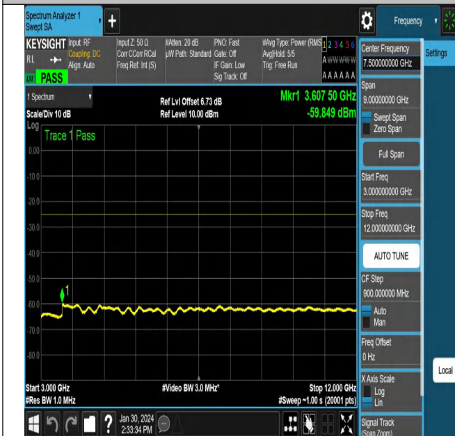
NTNV_N38_PC3_30_15_H_TID5_NS_01_3000_12000_#1
