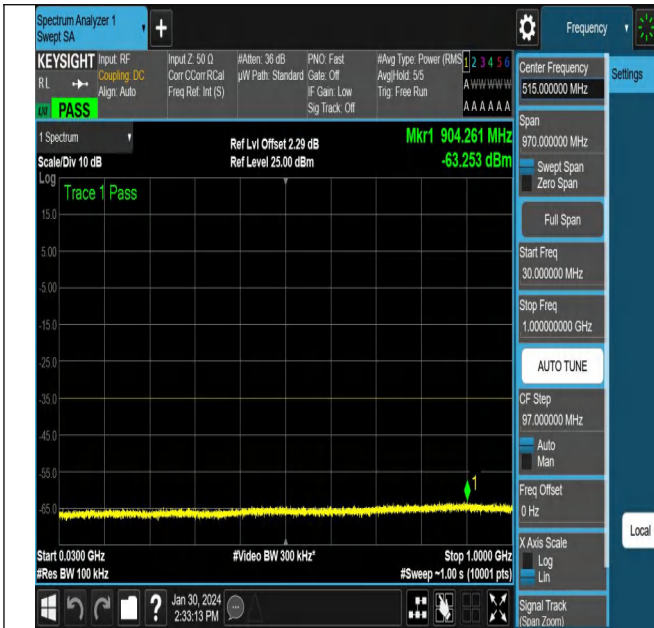
NTNV_N38_PC3_30_15_H_TID5_NS_01_30_1000_#1
