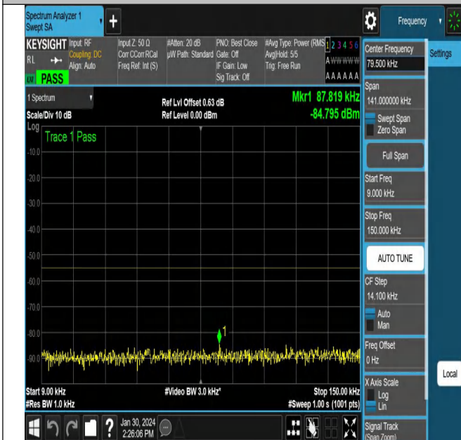
NTNV_N38_PC3_30_15_M_TID5_NS_01_0.009_0.15_#1
