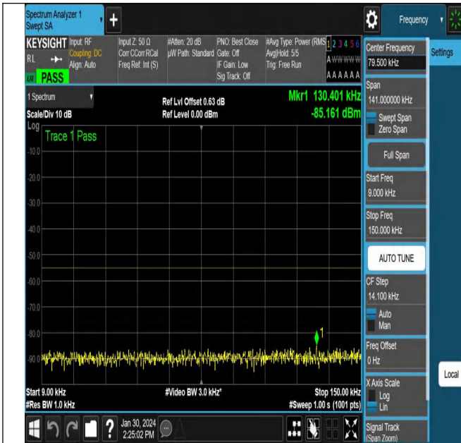
NTNV_N38_PC3_30_15_M_TID4_NS_01_0.009_0.15_#1
