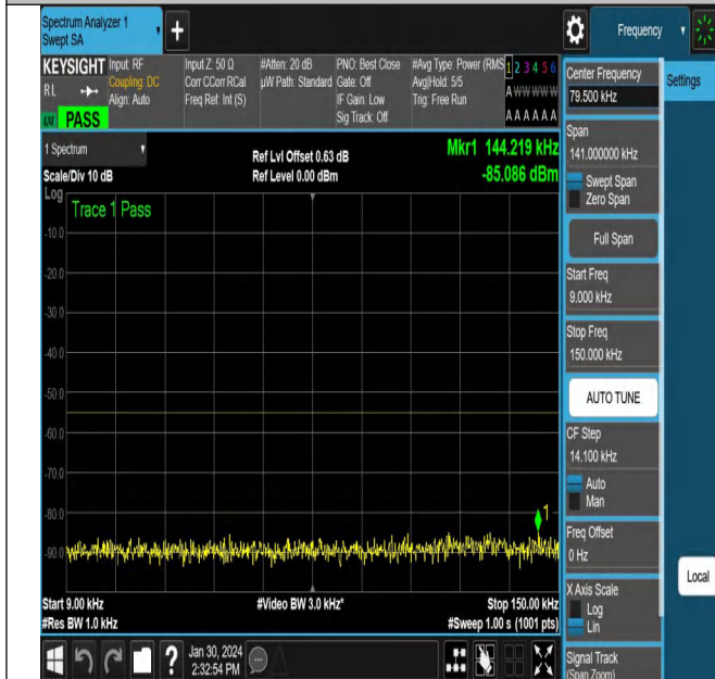
NTNV_N38_PC3_30_15_H_TID5_NS_01_0.009_0.15_#1
