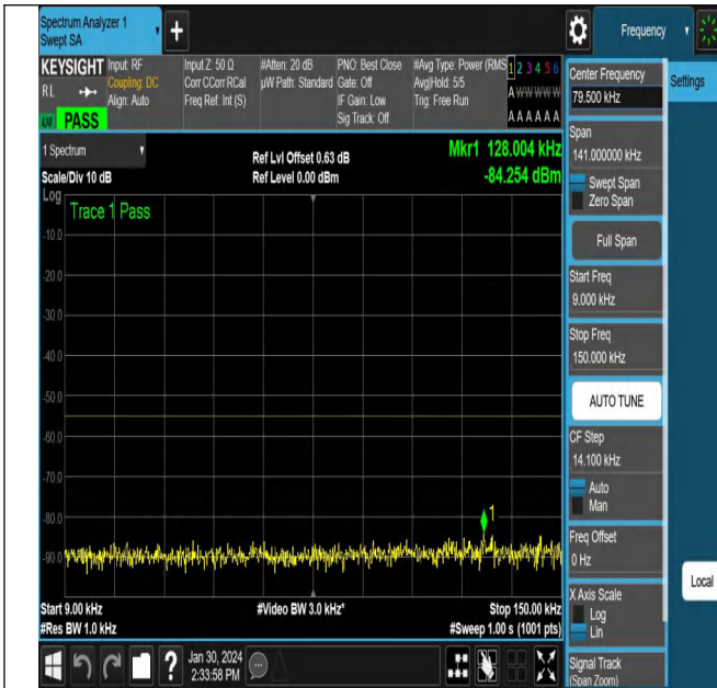
NTNV_N38_PC3_30_15_H_TID6_NS_01_0.009_0.15_#1
