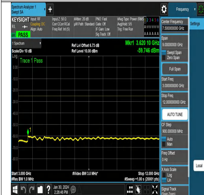
NTNV_N38_PC3_30_15_M_TID5_NS_01_3000_12000_#1
