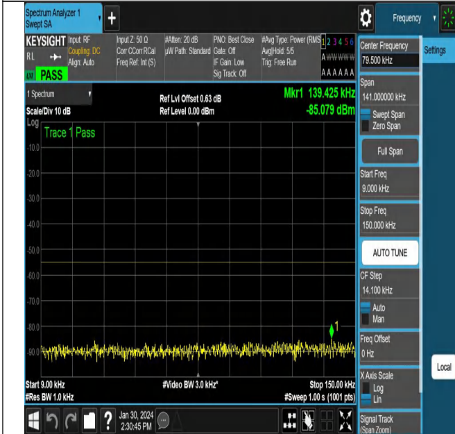
NTNV_N38_PC3_30_15_H_TID3_NS_01_0.009_0.15_#1
