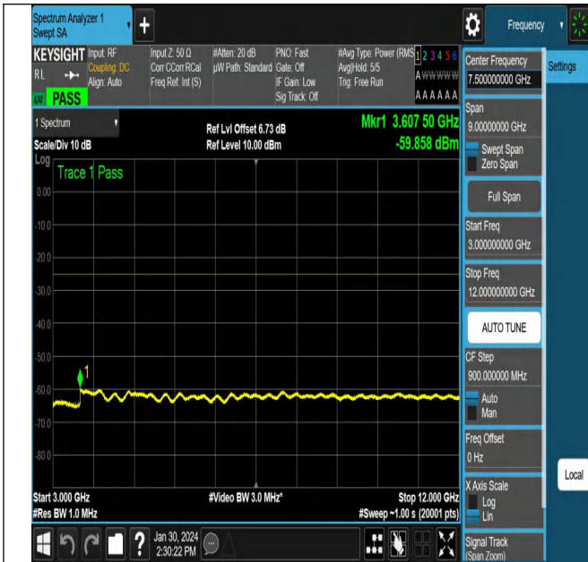
NTNV_N38_PC3_30_15_H_TID2_NS_01_3000_12000_#1
