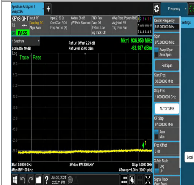
NTNV_N38_PC3_30_15_M_TID2_NS_01_30_1000_#1
