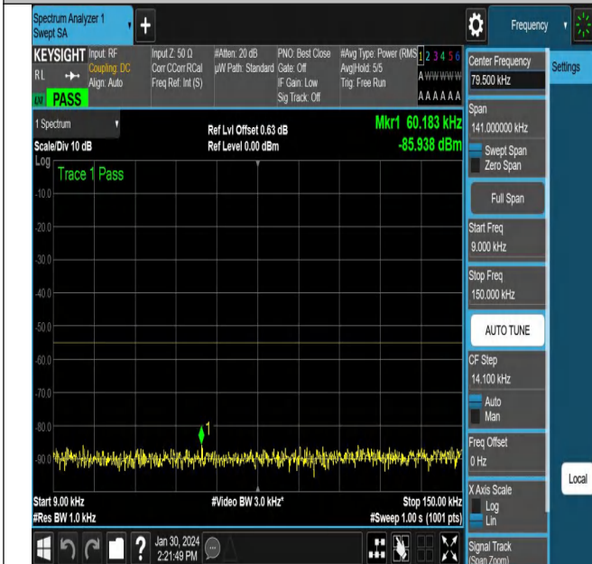
NTNV_N38_PC3_30_15_M_TID1_NS_01_0.009_0.15_#1
