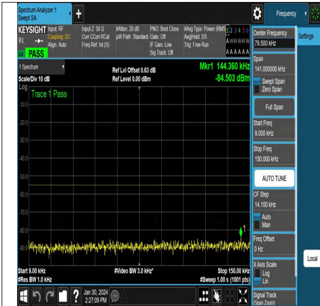
NTNV_N38_PC3_30_15_M_TID6_NS_01_0.009_0.15_#1
