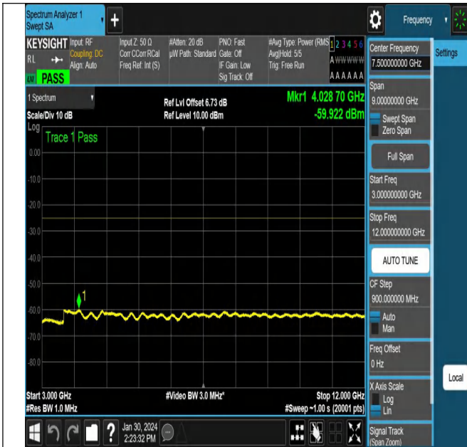
NTNV_N38_PC3_30_15_M_TID2_NS_01_3000_12000_#1
