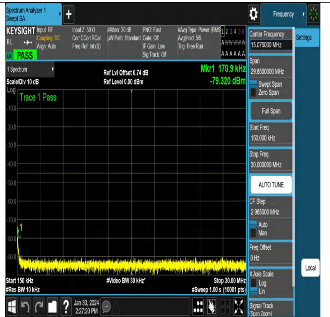
NTNV_N38_PC3_30_15_M_TID6_NS_01_0.15_30_#1
