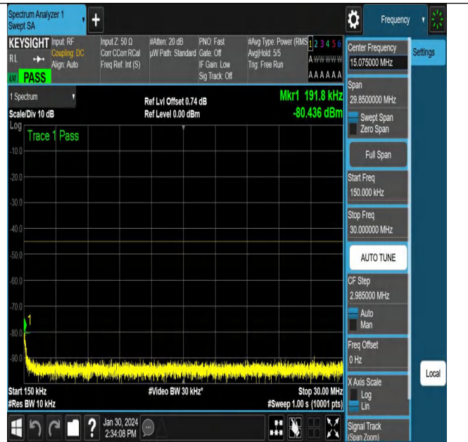
NTNV_N38_PC3_30_15_H_TID6_NS_01_0.15_30_#1
