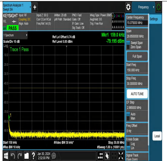
NTNV_N38_PC3_30_15_H_TID4_NS_01_0.15_30_#1
