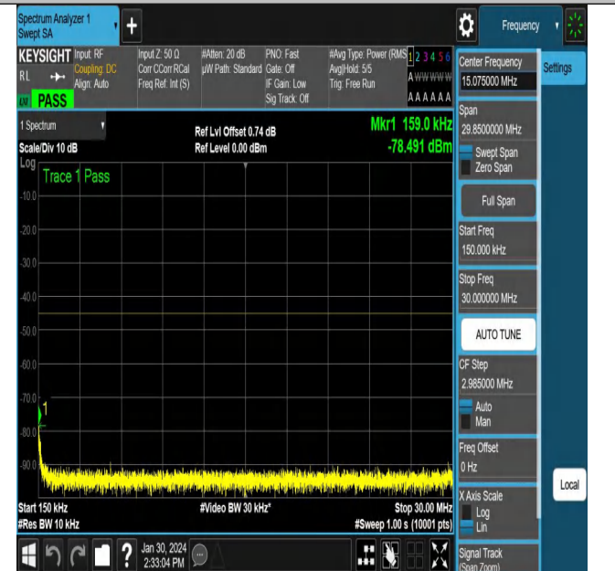
NTNV_N38_PC3_30_15_H_TID5_NS_01_0.15_30_#1
