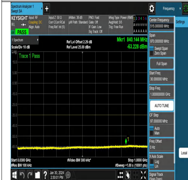
NTNV_N38_PC3_30_15_H_TID2_NS_01_30_1000_#1
