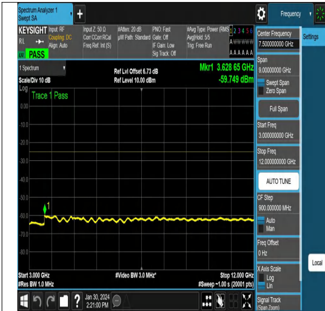
NTNV_N38_PC3_30_15_L_TID6_NS_01_3000_12000_#1
