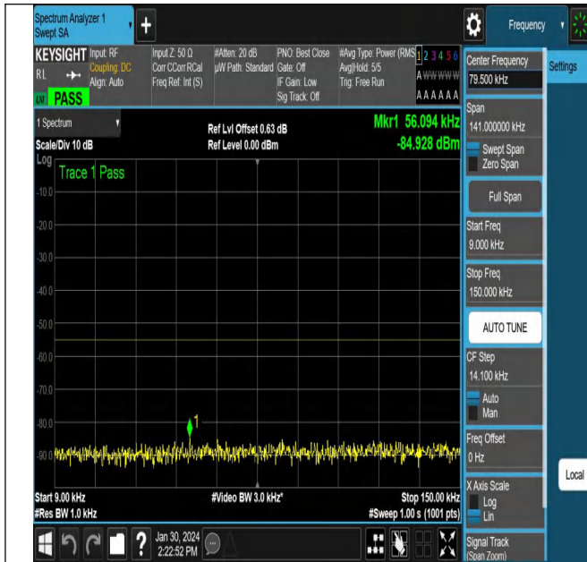
NTNV_N38_PC3_30_15_M_TID2_NS_01_0.009_0.15_#1
