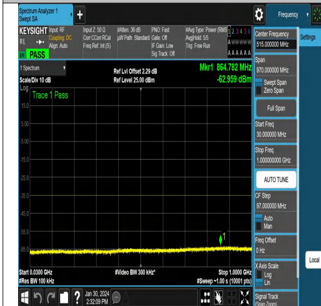
NTNV_N38_PC3_30_15_H_TID4_NS_01_30_1000_#1
