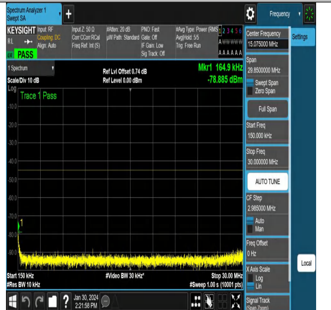
NTNV_N38_PC3_30_15_M_TID1_NS_01_0.15_30_#1
