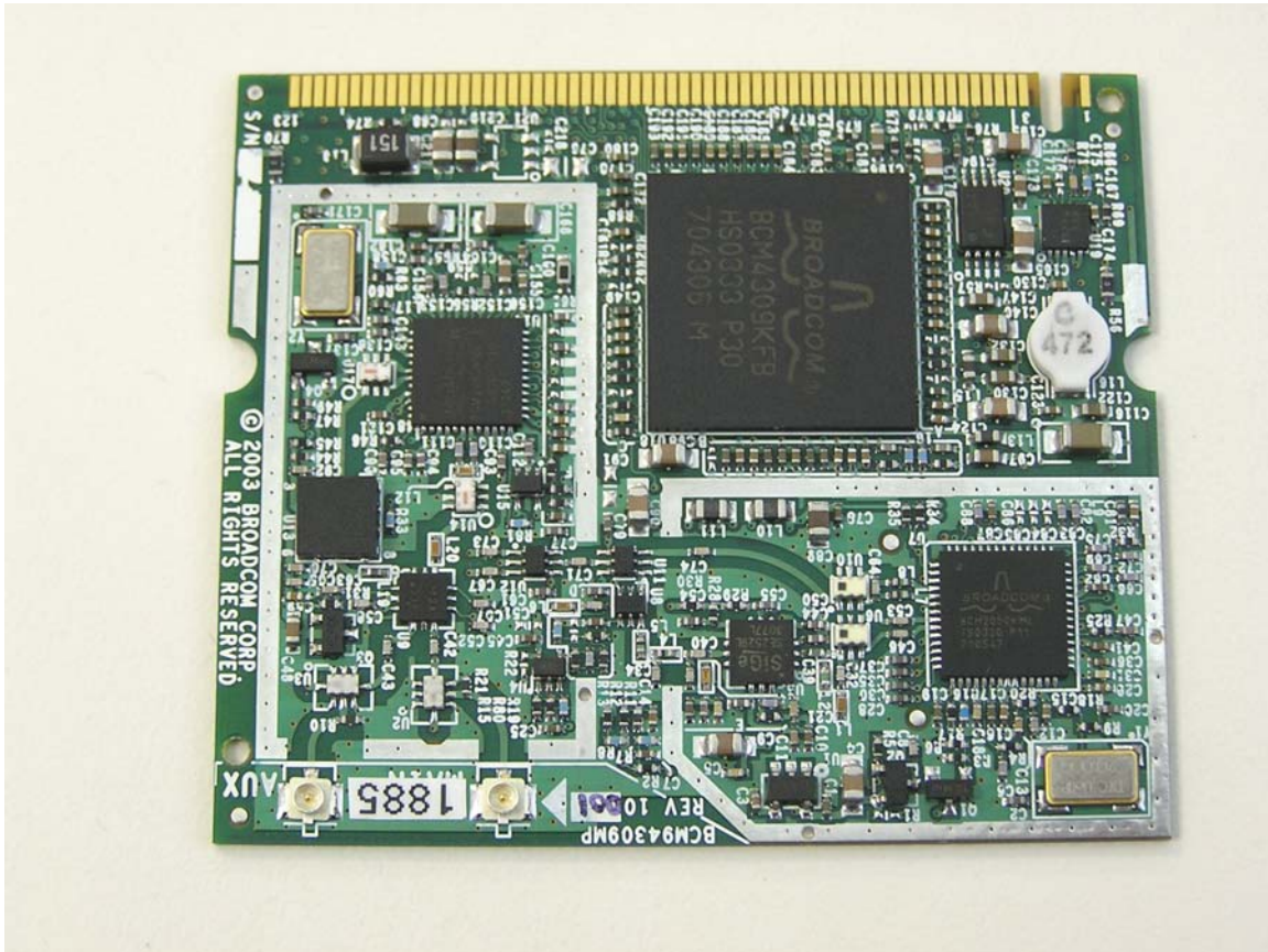
WLAN Model# BCM94309MP Top view - unshielded
