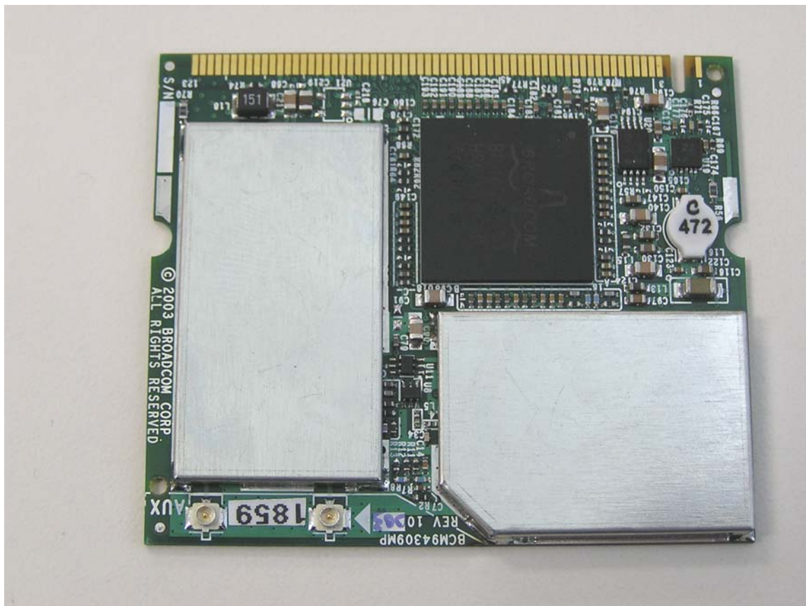
WLAN Model# BCM94309MP Top view - shielded
