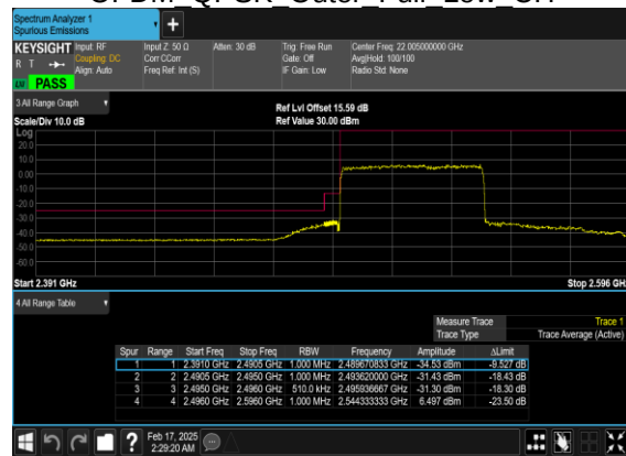
N41(50M)_DFT-s-OFDM_QPSK_Outer_Full_Low_CH
