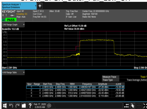
N41(50M)_DFT-s-OFDM_BPSK_Outer_Full_Low_CH
