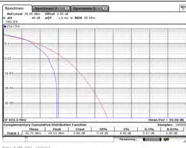
CH26783_1.4M_16-QAM_1RB5
