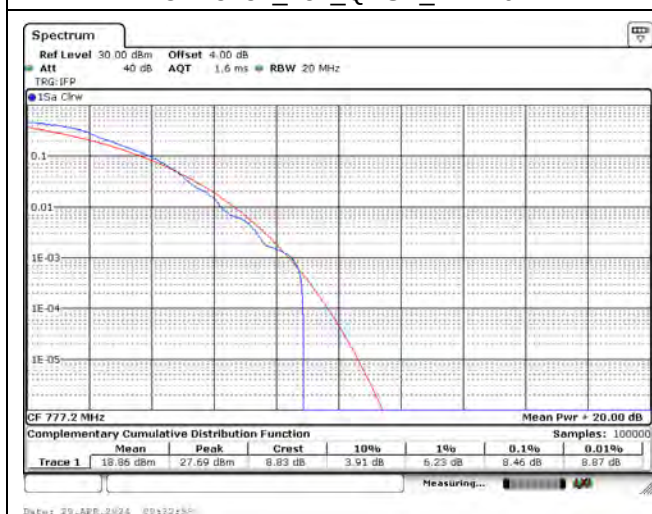
CH23182_15k_QPSK_12RB0
