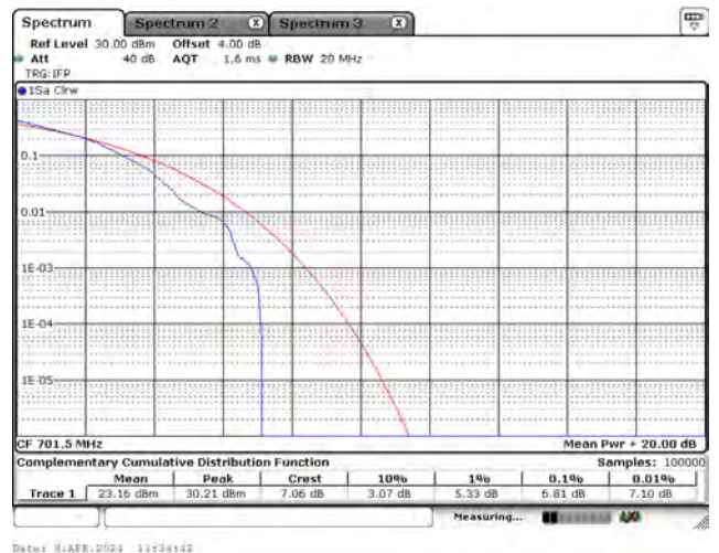
CH23155_5M_16-QAM_1RB5
