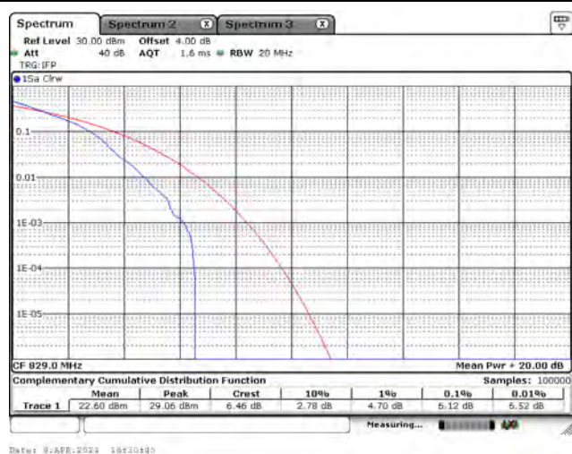
CH26840_10M_QPSK_1RB0
