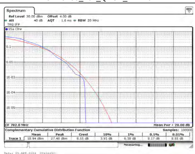
CH23230_15k_QPSK_12RB0
