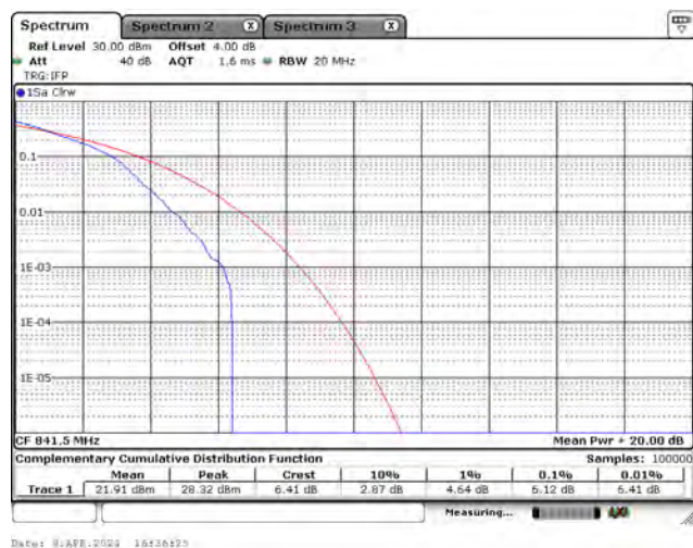
CH26965_15M_QPSK_1RB5
