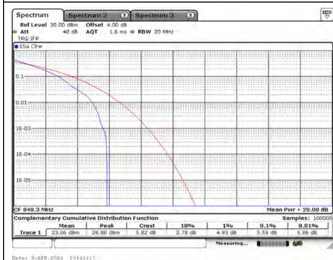
CH27033_1.4M_QPSK_1RB5
