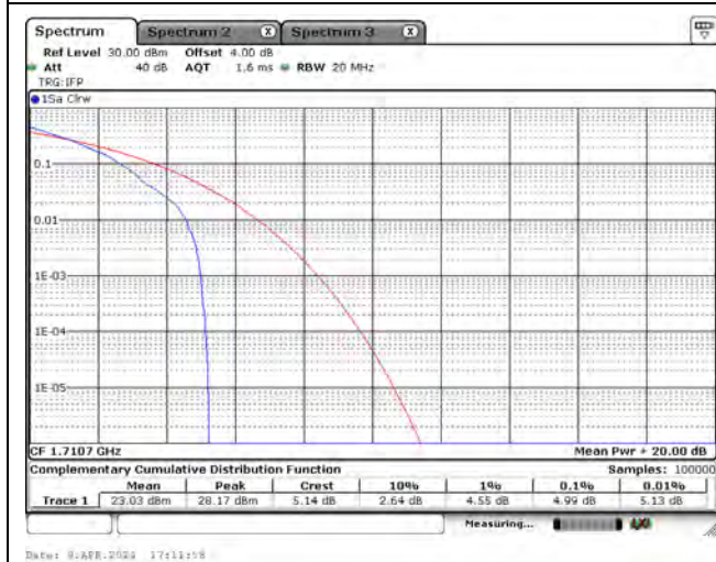
CH131979_1.4M_QPSK_1RB0
