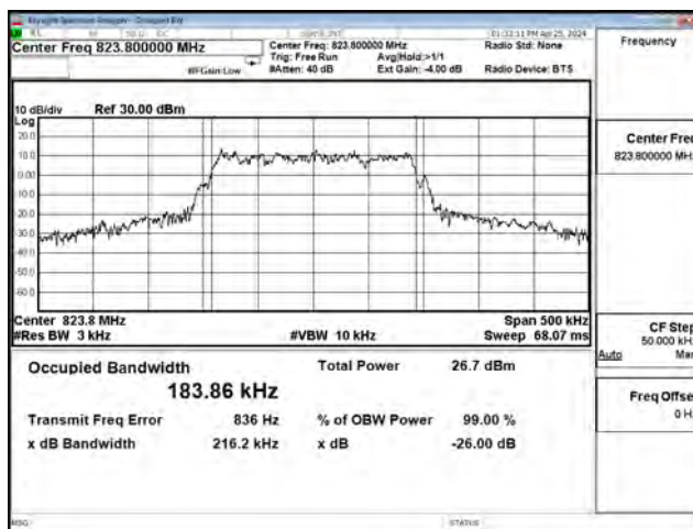
QPSK_CH26788_15k_12RB0
