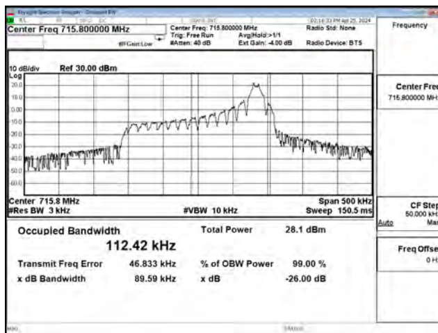
QPSK_CH134092_15k_1RB0
