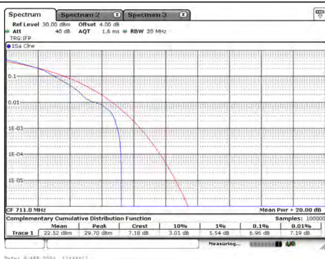
CH23130_10M_16-QAM_1RB5
