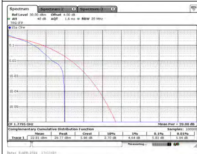
CH132665_1.4M_QPSK_1RB5
