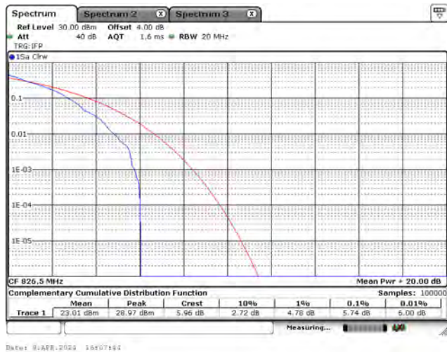
CH26815_5M_QPSK_1RB0
