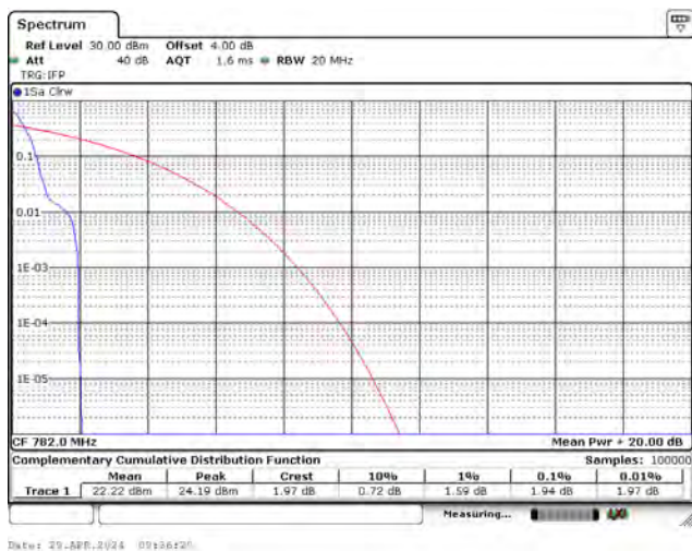
CH23230_15k_QPSK_1RB0
