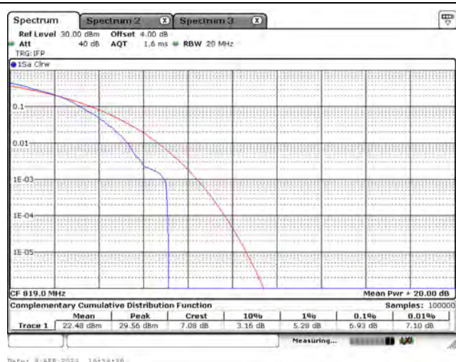
CH26740_1.4M_16-QAM_1RB0
