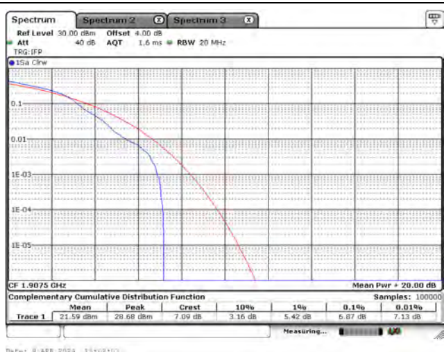
CH26615_15M_16-QAM_1RB5
