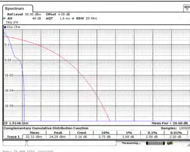
CH26688_15k_QPSK_1RB11
