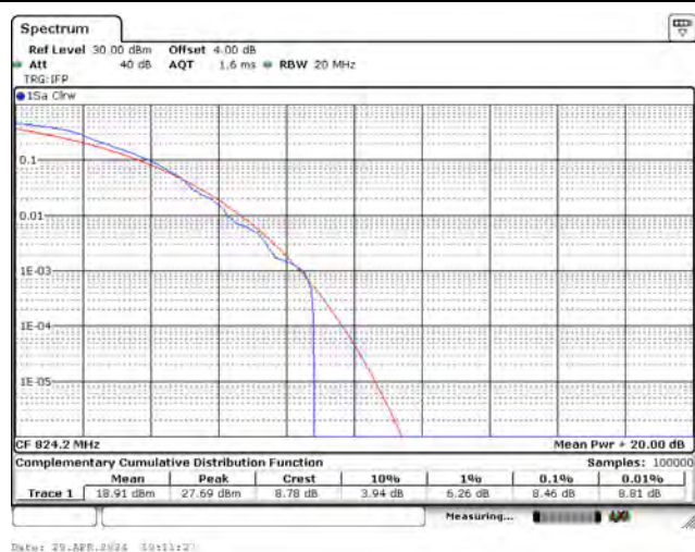
CH27038_15k_QPSK_12RB0
