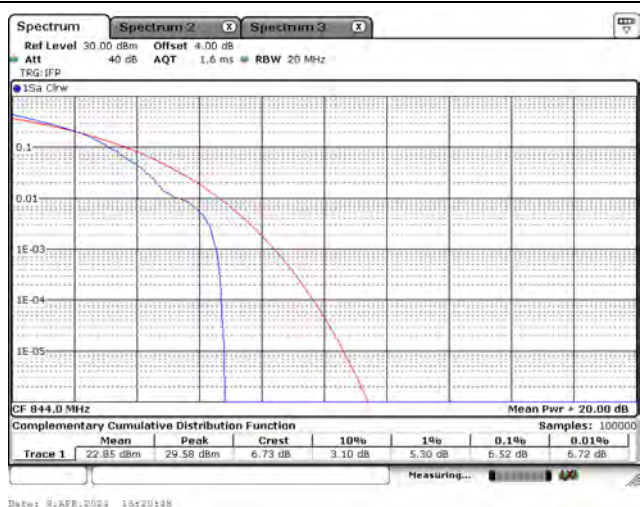
CH26990_10M_16-QAM_1RB5
