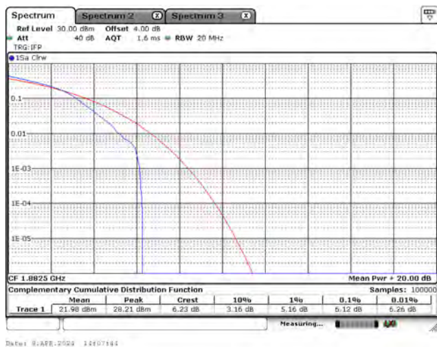
CH26365_3M_16-QAM_1RB0
