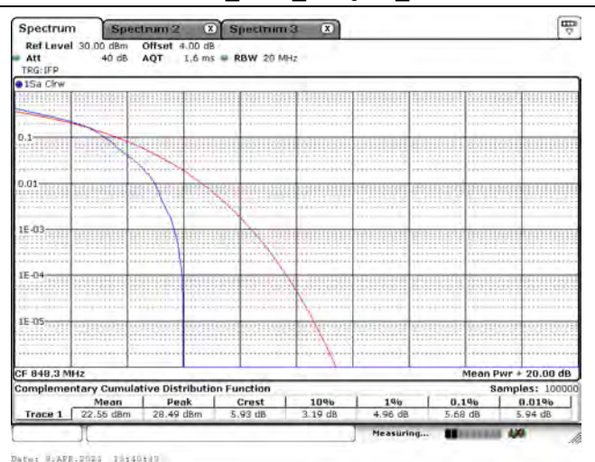
CH27033_1.4M_16-QAM_1RB5
