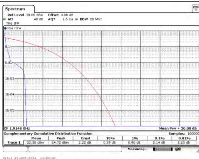
CH26688_3.75k_QPSK_1RB47
