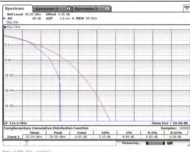
CH23165_16-QAM_1RB5
