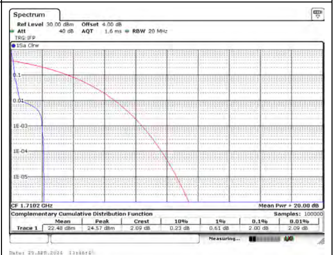
CH131974_3.75k_QPSK_1RB0
