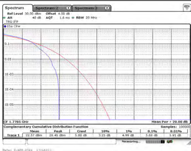
CH132657_3M_16-QAM_1RB5
