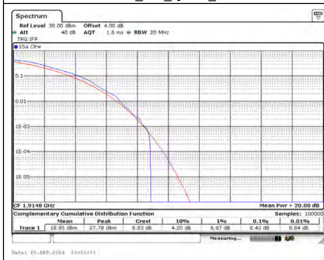
CH26688_15k_QPSK_12RB0
