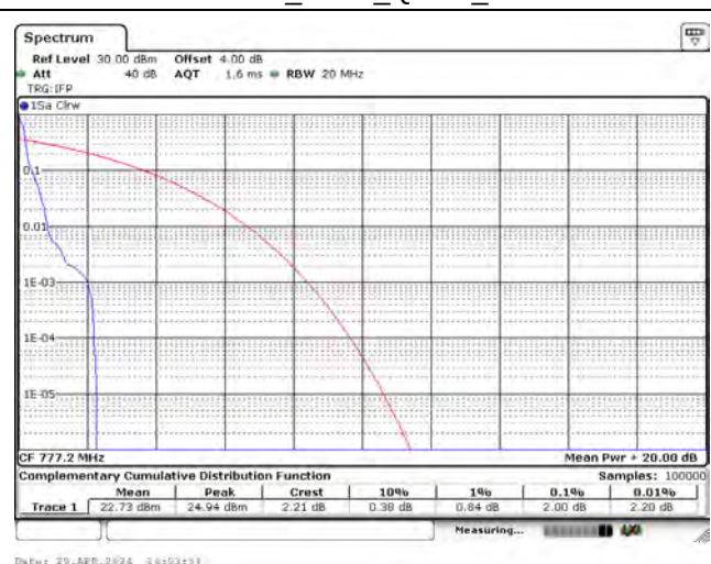
CH23182_3.75k_QPSK_1RB0
