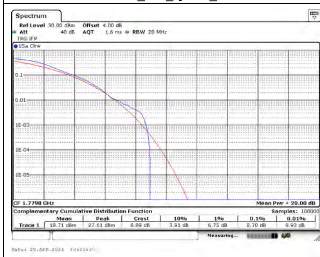
CH132670_15k_QPSK_12RB0
