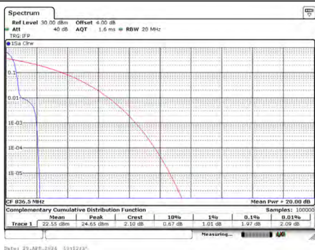
CH26915_15k_QPSK_1RB0
