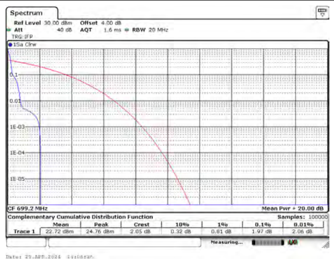
CH23012_3.75k_QPSK_1RB0
