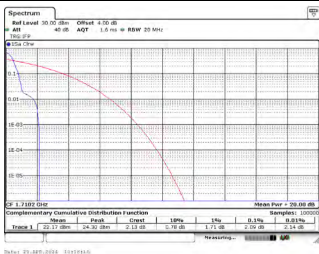
CH131974_15k_BPSK_1RB0
