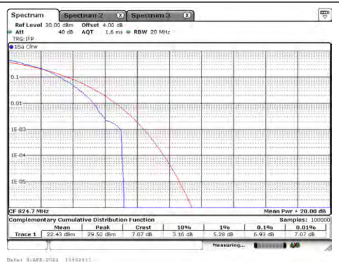
CH26797_1.4MN_16-QAM_1RB0
