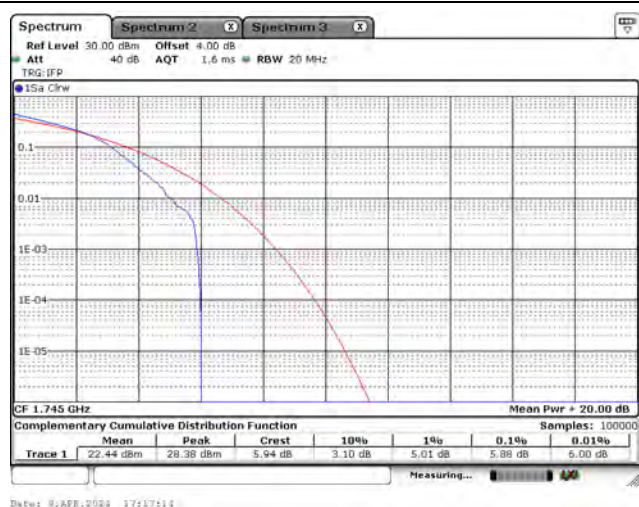
CH132322_3M_16-QAM_1RB0
