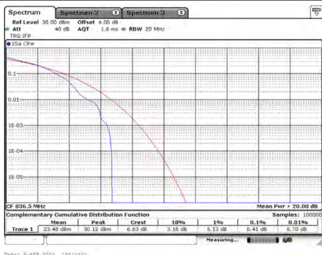
CH26915_5M_16-QAM_1RB0
