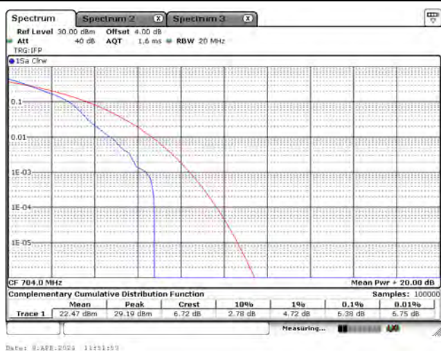
CH23060_10M_QPSK_1RB0
