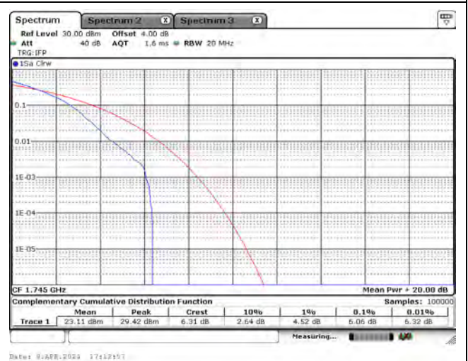
CH132322_1.4M_QPSK_1RB0
