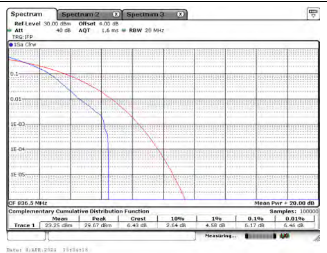
CH26915_1.4M_QPSK_1RB0
