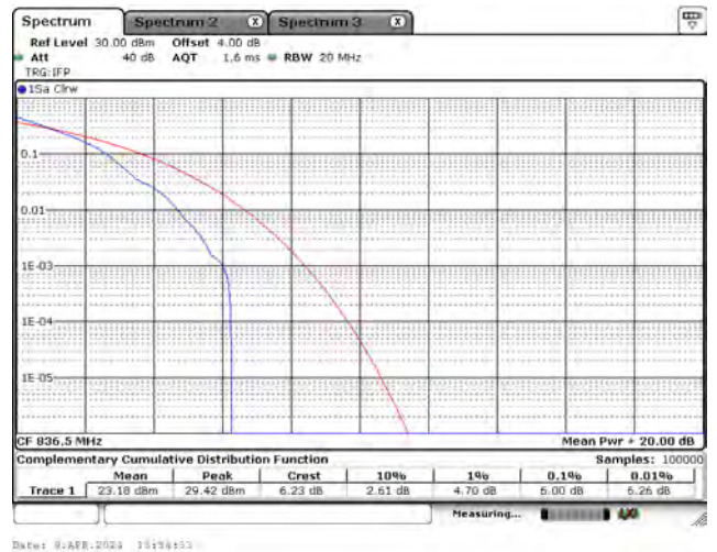
CH26915_3M_QPSK_1RB0
