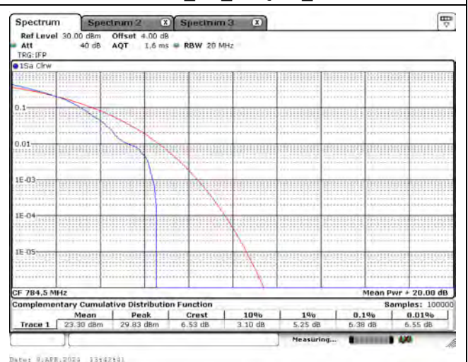
CH23255_5M_16-QAM_1RB5
