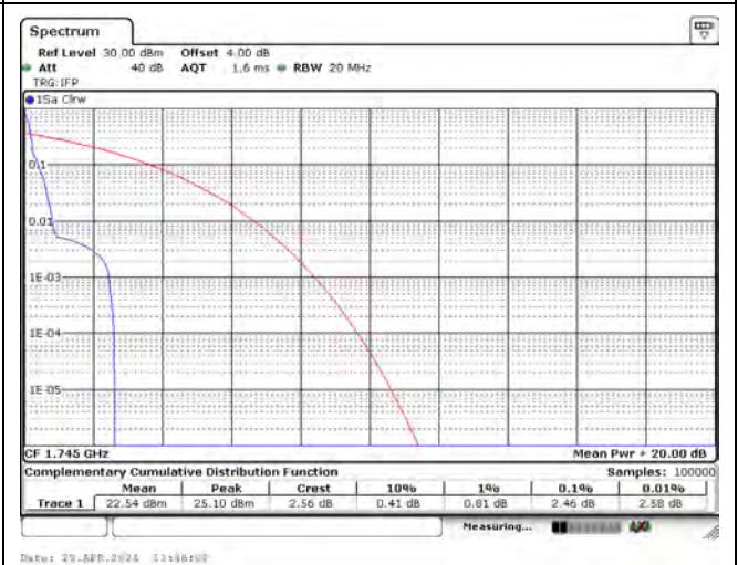
CH132322_3.75k_BPSK_1RB0
