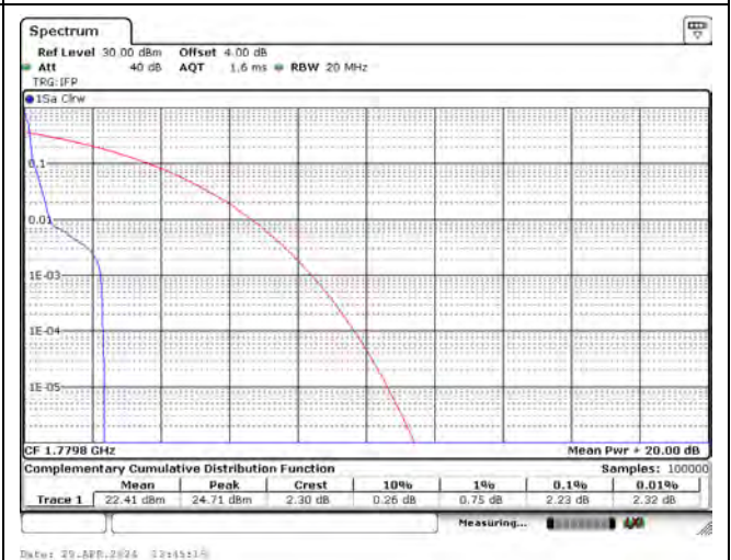
CH132670_3.75k_QPSK_1RB47
