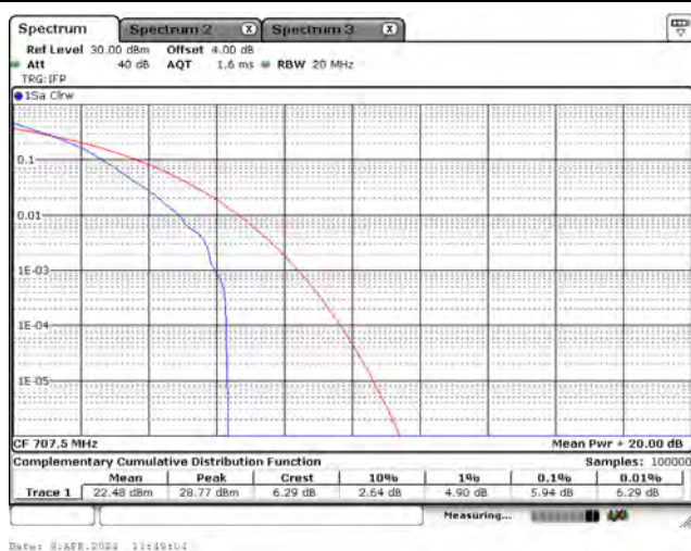
CH23095_10M_QPSK_1RB0
