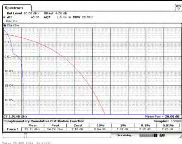
CH26365_15k_QPSK_1RB0
