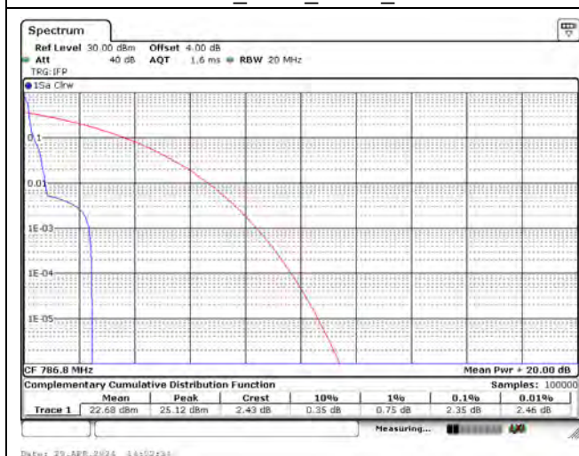
CH23278_3.75k_BPSK_1RB47
