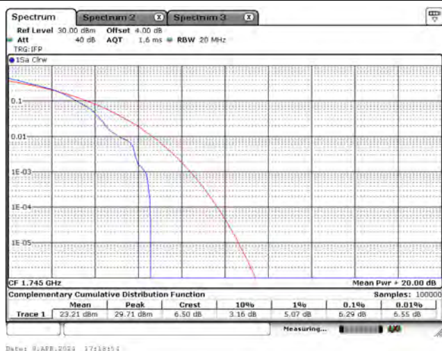
CH132322_5M_16-QAM_1RB0
