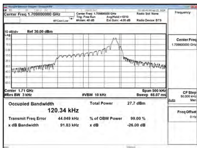
QPSK_CH133047_15k_1RB0
