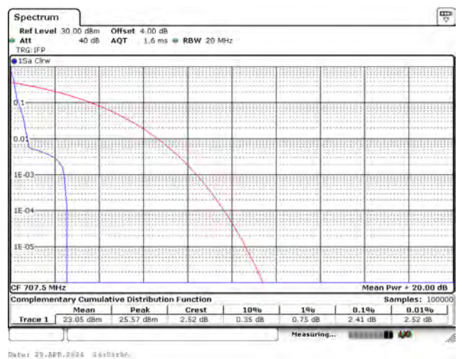
CH23095_3.75k_BPSK_1RB0
