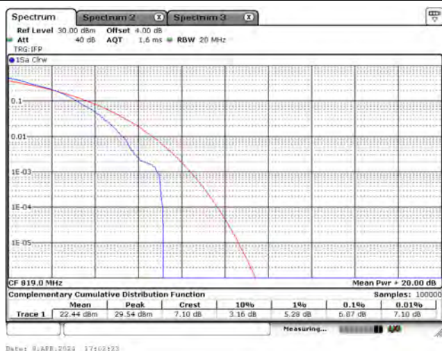
CH26740_3M_16-QAM_1RB0
