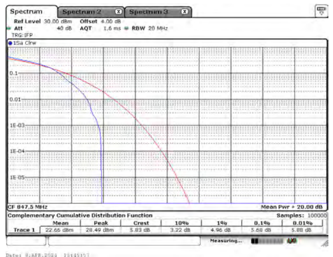
CH27025_3M_16-QAM_1RB5
