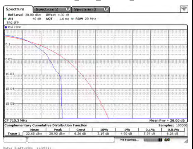
CH23173_1.4M_16-QAM_RB5
