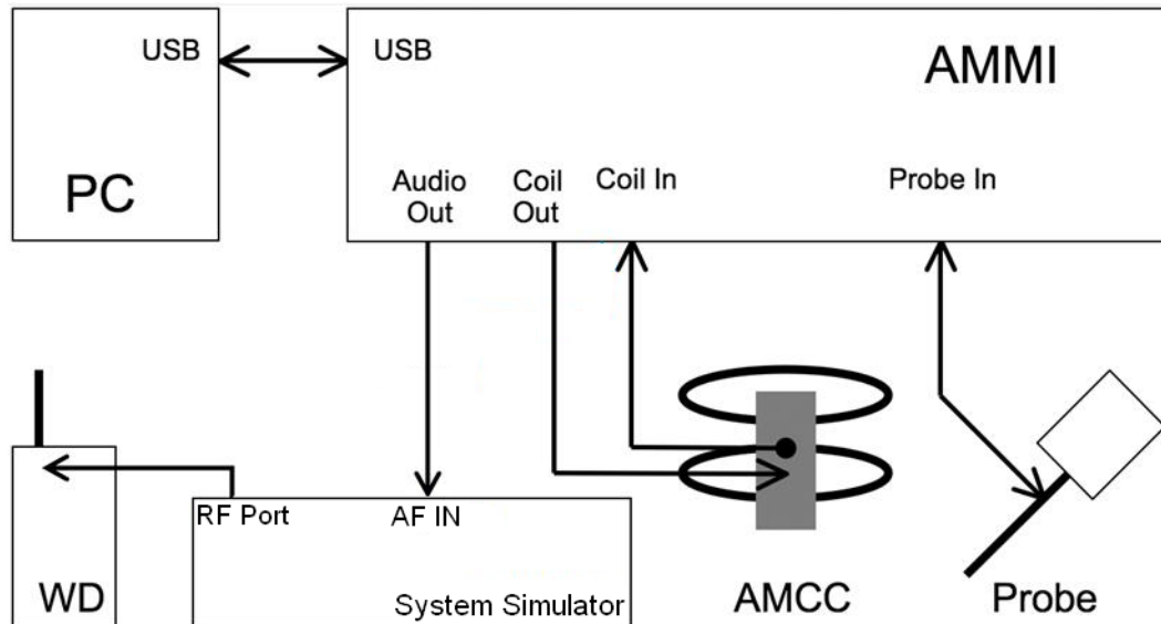
Fig-3.2 T-Coil Setup Cabling
