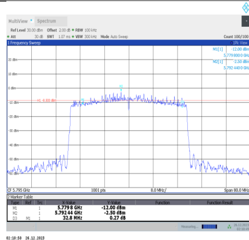
11ax40MIMO-Ant2-5795-PASS
