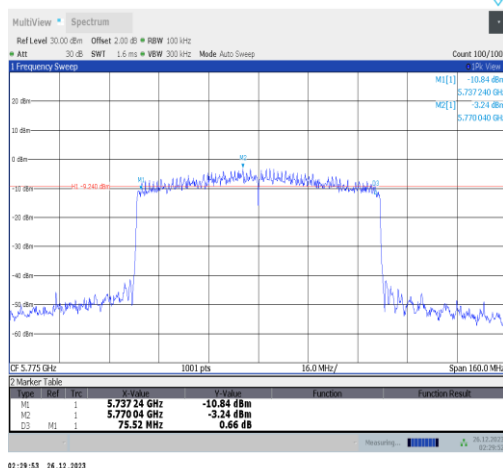
11ax80MIMO-Ant1-5775-PASS
