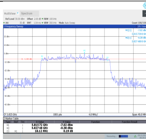
11ax20MIMO-Ant2-5825-PASS
