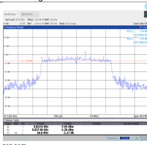
11ax20MIMO-Ant4-5825-PASS
