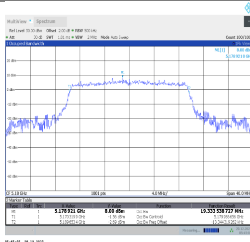
11ax20MIMO-Ant4-5180
