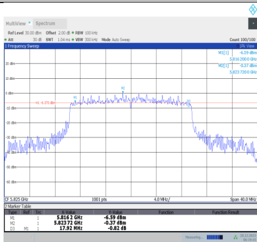
11ax20MIMO-Ant1-5825-PASS
