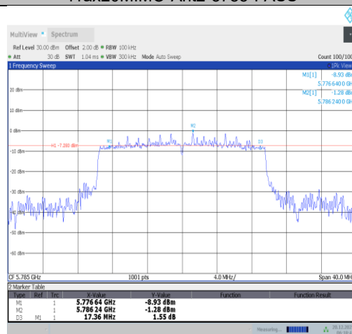
11ax20MIMO-Ant4-5785-PASS
