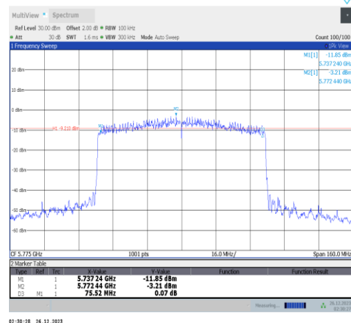
11ax80MIMO-Ant2-5775-PASS
