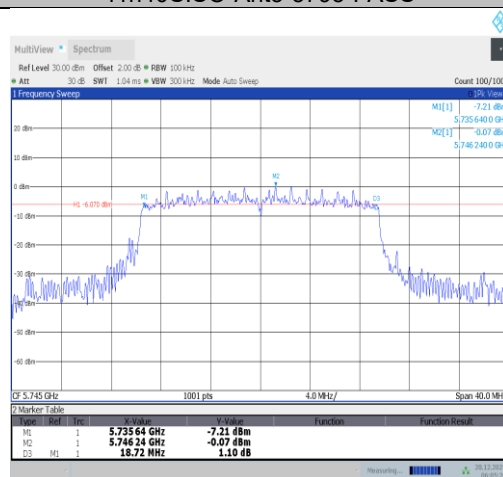
11ax20MIMO-Ant2-5745-PASS
