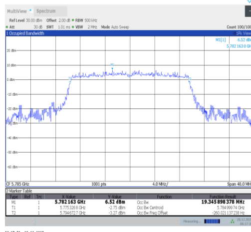
11ax20MIMO-Ant2-5785
