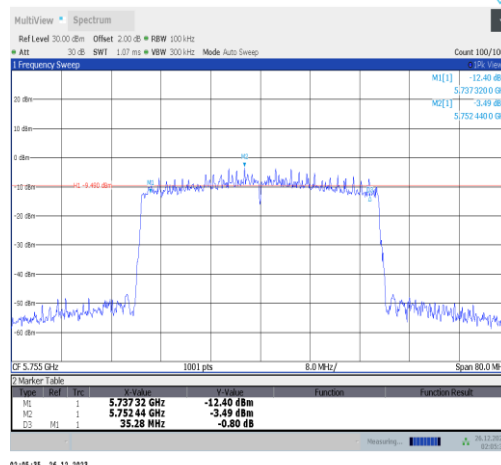
11ax40MIMO-Ant2-5755-PASS
