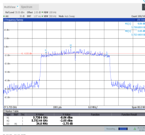
11ax40MIMO-Ant4-5755-PASS
