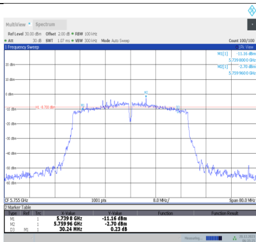
11n40SISO-Ant3-5755-PASS
