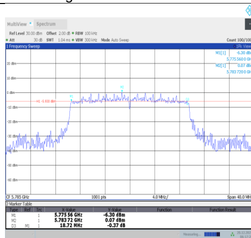
11ax20MIMO-Ant2-5785-PASS
