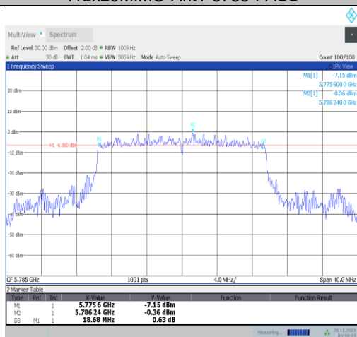
11ax20MIMO-Ant3-5785-PASS
