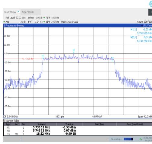
11ax20MIMO-Ant4-5745-PASS
