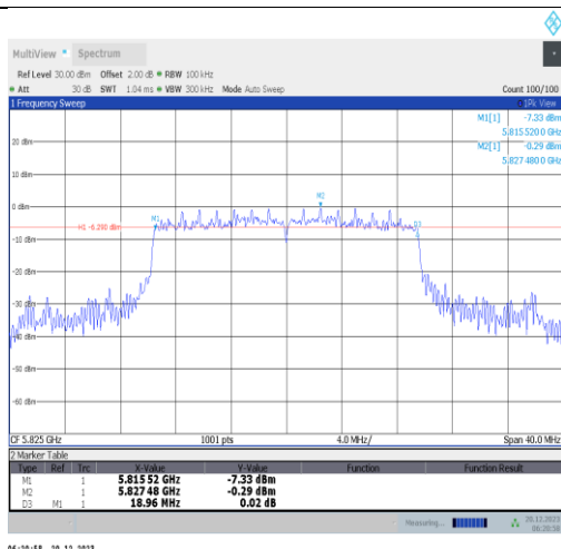
11ax20MIMO-Ant3-5825-PASS
