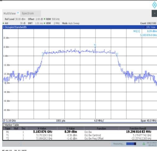
11ax20MIMO-Ant3-5180
