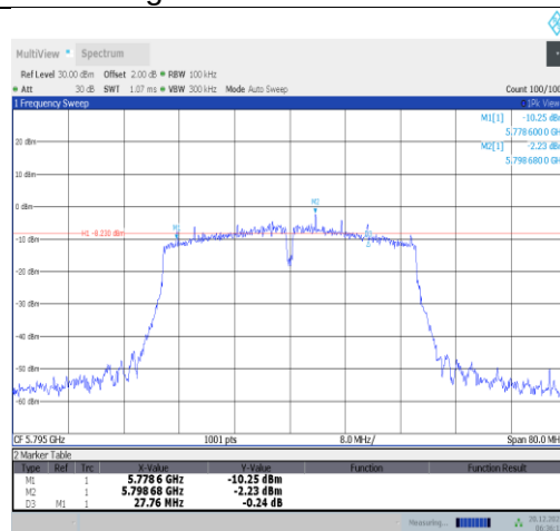
11n40SISO-Ant3-5795-PASS
