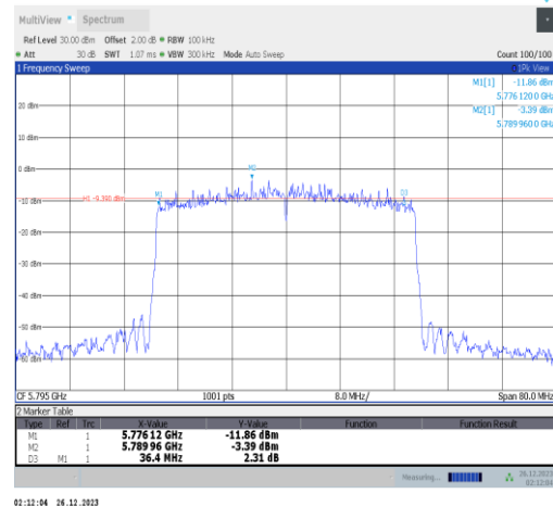
11ax40MIMO-Ant4-5795-PASS
