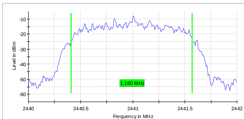
99 % Bandwidth
