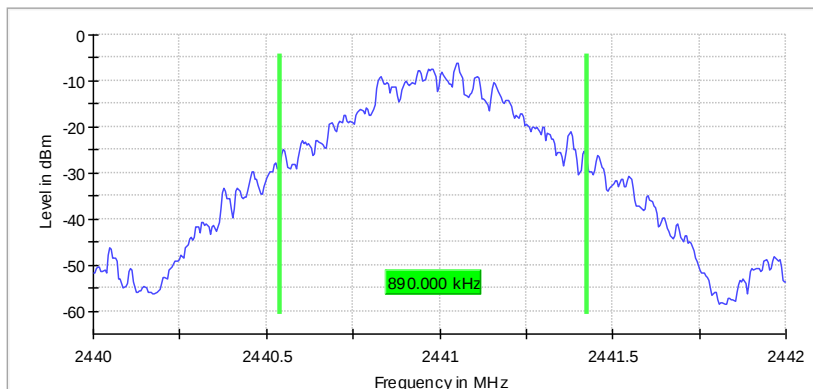
20 dB Bandwidth
