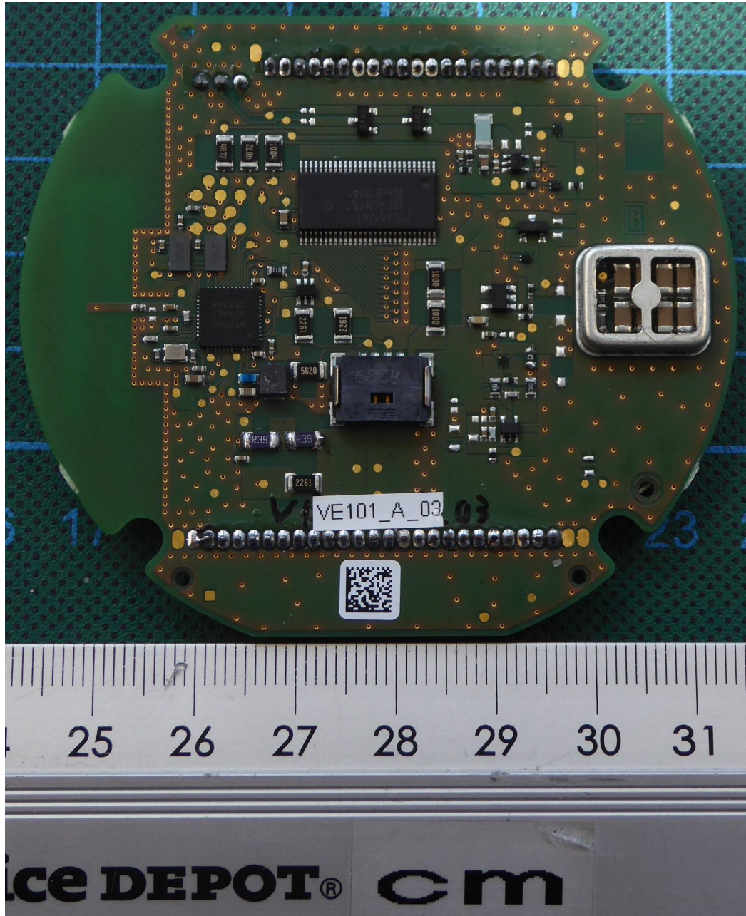
VE_101_A_03 – PCP bottom view
