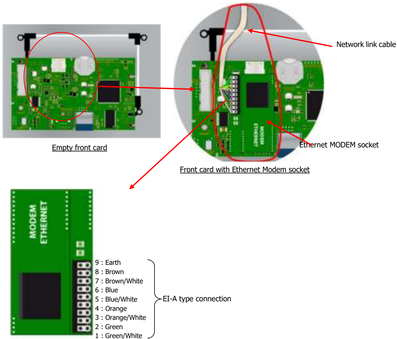
Network cable connection on the modem
