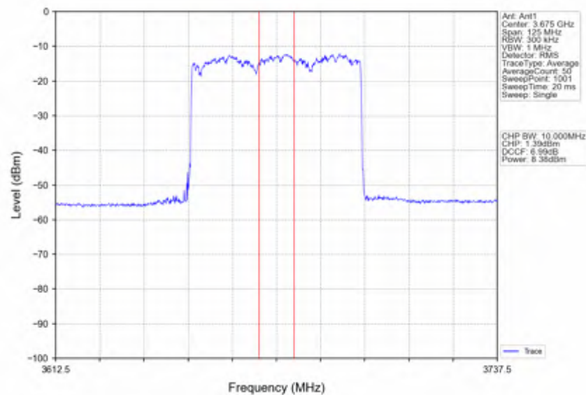
n78d_30kHz_SISO_NTNV_50MHz_CP-OFDM 16 QAM_3675MHz_Inner_Full
