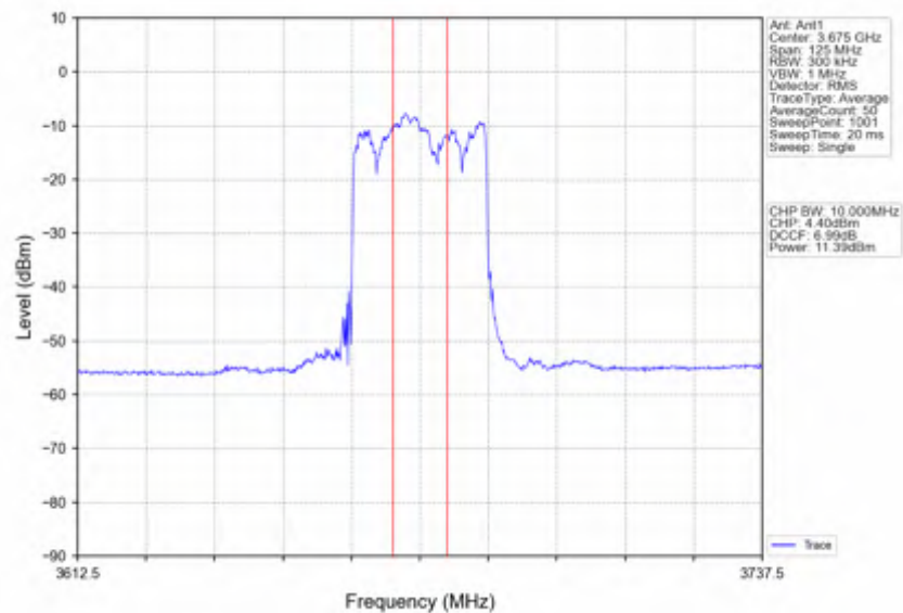
n78d_30kHz_SISO_NTNV_50MHz_CP-OFDM_256_QAM_3675MHz_Inner_Full
