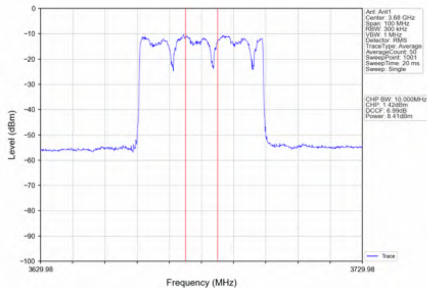
n78d_30kHz_SISO_NTNV_40MHz_CP-OFDM 256 QAM_3679.98MHz_Inner_Full
