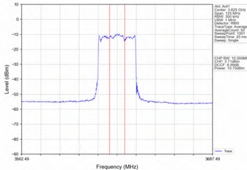
n78d_30kHz_SISO_NTNV_50MHz_CP-OFDM 16 QAM_3624.99MHz_Inner_Full
