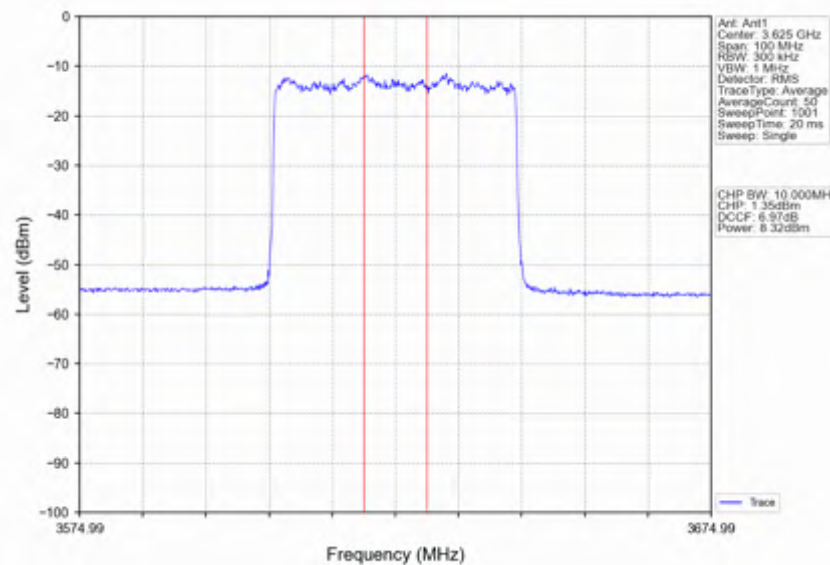
n78d_30kHz_SISO_NTNV_40MHz_CP-OFDM_QPSK_3624.99MHz_Inner_Full
