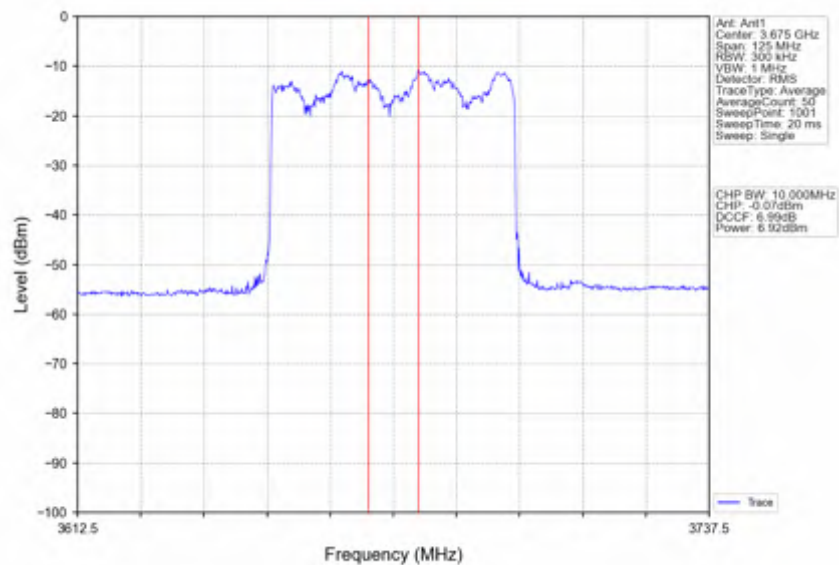
n78d_30kHz_SISO_NTNV_50MHz_CP-OFDM_256_QAM_3675MHz_Inner_Full
