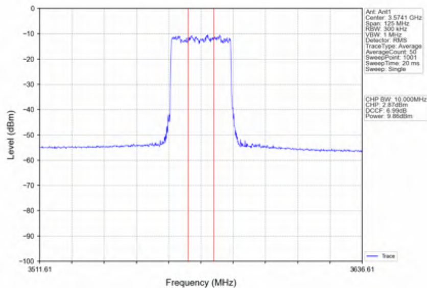
n78d 30kHz SISO NTNV 50MHz DFT-s-OFDM QPSK 3575.01MHz Inner Full
