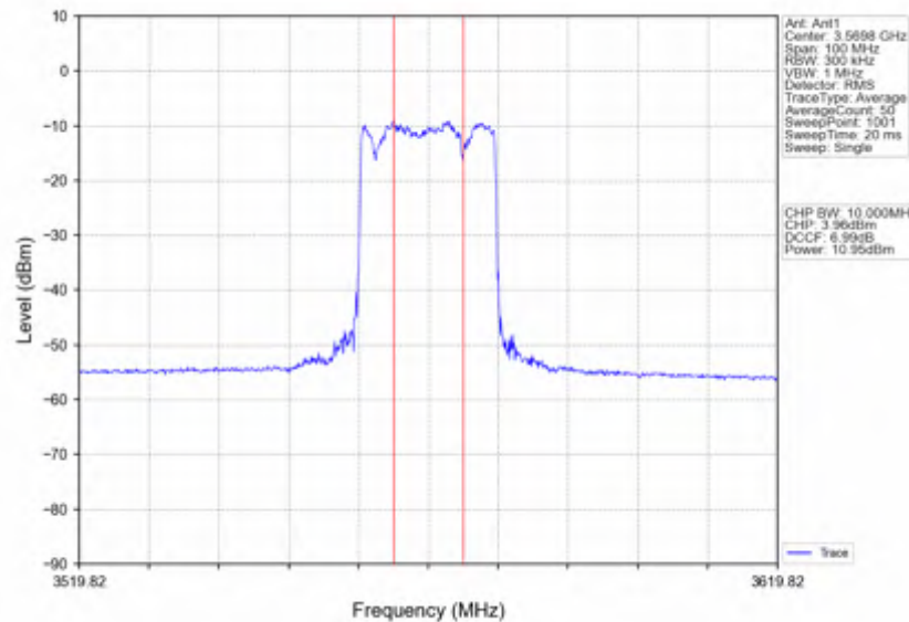
n78d_30kHz_SISO_NTNV_40MHz_CP-OFDM 64 QAM_3570MHz_Inner_Full
