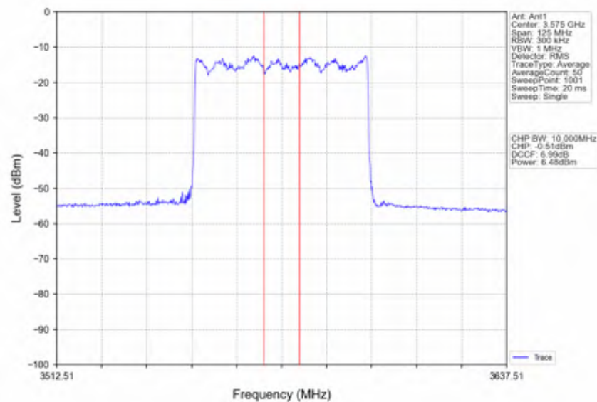
n78d_30kHz_SISO_NTNV_50MHz_CP-OFDM 64 QAM_3575.01MHz_Inner_Full
