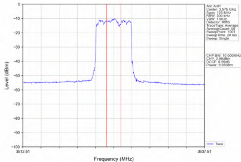
n78d_30kHz_SISO_NTNV_50MHz_CP-OFDM 16 QAM 3575.01MHz_Inner_Full
