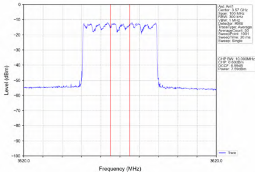
n78d_30kHz_SISO_NTNV_40MHz_CP-OFDM 64 QAM_3570MHz_Inner_Full
