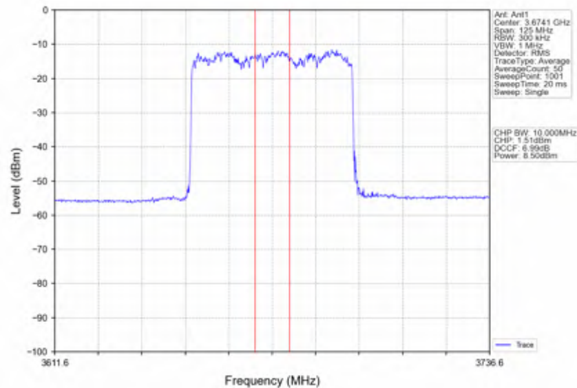
n78d_30kHz_SISO_NTNV_50MHz_DFT-s-OFDM 64 QAM_3675MHz_Inner_Full
