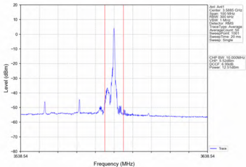
n78d_30kHz_SISO_NTNV_40MHz_CP-OFDM 16 QAM_3570MHz_Inner_1RB_Right
