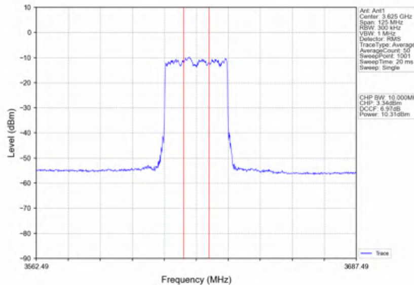
n78d_30kHz_SISO_NTNV_50MHz_CP-OFDM 64 QAM_3624.99MHz_Inner_Full
