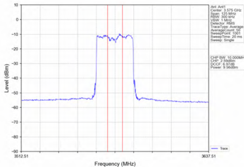
n78d_30kHz_SISO_NTNV_50MHz_CP-OFDM 64 QAM_3575.01MHz_Inner_Full
