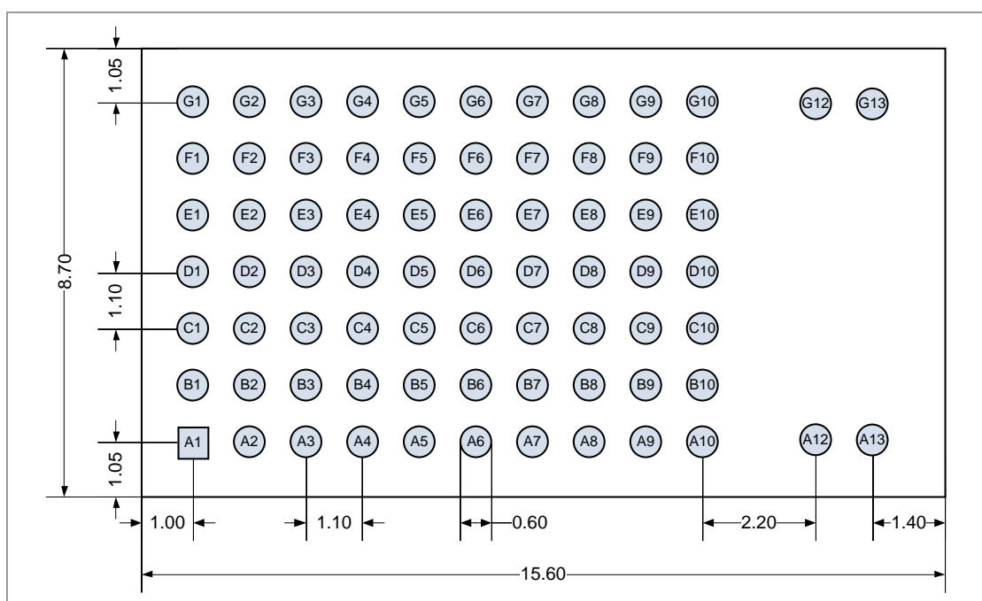
Top View
