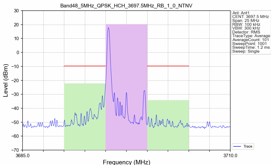
Band48_5MHz_QPSK_HCH_3697.5MHz_RB_1_0_NTNV
