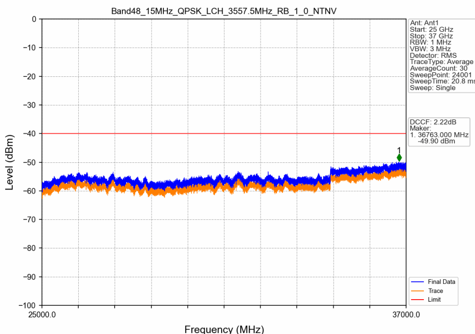
Band48_15MHz_QPSK_LCH_3557.5MHz_RB_1_0_NTNV
