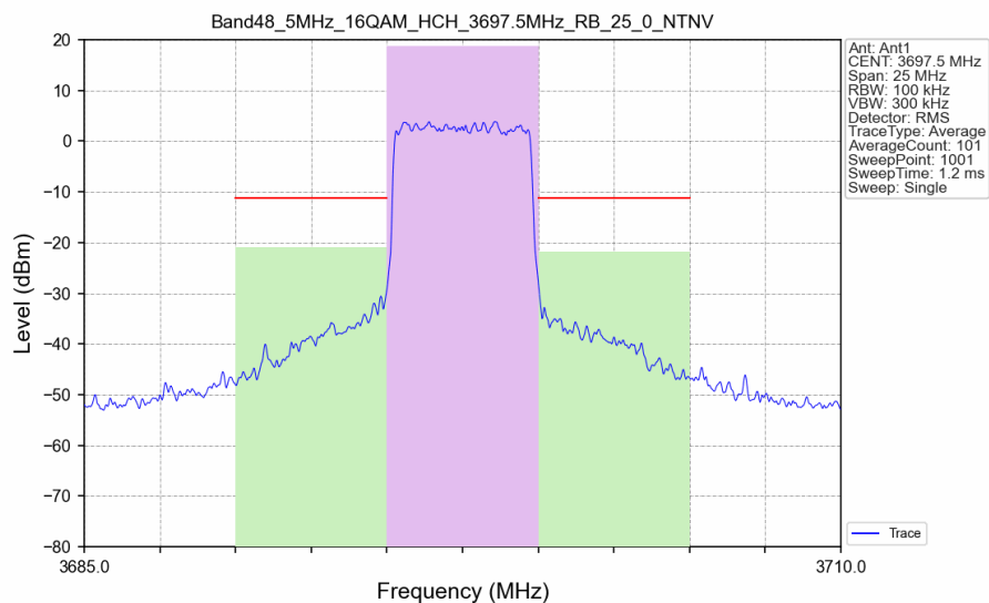
Band48_5MHz_16QAM_HCH_3697.5MHz_RB_25_0_NTNV
