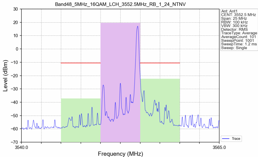
Band48_5MHz_16QAM_LCH_3552.5MHz_RB_1_24_NTNV
