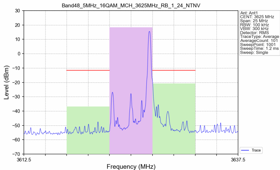
Band48_5MHz_16QAM_MCH_3625MHz_RB_1_24_NTNV
