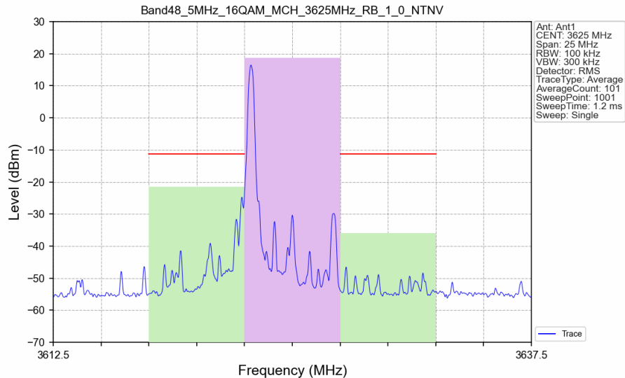
Band48_5MHz_16QAM_MCH_3625MHz_RB_1_0_NTNV
