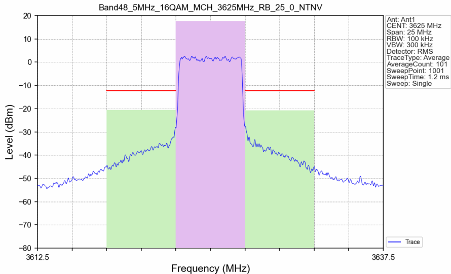
Band48_5MHz_16QAM_MCH_3625MHz_RB_25_0_NTNV
