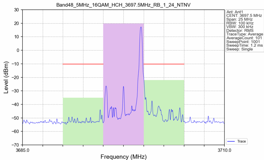
Band48_5MHz_16QAM_HCH_3697.5MHz_RB_1_24_NTNV
