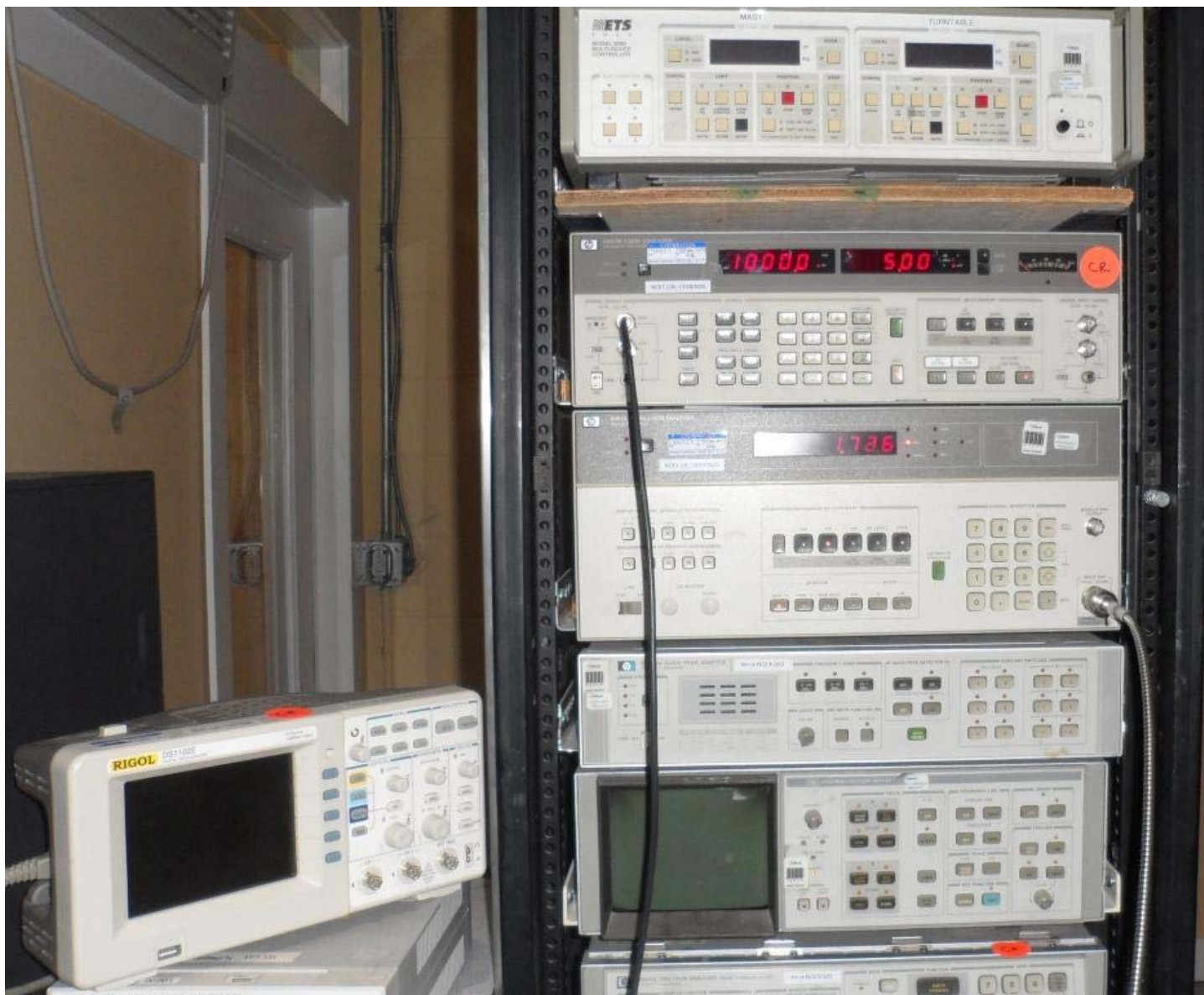
Figure E20.3 – Setup Photo – Audio Response Measurements
