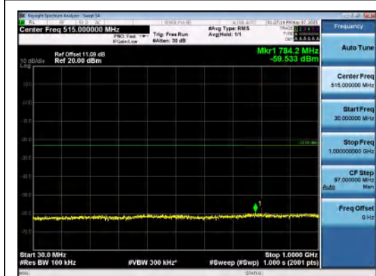
Band66-1.4MHz-QPSK-131979-1RB#0-30~1000-PASS
