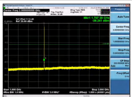
Band66-1.4MHz-QPSK-131979-1RB#0-1000~3000-PASS
