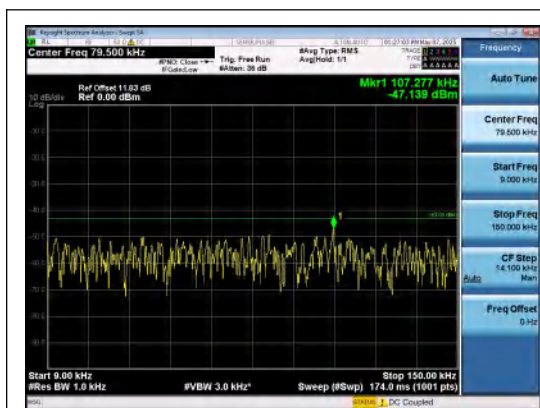
Band66-1.4MHz-QPSK-131979-1RB#0-0.009~0.15-PASS
