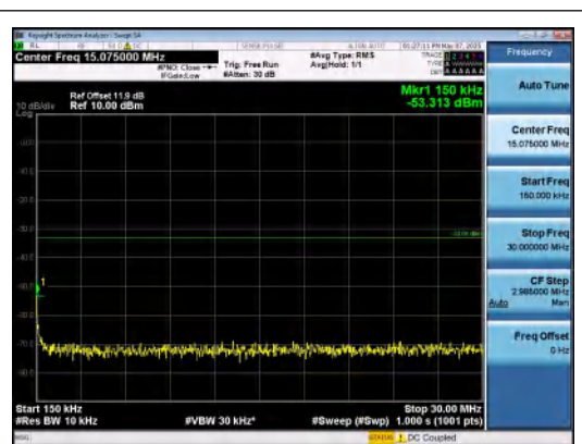
Band66-1.4MHz-QPSK-131979-1RB#0-0.15~30-PASS
