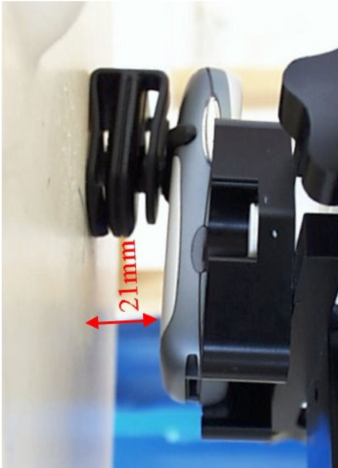
Fig. 43: Body worn configuration, Belt Clip without Headset, (1 TX slot / 2 TX slots).
