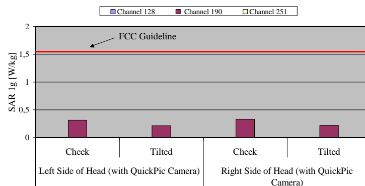
Fig. 8: The measured head phantom SAR values for the Siemens S56 with QuickPic Camera for GSM 850 in comparison to the FCC exposure limit.
