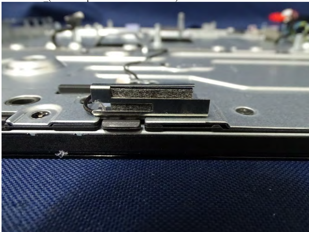
(17) EUT Photo ( VSO Corporation - Main Antenna)
