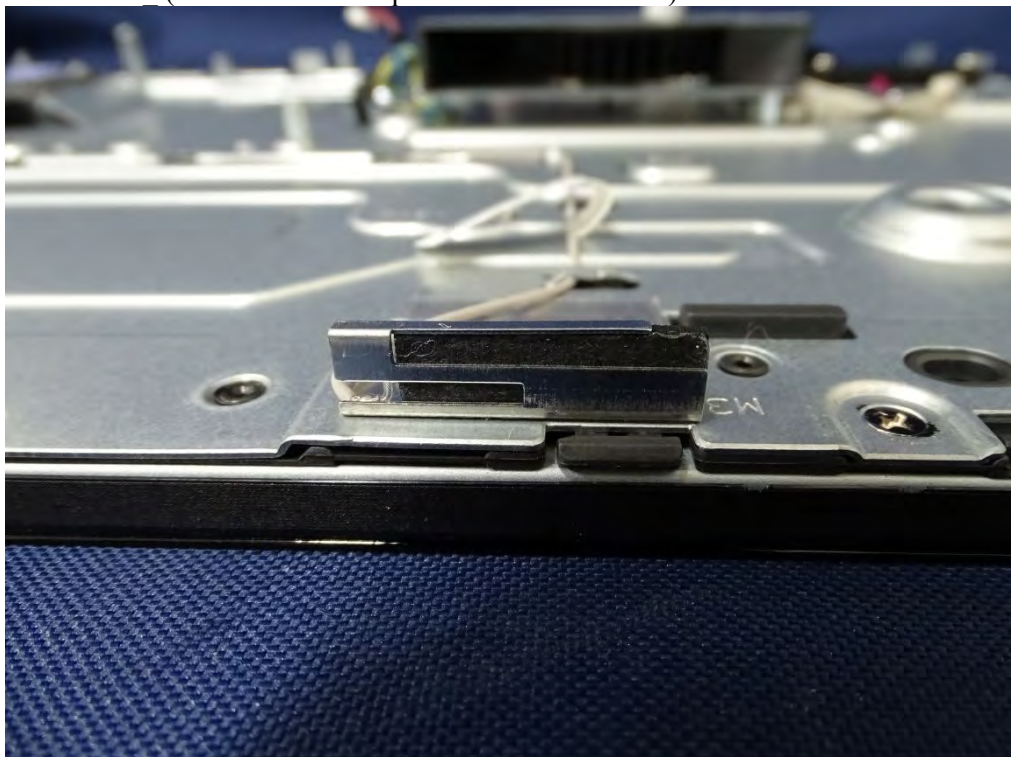
(16) EUT Photo (Luxshare-ICT Corporation - Aux Antenna)
