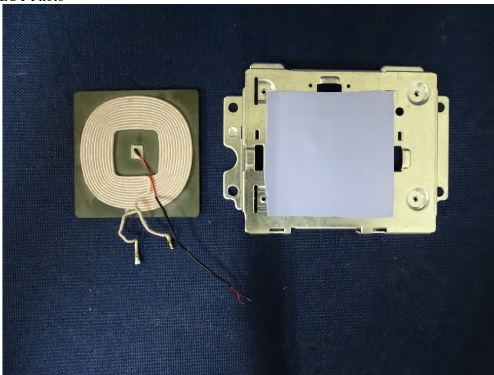
(43) EUT Photo
