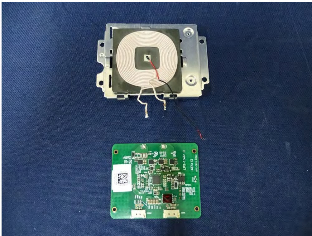
(42) EUT Photo
