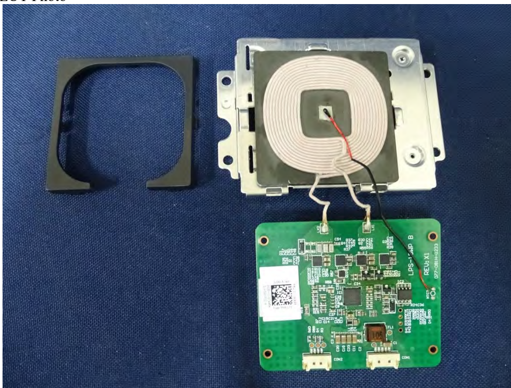
(39) EUT Photo
