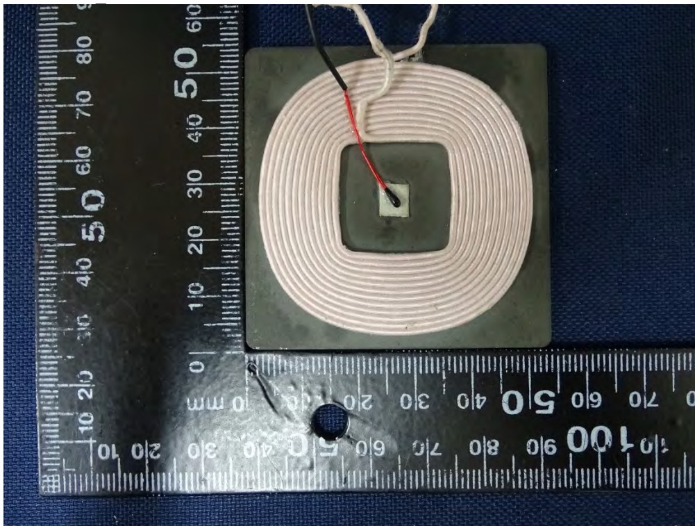
(44) EUT Photo WPT Antenna
