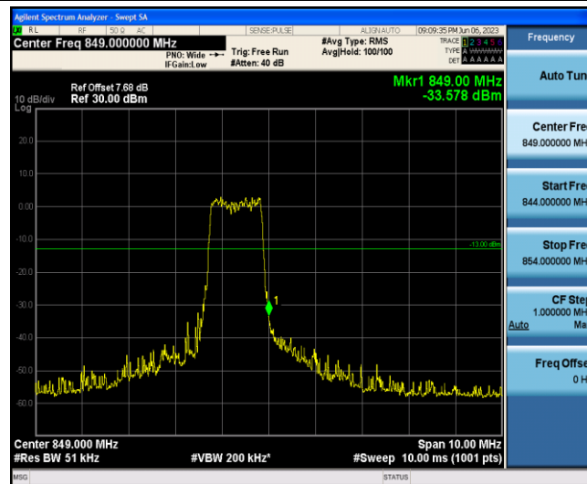
Band5-1.4MHz-QPSK-20643-6-0-High--33.58-PASS
