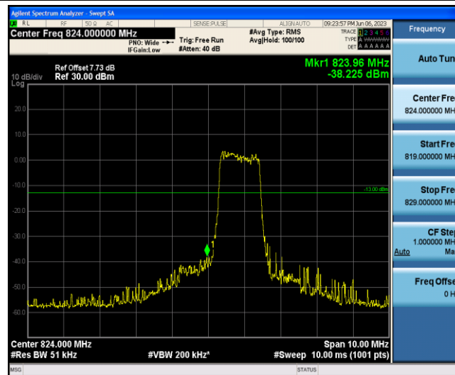
Band5-3MHz-QPSK-20415-6-0-Low--38.23-PASS
