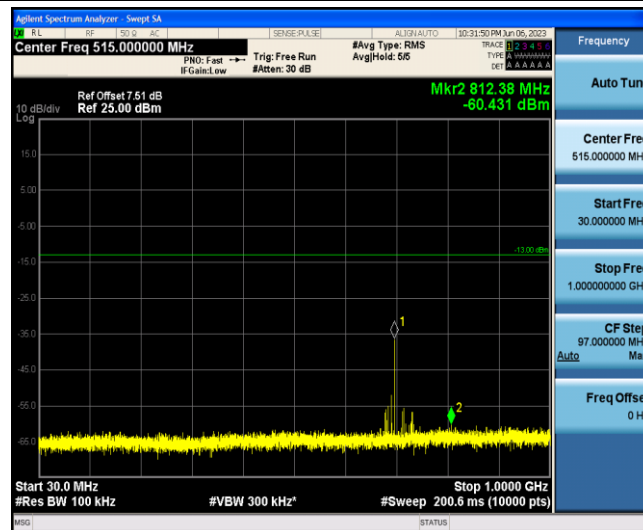
Band12-3MHz-16QAM-23095-1-0-Low-30-1000--60.43-PASS
