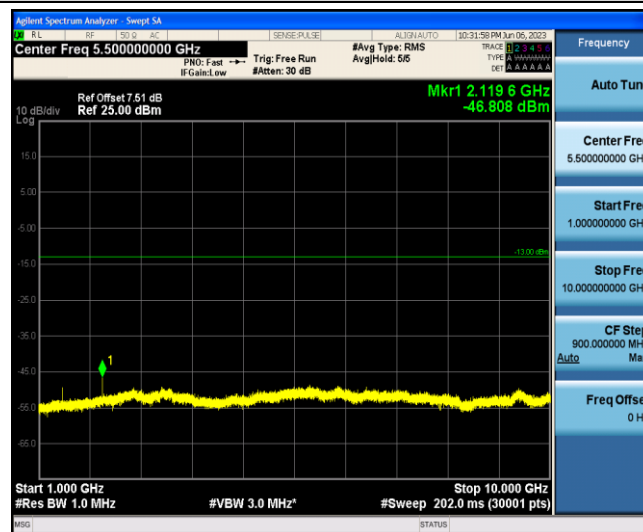
Band12-3MHz-16QAM-23095-1-0-Low-1000-10000--46.81-PASS
