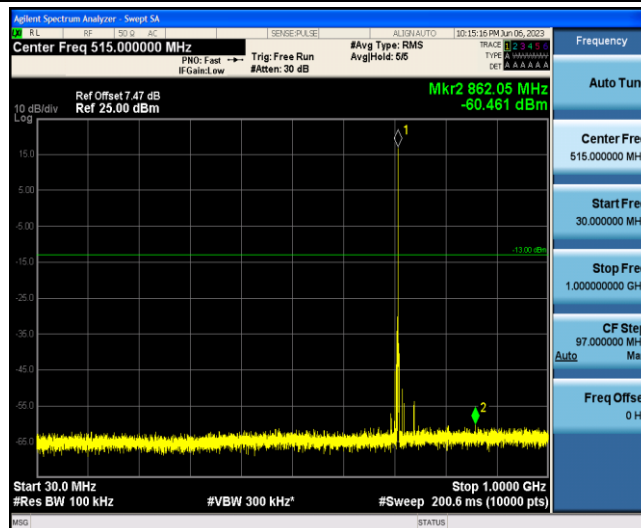
Band12-1.4MHz-QPSK-23173-1-0-Low-30-1000--60.46-PASS
