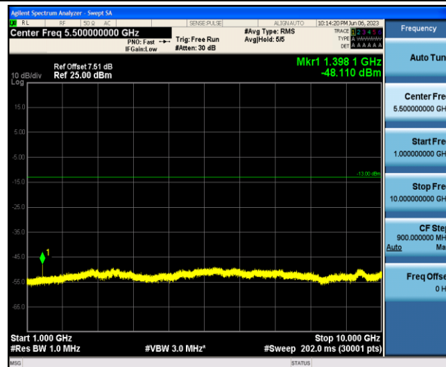
Band12-1.4MHz-16QAM-23017-1-0-Low-1000-10000--48.11-PASS
