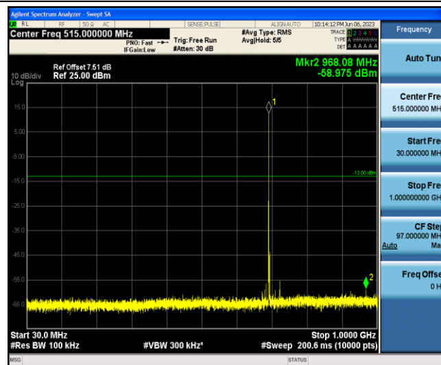
Band12-1.4MHz-16QAM-23017-1-0-Low-30-1000--58.98-PASS
