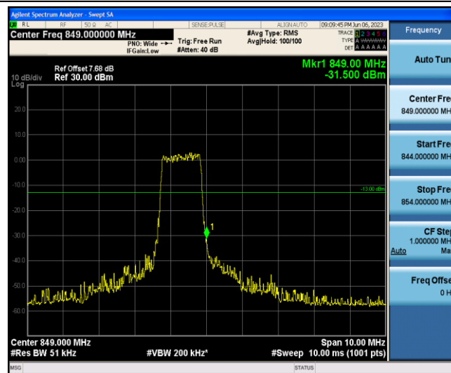
Band5-1.4MHz-16QAM-20643-6-0-High--31.50-PASS
