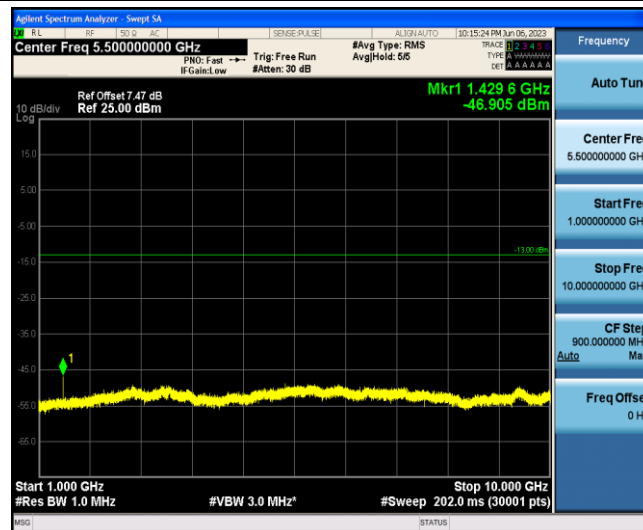
Band12-1.4MHz-QPSK-23173-1-0-Low-1000-10000--46.91-PASS
