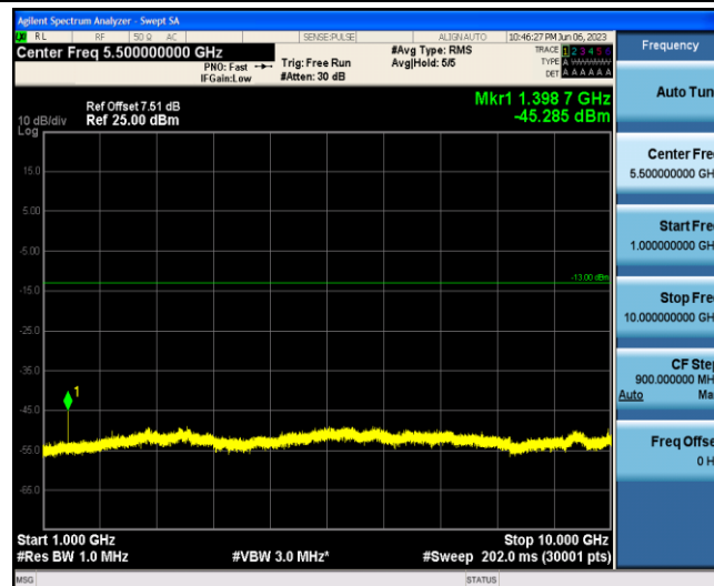
Band12-5MHz-QPSK-23035-1-0-Low-1000-10000--45.29-PASS
