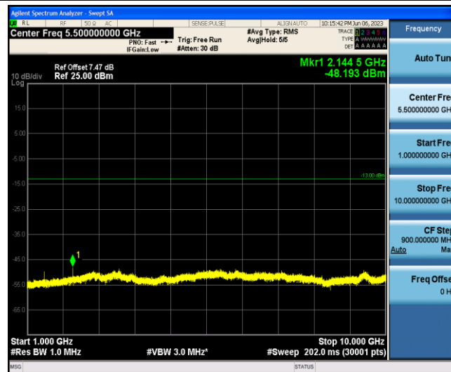
Band12-1.4MHz-16QAM-23173-1-0-Low-1000-10000--48.19-PASS
