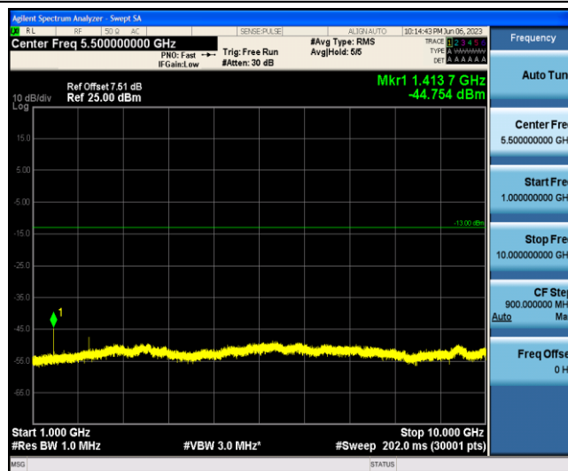
Band12-1.4MHz-QPSK-23095-1-0-Low-1000-10000--44.75-PASS
