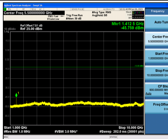
Band12-3MHz-QPSK-23095-1-0-Low-1000-10000--45.76-PASS
