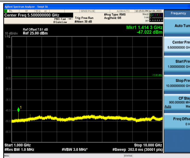
Band12-1.4MHz-16QAM-23095-1-0-Low-1000-10000--47.02-PASS
