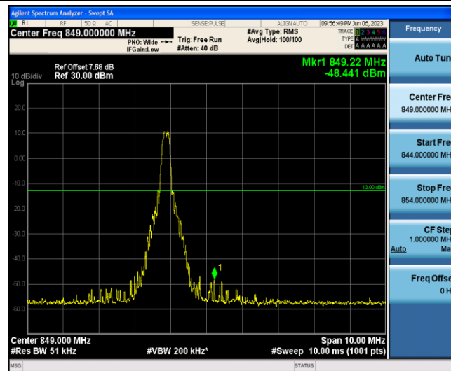
Band5-10MHz-16QAM-20600-1-5-High--48.44-PASS
