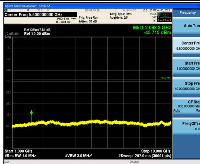
Band12-3MHz-16QAM-23025-1-0-Low-1000-10000--45.72-PASS
