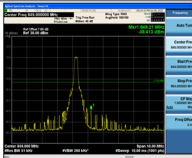
Band5-3MHz-16QAM-20635-1-5-High--39.41-PASS
