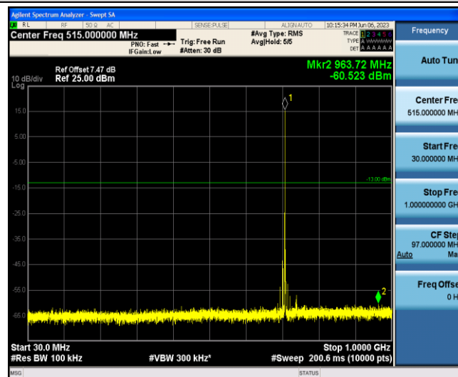
Band12-1.4MHz-16QAM-23173-1-0-Low-30-1000--60.52-PASS
