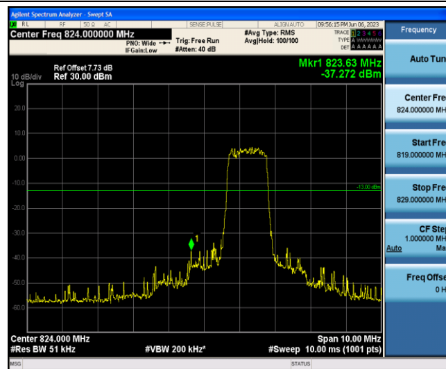
Band5-10MHz-QPSK-20450-6-0-Low--37.27-PASS
