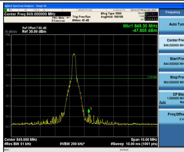
Band5-5MHz-16QAM-20625-1-5-High--47.60-PASS
