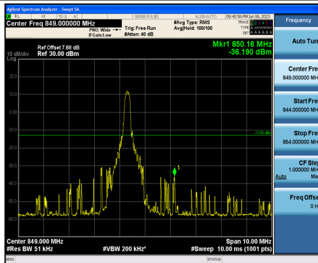
Band5-5MHz-QPSK-20625-1-5-High--36.19-PASS
