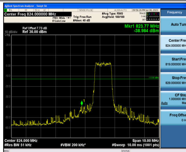
Band5-10MHz-16QAM-20450-6-0-Low--38.98-PASS
