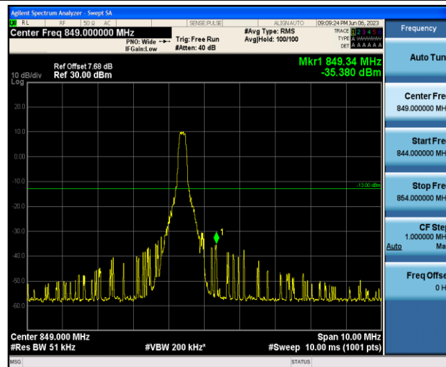
Band5-1.4MHz-16QAM-20643-1-5-High--35.38-PASS
