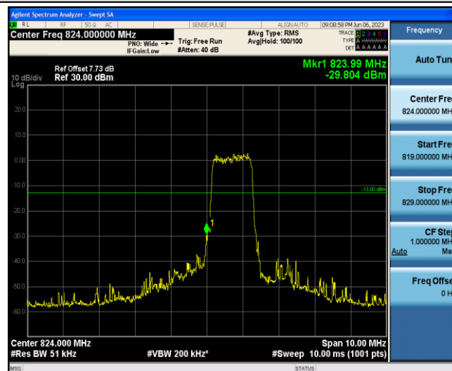
Band5-1.4MHz-16QAM-20407-6-0-Low--29.80-PASS
