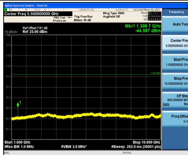
Band12-1.4MHz-QPSK-23017-1-0-Low-1000-10000--44.59-PASS
