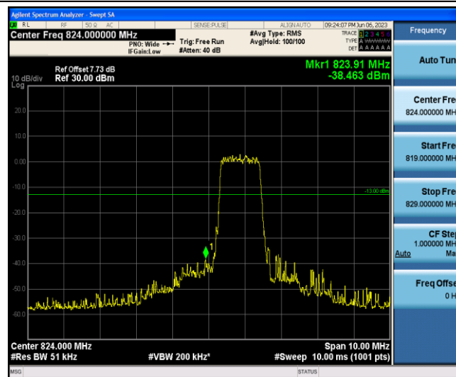
Band5-3MHz-16QAM-20415-6-0-Low--38.46-PASS
