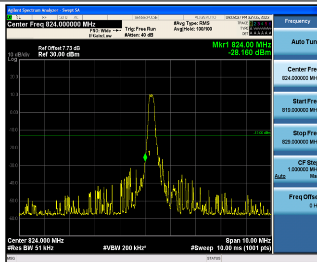
Band5-1.4MHz-16QAM-20407-1-0-Low--28.16-PASS
