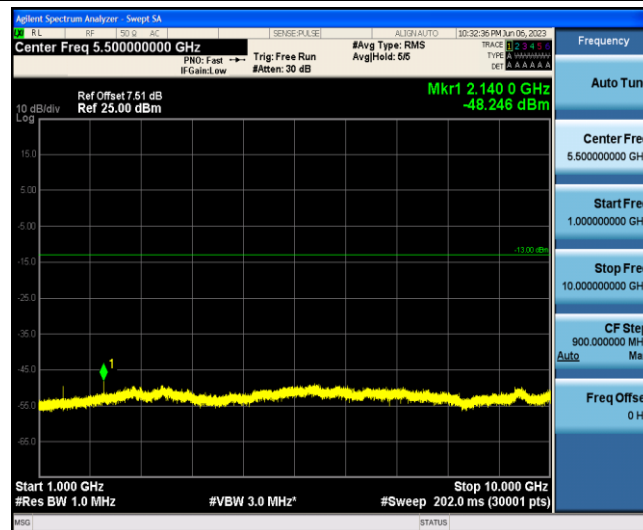
Band12-3MHz-16QAM-23165-1-0-Low-1000-10000--48.25-PASS
