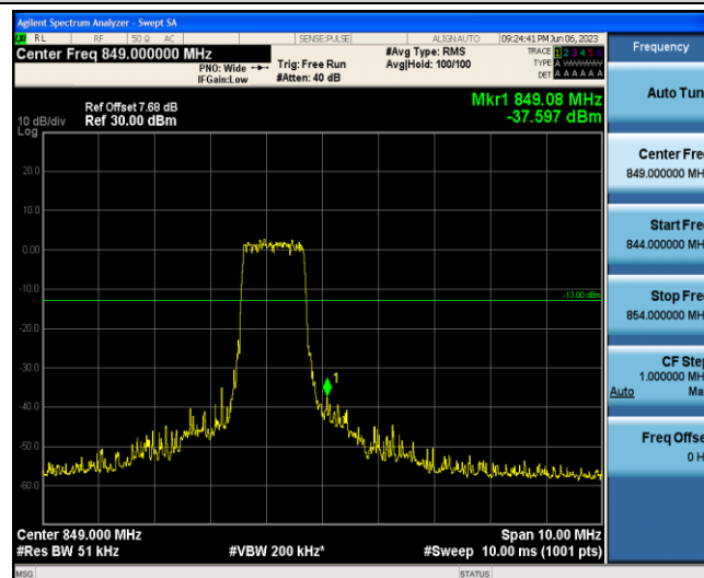
Band5-3MHz-QPSK-20635-6-0-High--37.60-PASS
