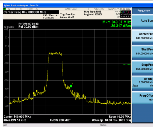
Band5-10MHz-16QAM-20600-6-0-High--39.32-PASS
