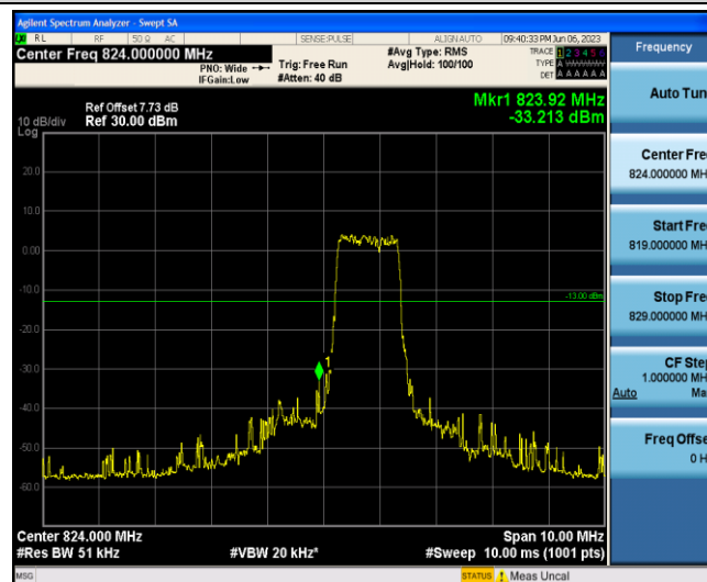
Band5-5MHz-QPSK-20425-6-0-Low--33.21-PASS
