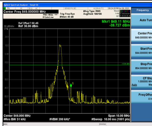
Band5-3MHz-QPSK-20635-1-5-High--39.73-PASS
