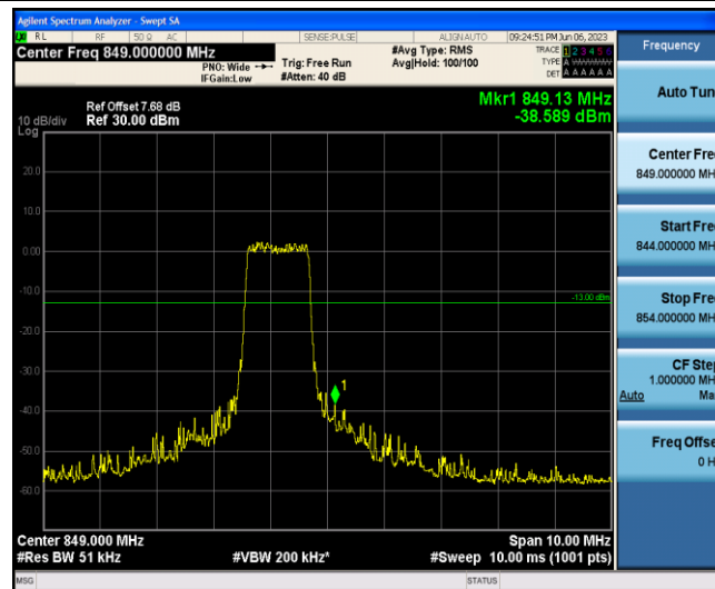
Band5-3MHz-16QAM-20635-6-0-High--38.59-PASS
