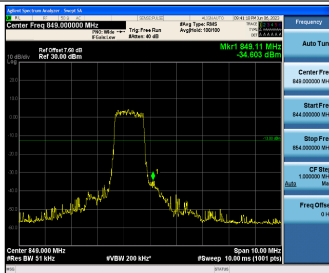
Band5-5MHz-QPSK-20625-6-0-High--34.60-PASS
