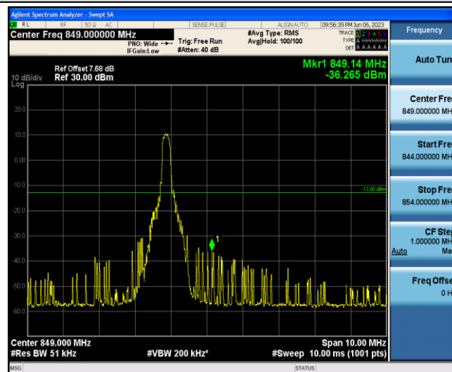
Band5-10MHz-QPSK-20600-1-5-High--36.27-PASS
