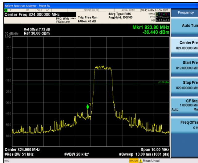
Band5-5MHz-16QAM-20425-6-0-Low--36.44-PASS
