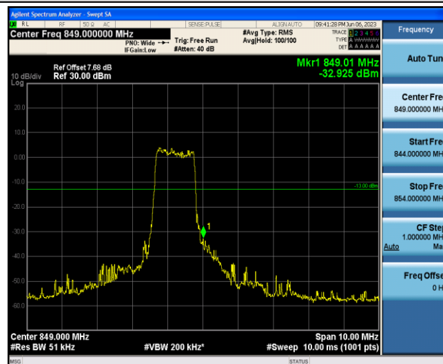
Band5-5MHz-16QAM-20625-6-0-High--32.93-PASS
