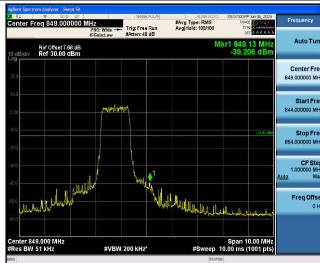
Band5-10MHz-QPSK-20600-6-0-High--39.21-PASS
