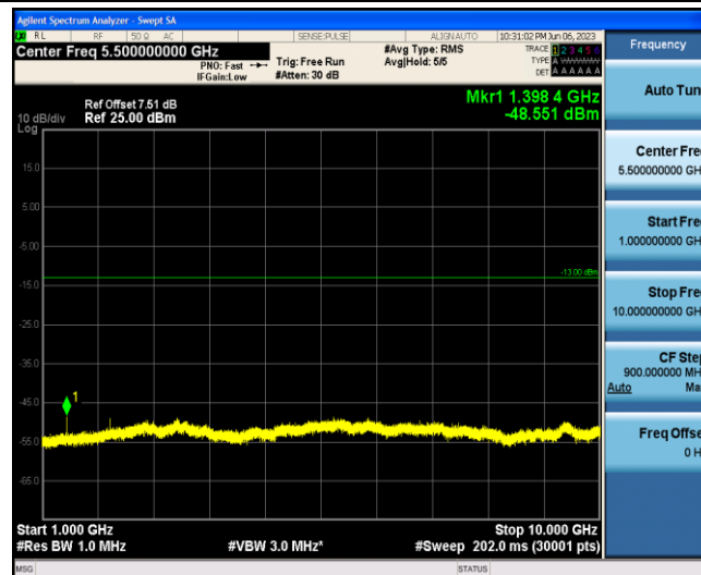
Band12-3MHz-QPSK-23025-1-0-Low-1000-10000--48.55-PASS
