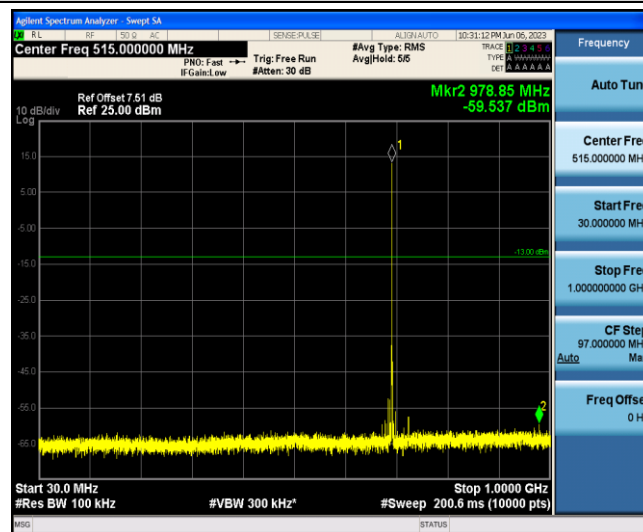
Band12-3MHz-16QAM-23025-1-0-Low-30-1000--59.54-PASS
