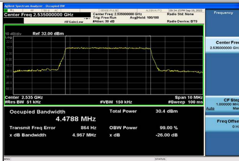
Band7-5MHz-16QAM-21100-25RB#0-4.4788
