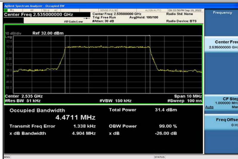
Band7-5MHz-QPSK-21100-25RB#0-4.4711
