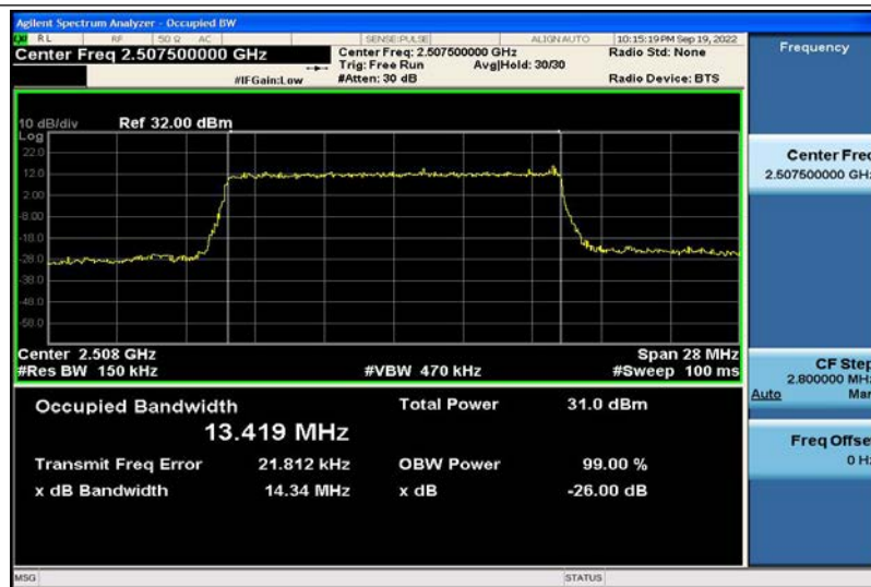
Band7-15MHz-16QAM-20825-75RB#0-13.419
