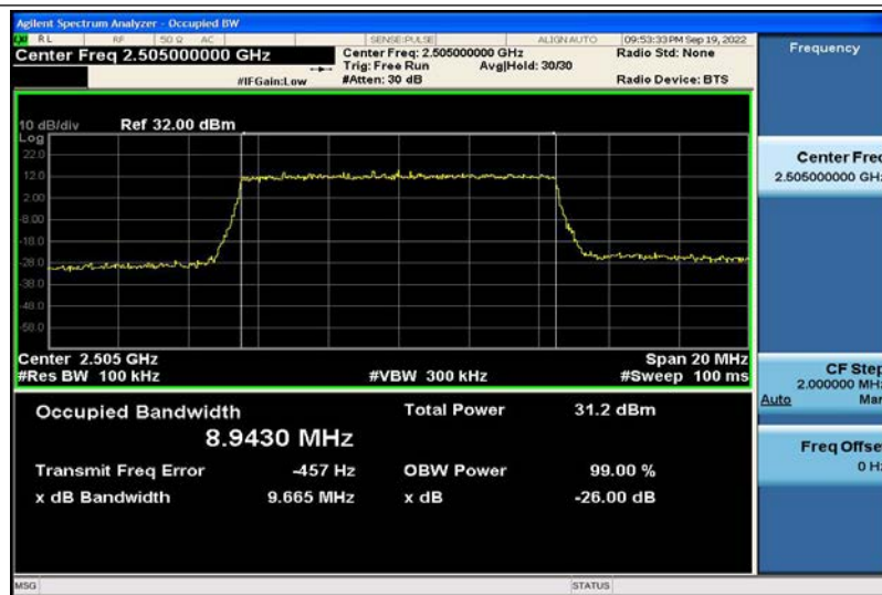
Band7-10MHz-QPSK-20800-50RB#0-8.9430
