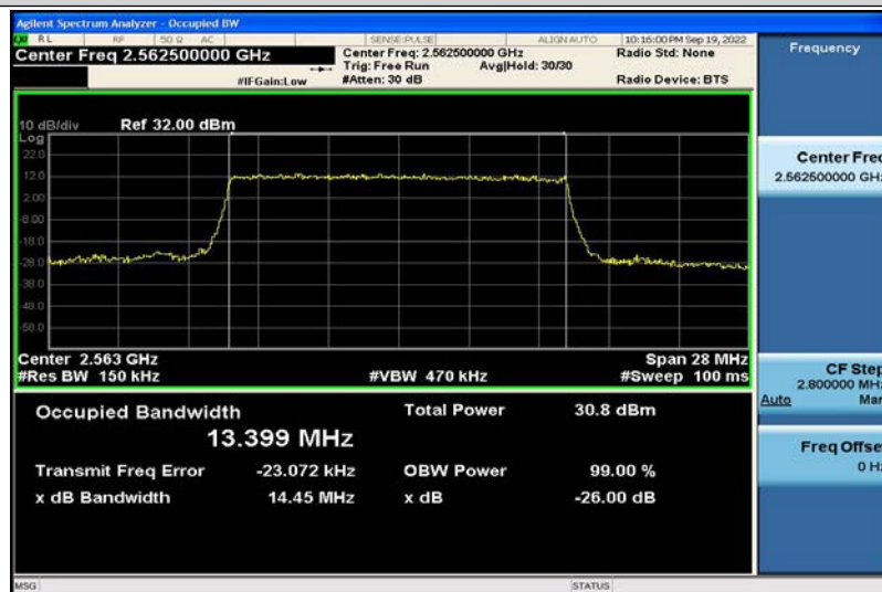
Band7-15MHz-16QAM-21375-75RB#0-13.399
