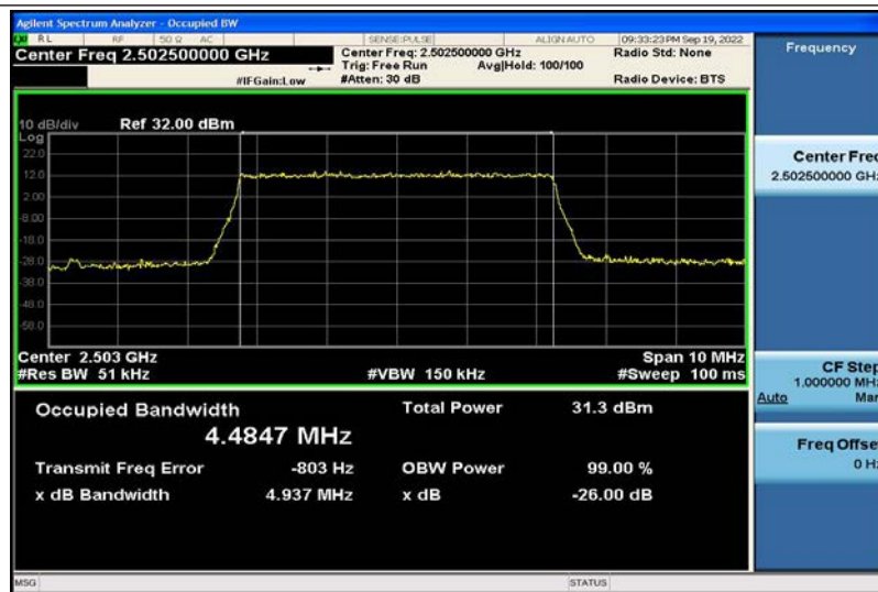
Band7-5MHz-QPSK-20775-25RB#0-4.4847
