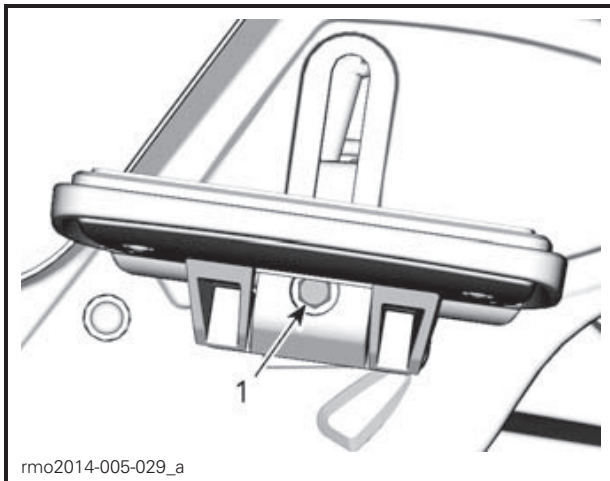
1. Retaining screw
