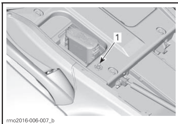
1. Schrader valve
