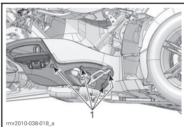
1. Retaining screws
