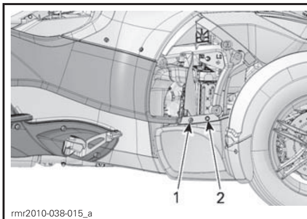
1. Upper retaining screw 2. Upper plastic rivet
