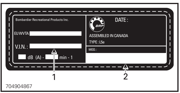
VEHICLE IDENTIFICATION NUMBER LABEL 1. VIN (Vehicle Identification Number) 2. Model number
