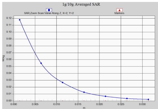
LTE Band38 Body 10mm ANT8
