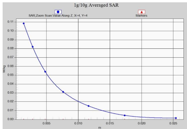
N78 Body 10mm ANT7
