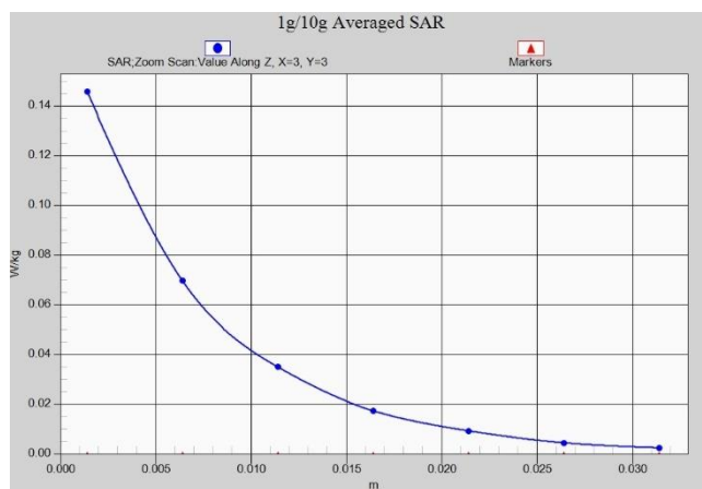
N38 Body 15mm ANT8
