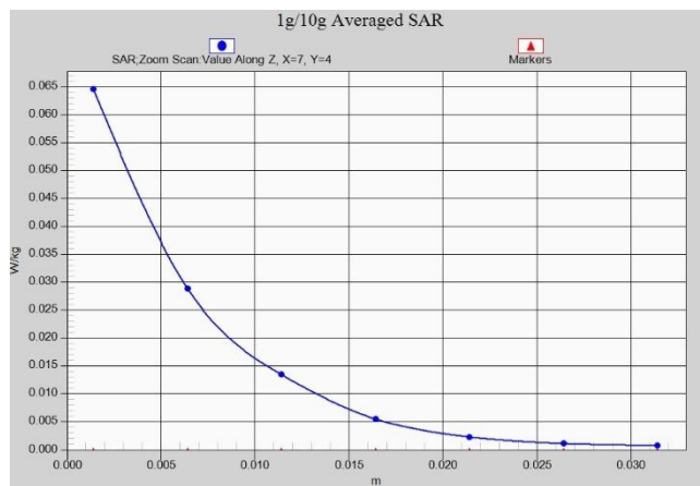
WIFI2.4G Body 15mm ANT6
