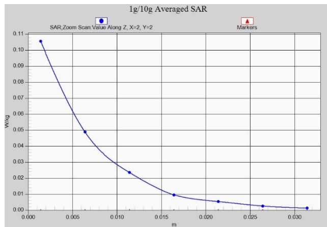
LTE Band41 PC3 Body 10mm ANT8
