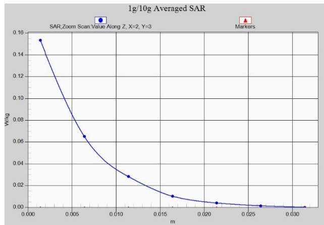
LTE Band41 PC2 Head ANT8
