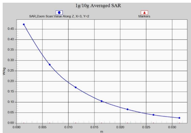
LTE Band25 Body 15mm ANT1
