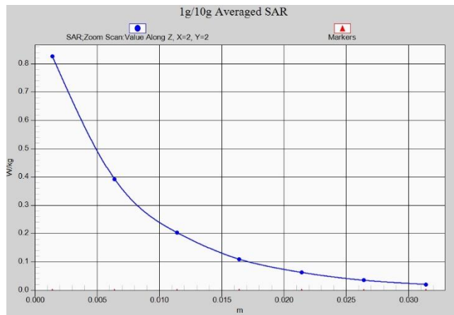
LTE Band66 Head ANT8
