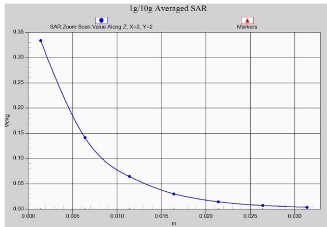
LTE Band38 Head ANT8
