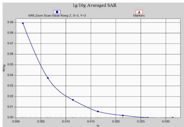
LTE Band38 Body 15mm ANT8
