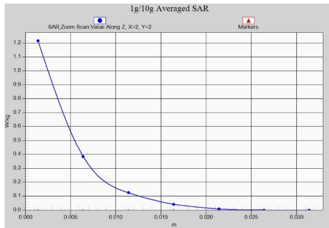
N78 Head ANT6
