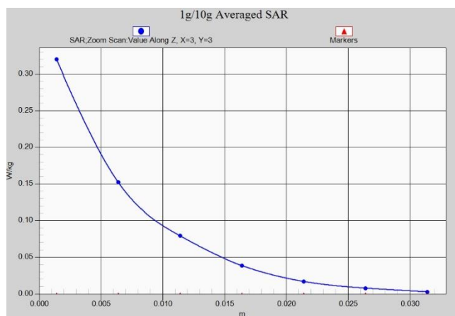
LTE Band41 PC2 Body 15mm ANT4
