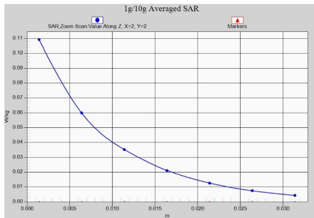
LTE Band66 Body 10mm ANT8
