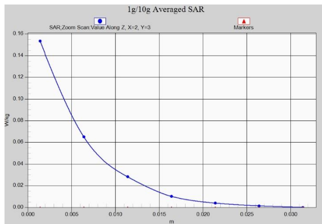
LTE Band41 PC2 Body 15mm ANT2
