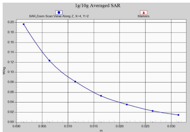
LTE Band66 Body 15mm ANT4
