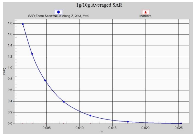
N78 Head ANT4
