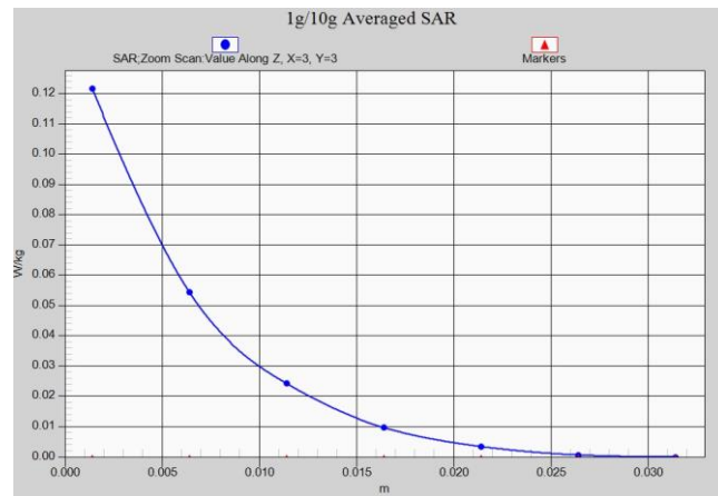
BT Body 10mm ANT8
