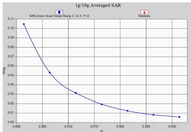
N5 Body 10mm ANT3
