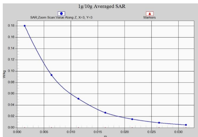
N7 Body 15mm ANT4
