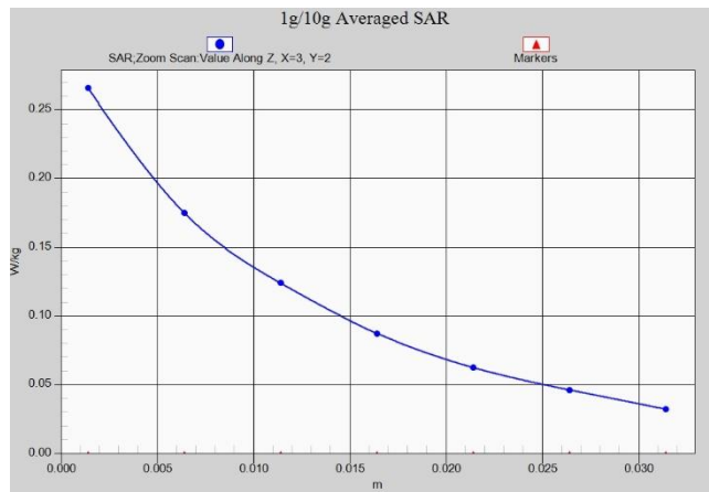
LTE Band66 Head ANT1
