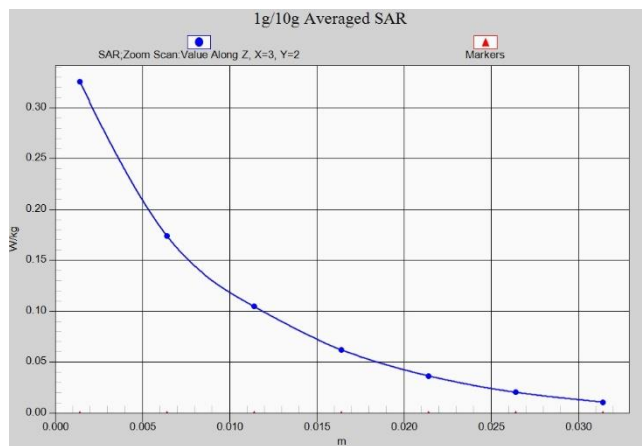
LTE Band66 Body 15mm ANT2
