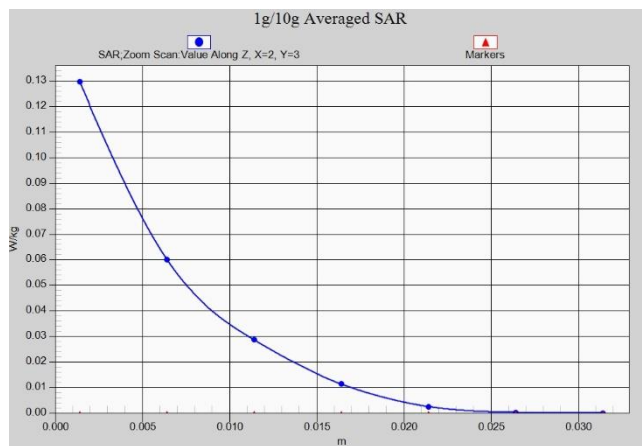
LTE Band41 PC3 Body 15mm ANT2
