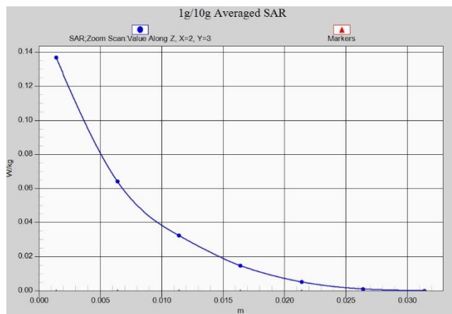
LTE Band38 Body 15mm ANT2
