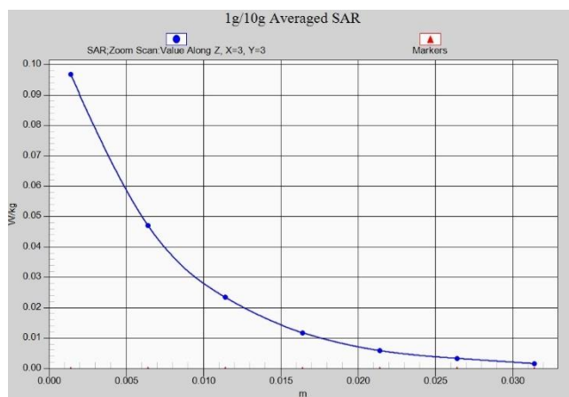
N7 Body 15mm ANT8
