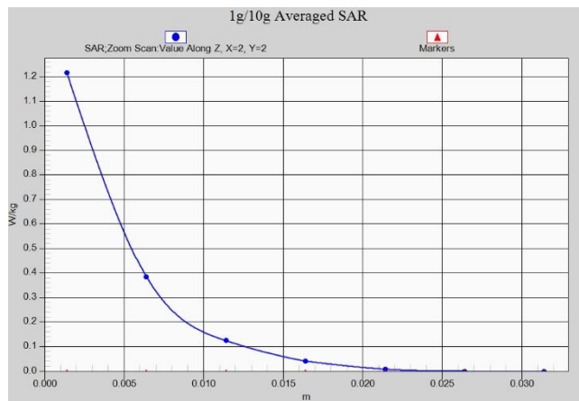
N78 Body 10mm ANT6
