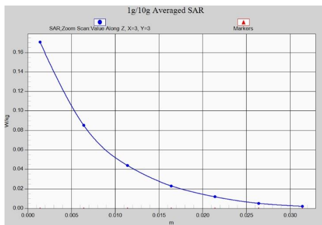
LTE Band41 PC3 Body 15mm ANT4
