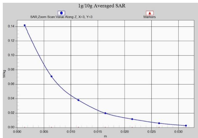
N38 Body 15mm ANT4
