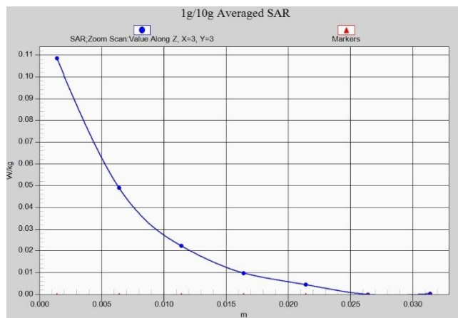
WIFI2.4G Body 15mm ANT8
