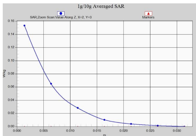
LTE Band41 PC2 Body 15mm ANT8
