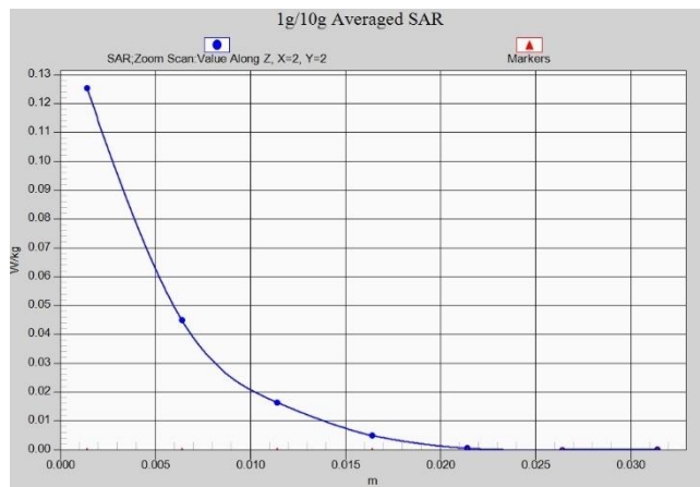
N38 Body 10mm ANT8
