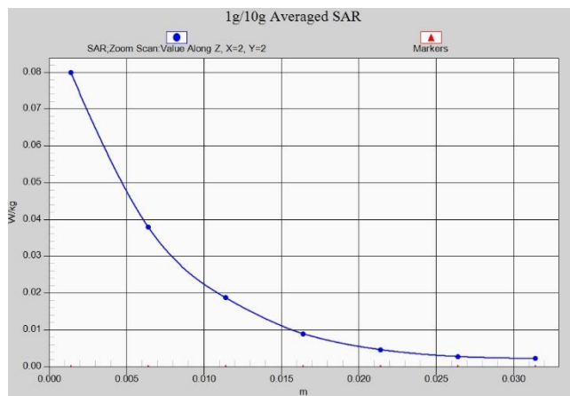
LTE Band41 PC3 Body 15mm ANT8
