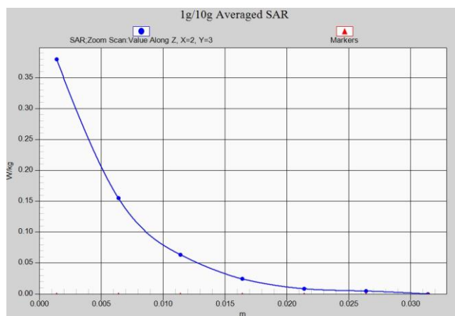
BT Head ANT8
