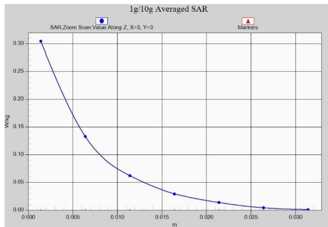
WIFI2.4G Body 10mm ANT8
