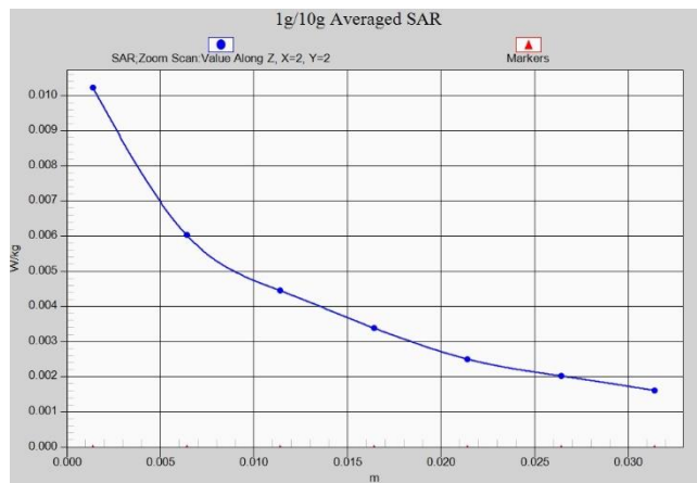
LTE Band26 Body 10mm ANT3
