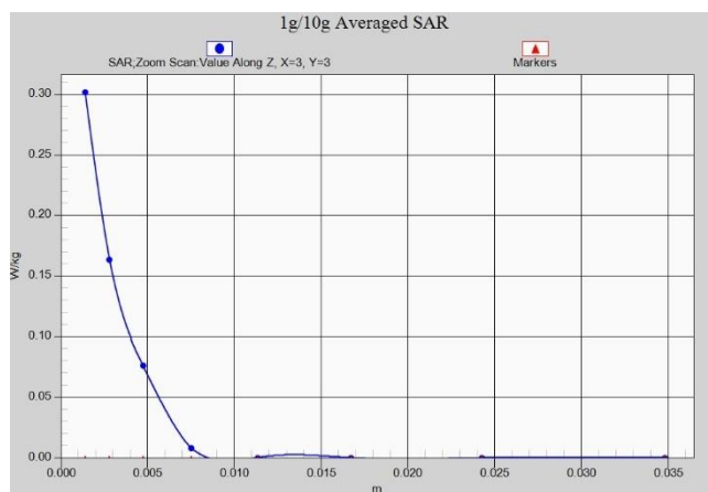
WIFI5G Body 15mm ANT7
