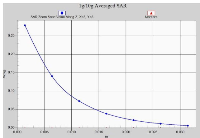
LTE Band38 Body 15mm ANT1
