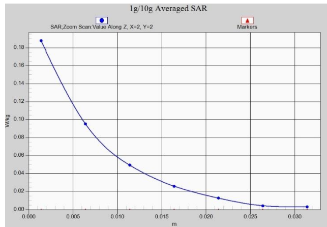
N41 Head ANT1
