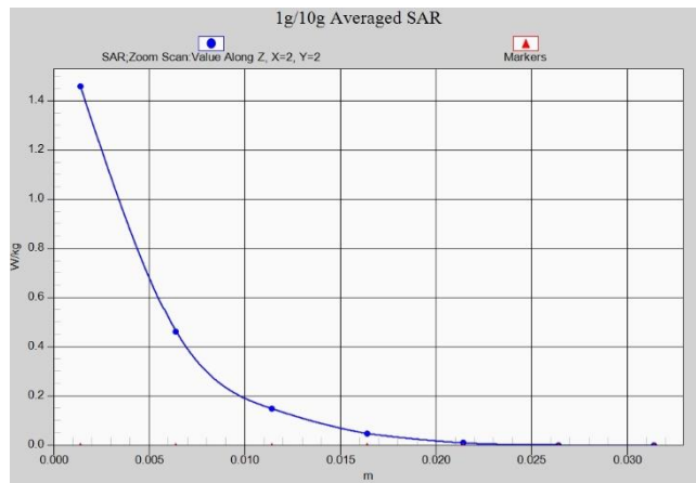
N78 Head ANT7
