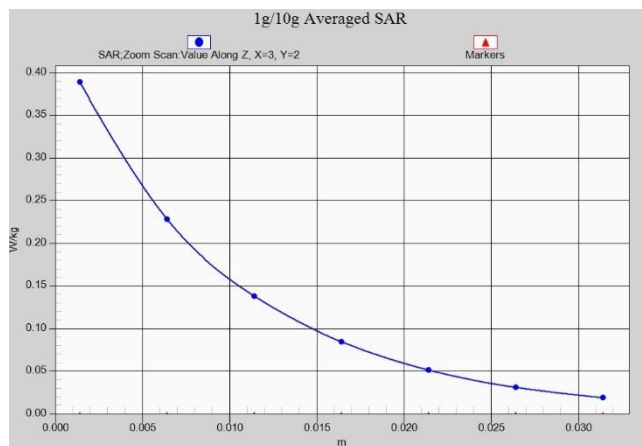
N2 Body 15mm ANT1
