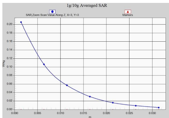
N41 Body 15mm ANT2
