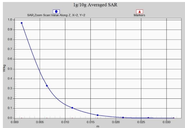
N78 Head ANT2
