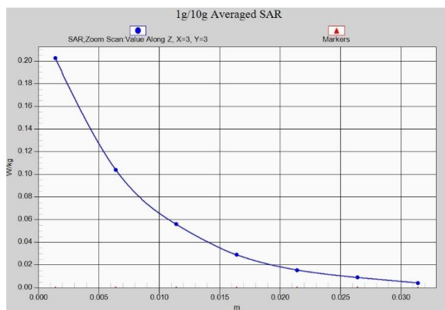
N38 Body 15mm ANT2
