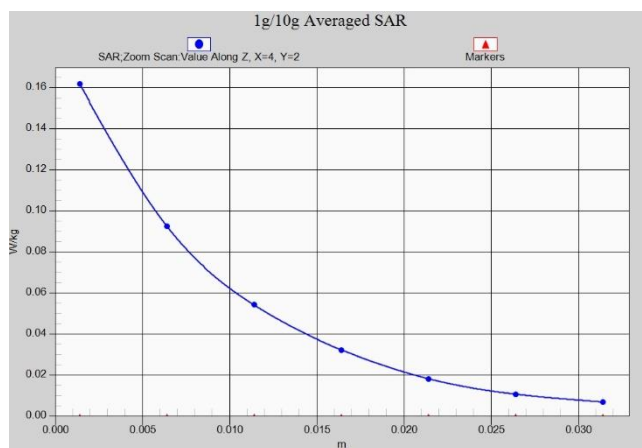
N2 Body 15mm ANT2
