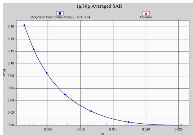
N78 Body 15mm ANT4
