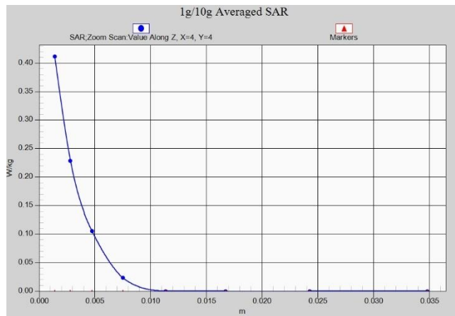
WIFI5G Head ANT6
