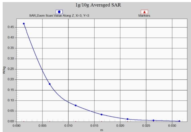
WIFI2.4G Head ANT8
