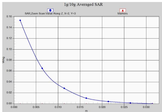
LTE Band41 PC2 Body 10mm ANT8
