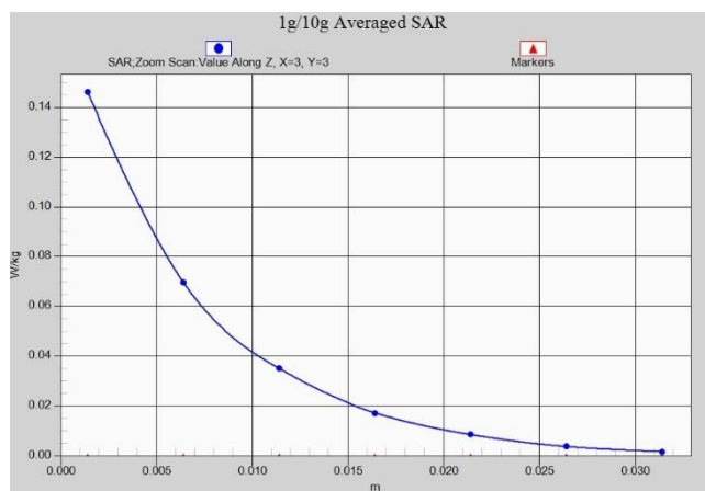
N41 Body 15mm ANT4
