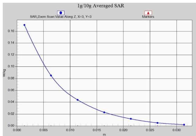
LTE Band41 PC3 Body 15mm ANT1
