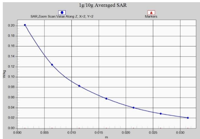
N2 Head ANT1
