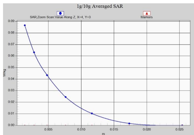
N78 Body 15mm ANT2
