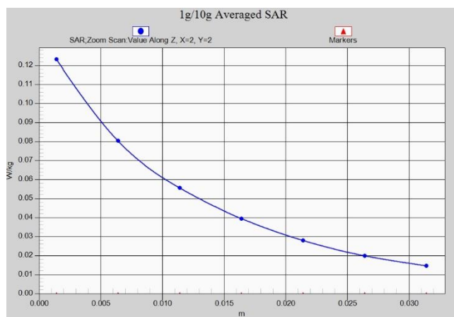
LTE Band26 Body 15mm ANT3
