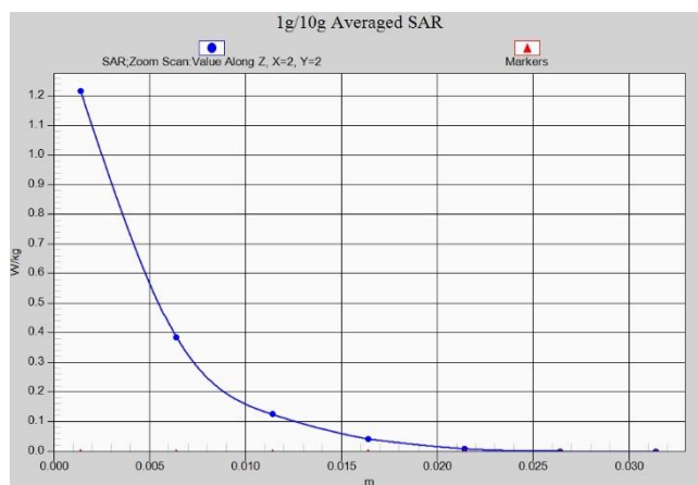
N78 Body 15mm ANT6
