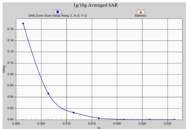
N78 Body 10mm ANT4
