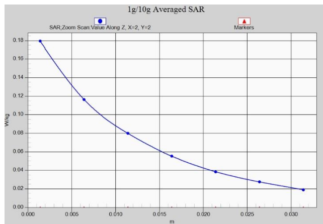
LTE Band26 Body 15mm ANT0
