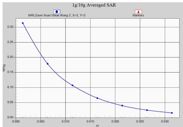
LTE Band66 Body 10mm ANT1
