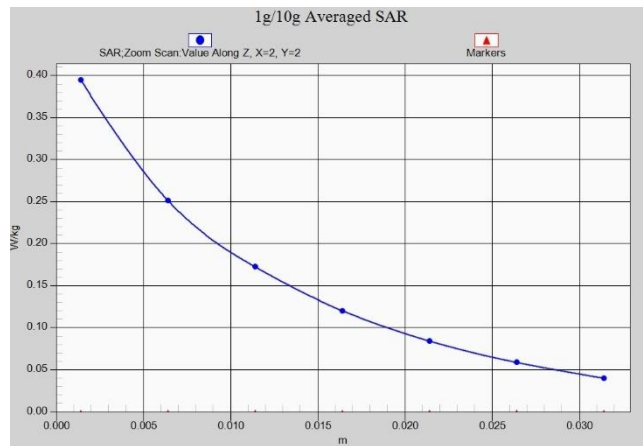
N66 Head ANT1
