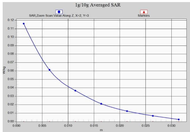
LTE Band41 PC2 Head ANT1
