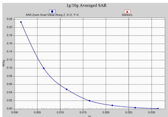
LTE Band41 PC2 Body 15mm ANT1
