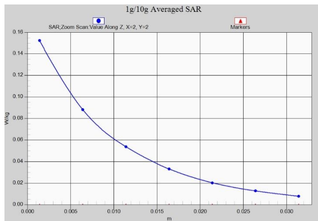
LTE Band66 Body 15mm ANT8
