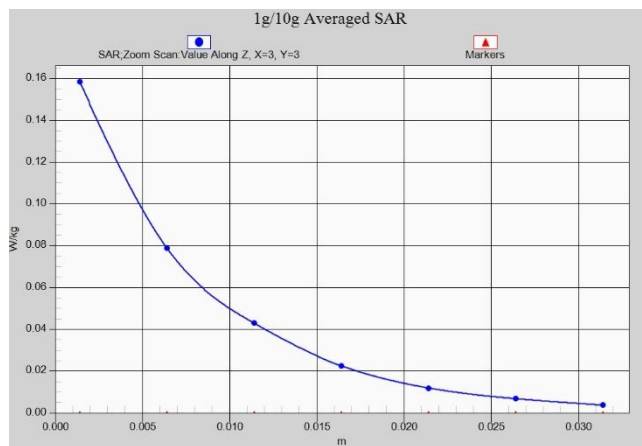
LTE Band38 Body 15mm ANT4
