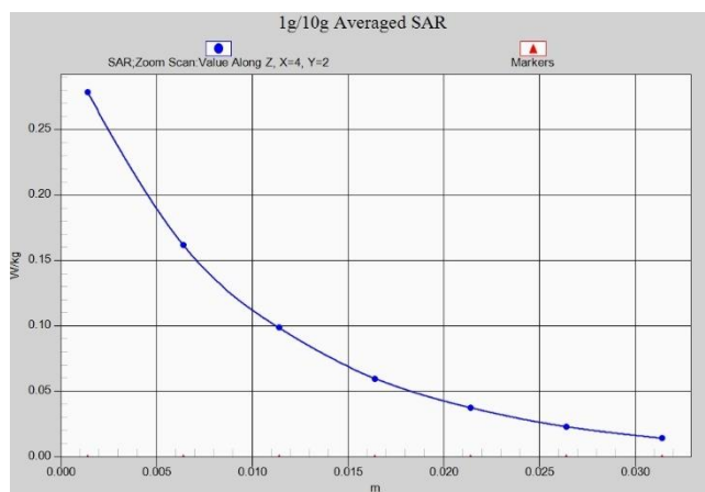
N66 Body 15mm ANT2
