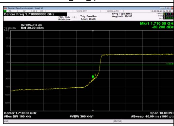
LowRange_FDD04_10MHz_1715_fullRB Low Q16
