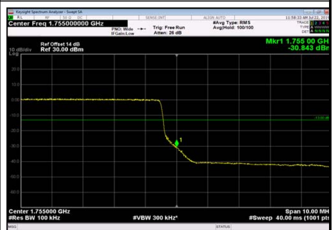
HighRange_FDD04_10MHz_1750_fullRB _High_Q16
