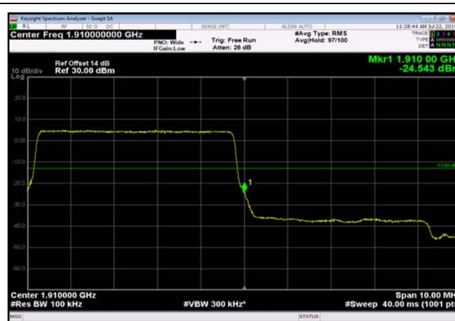
HighRange_FDD02_10MHz_1905_OneRB _high_QPSK
