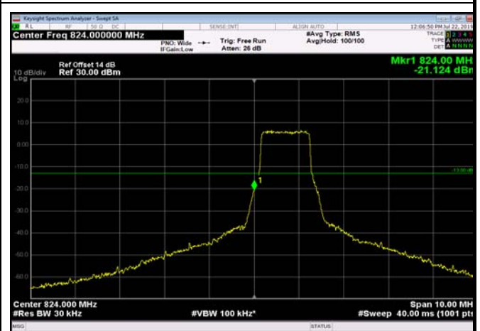
LowRange_FDD05_1.4MHz_824.7_fullRB _Low_Q16
