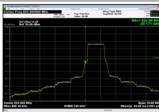
LowRange_FDD05_1.4MHz_824.7_fullRB _Low_QPSK
