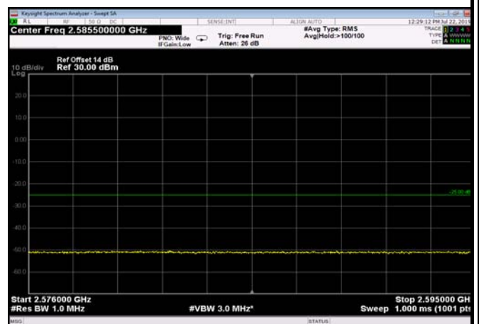
FDD07_5MHz_2502.5_Q16_fullRB_ExtraBan ds_Range_2576~2595
