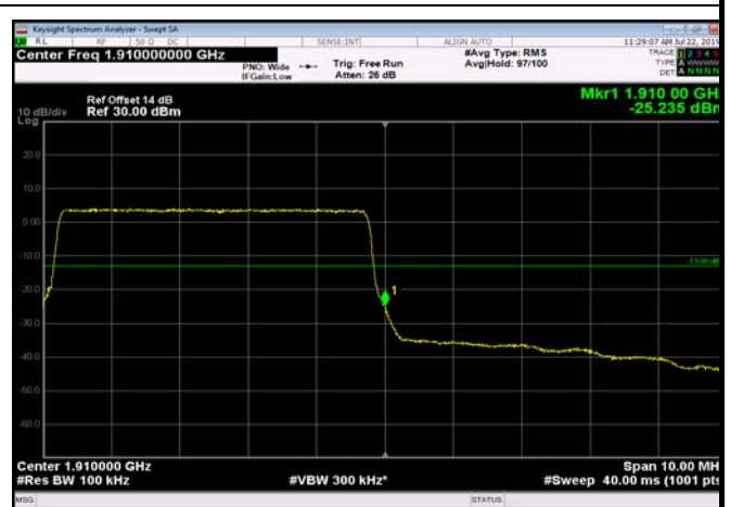
HighRange_FDD02_10MHz_1905_OneRB _high_Q16
