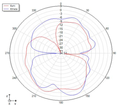
Phi=90 freq=2454MHz
