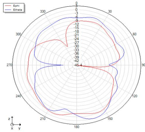
Phi=90 freq=2446MHz
