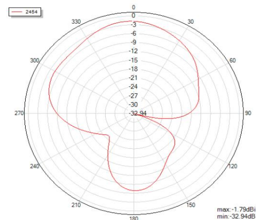
Theta=90 freq=2454MHz
