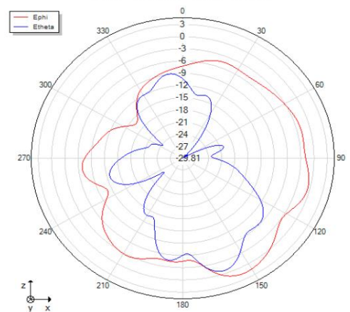
Phi=0 freq=2454MHz
