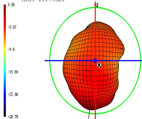
Phi=90 freq=2410MHz
