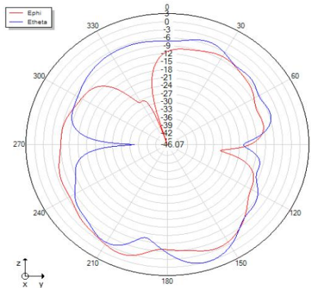
Phi=90 freq=2460MHz
