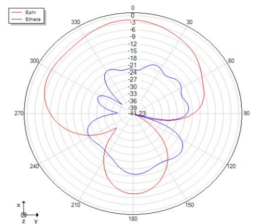
Theta=90 freq=2454MHz
