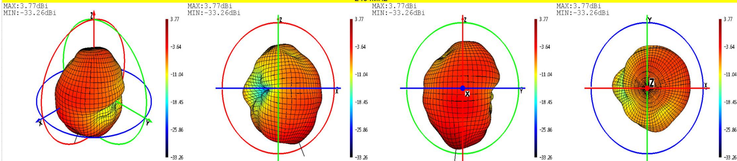
Phi=0 freq=2454MHz
