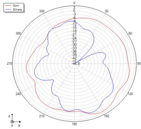
Phi=0 freq=2446MHz
