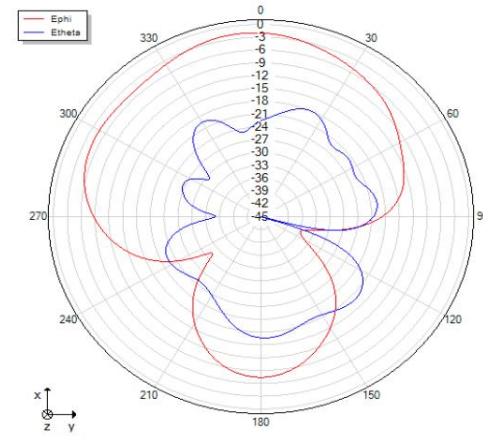
Theta=90 freq=2446MHz
