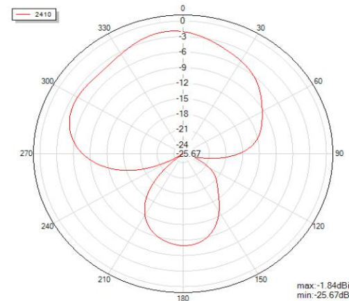
Theta=90 freq=2410MHz
