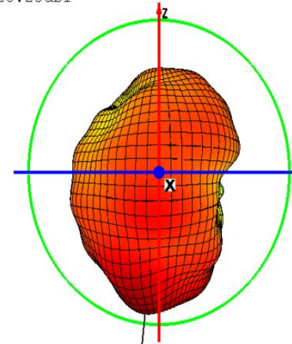
Phi=90 freq=2460MHz
