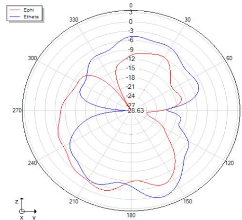
Phi=90 freq=2410MHz
