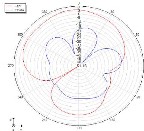
Theta=90 freq=2410MHz
