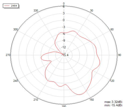
Phi=0 freq=2454MHz
