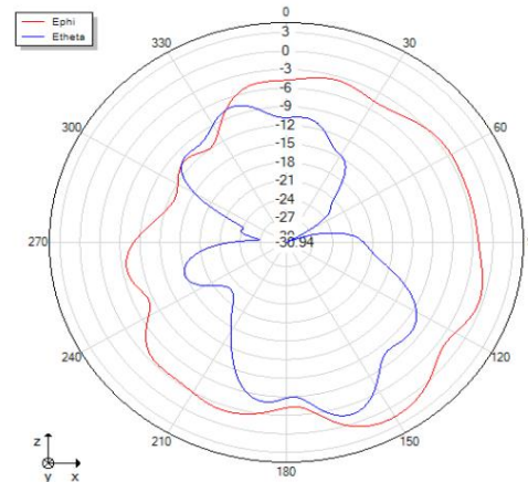
Phi=0 freq=2410MHz
