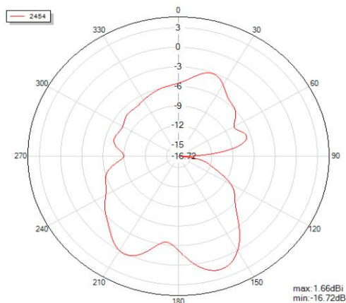
Phi=90 freq=2454MHz
