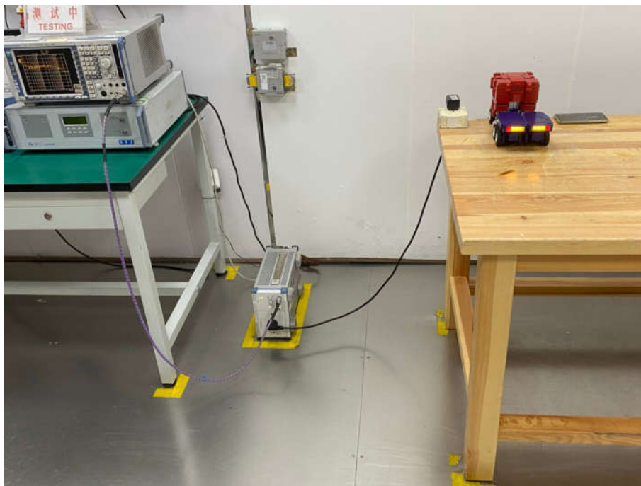
Conducted Emissions Test Setup(adapter 2)
