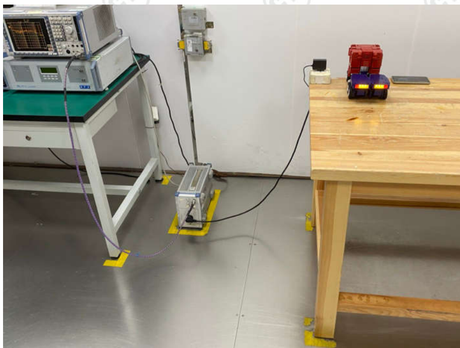
Conducted Emissions Test Setup(adapter 1)
