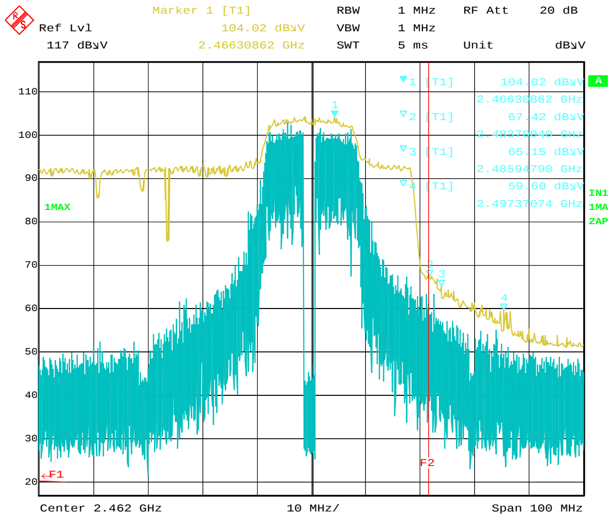
Plot 1-3 Ch.11 2462MHz TX, OFDM 6Mbps (Peak) in Tablet operation mode
