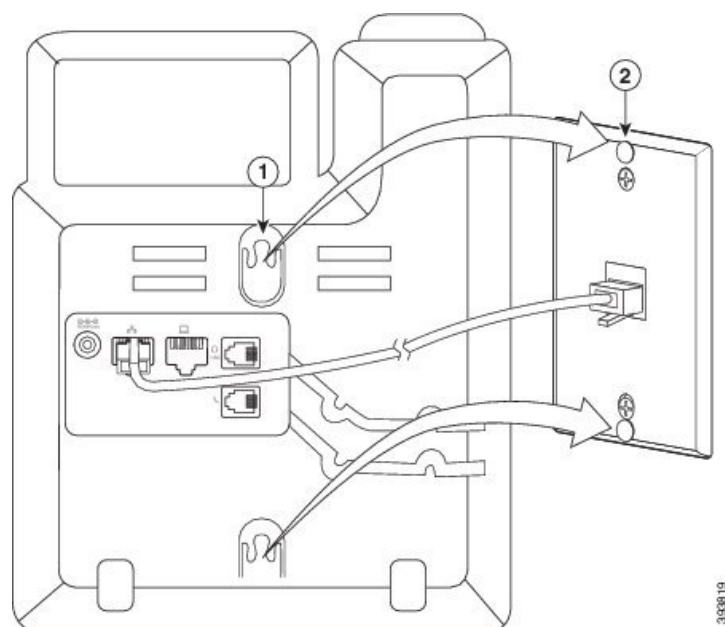
Figure 15: Mounting Holes
