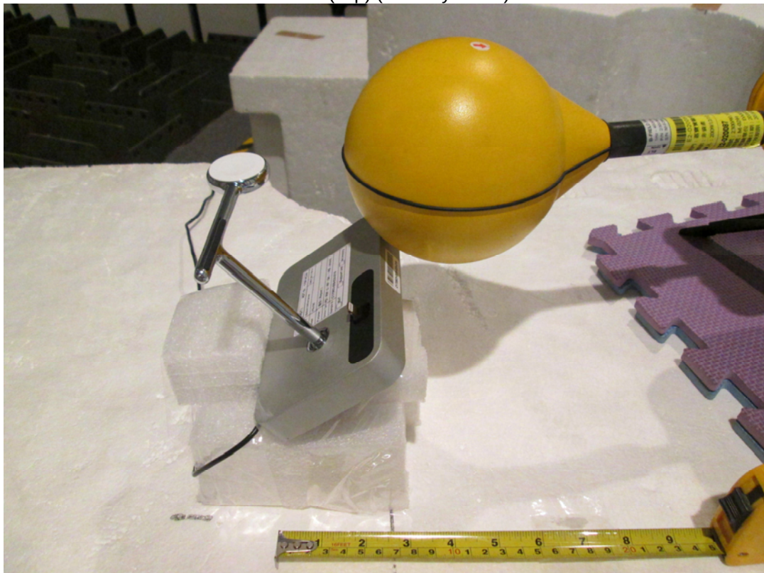
H-Field (Top) (Standby Mode)
