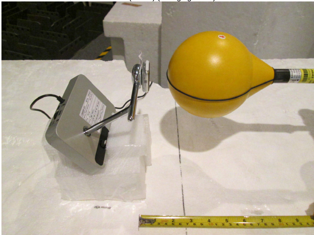
H-Field (Z-axis) (Charging Mode)
