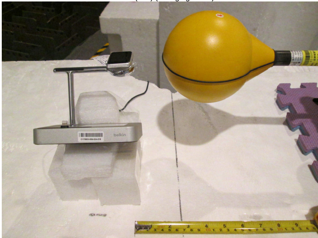
H-Field (Left) (Charging Mode)
