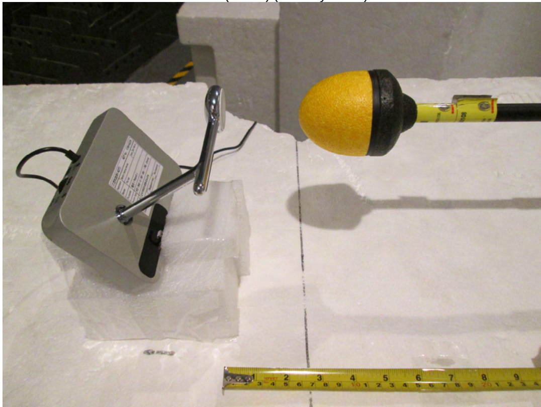
H-Field (Left) (Standby Mode)
