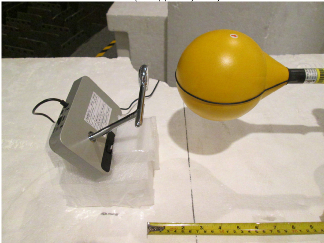
H-Field (Z-axis) (Standby Mode)
