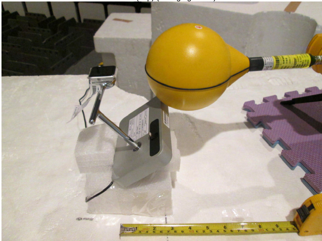
H-Field (Top) (Charging Mode)
