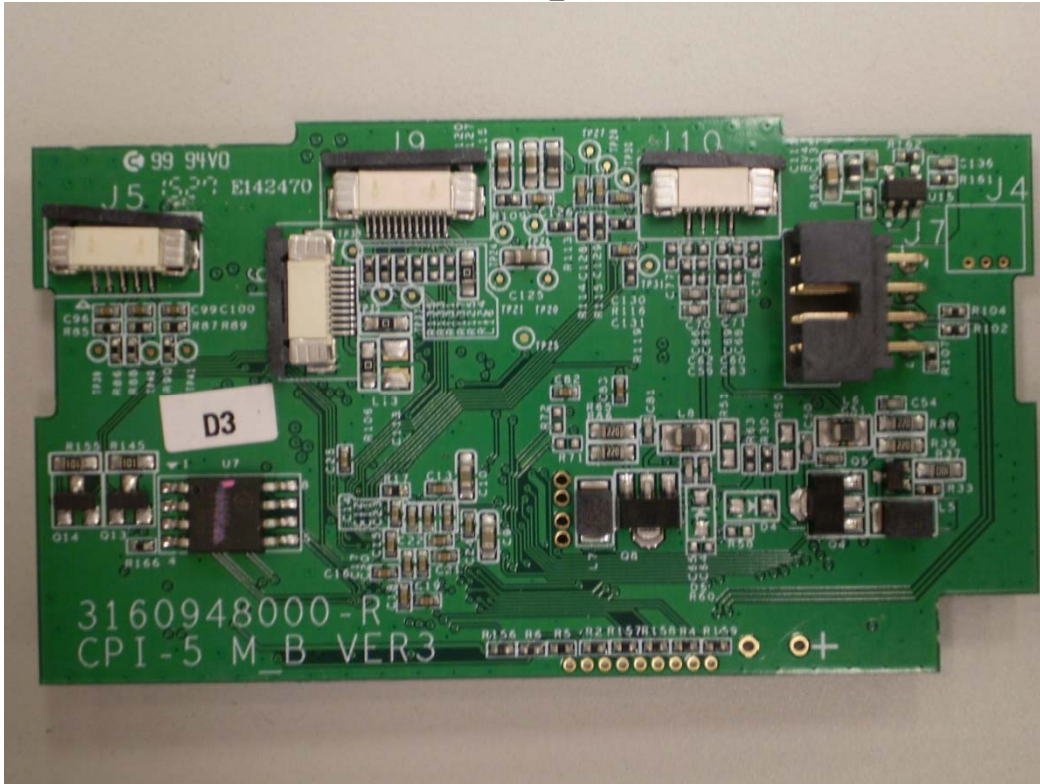
Main PCB_Back
