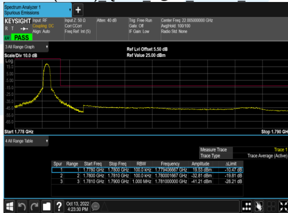
B66(10.0M) 16QAM 1@49 132622 CH
