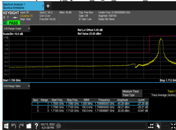
B66(15.0M) 16QAM 1@0 132047 CH
