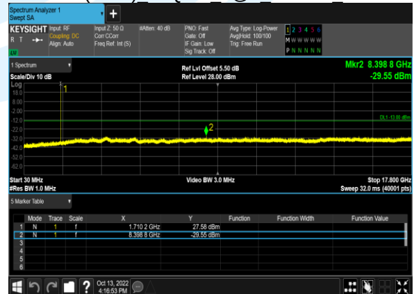
B66(1.4M) 16QAM 1@0 131979 CH
