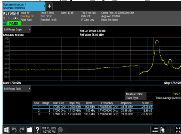
B66(1.4M) 16QAM 1@0 131979 CH
