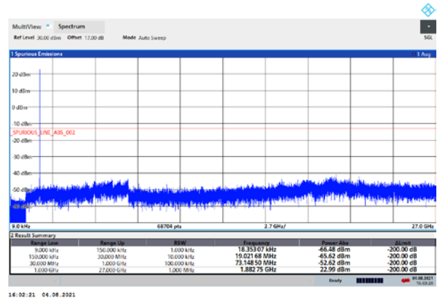
NB-IoT Band 25 CH-High 9kHz~27GHz
