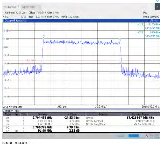
1-N78-3700-3800--30-90-M-9-CP-256QAM-Outer_F ull-245@0-Ant0-87.427-91.080-≤90-PASS
