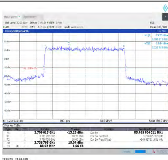
1-N78-3700-3800--30-90-H-2-DFT-PI2BPSK-Outer_ Full-240@0-Ant0-85.466-88.920-≤90-PASS
