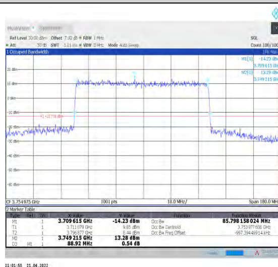
1-N78-3700-3800--30-90-H-3-DFT-16QAM-Outer_Fu ll-240@0-Ant0-85.798-88.920-≤90-PASS
