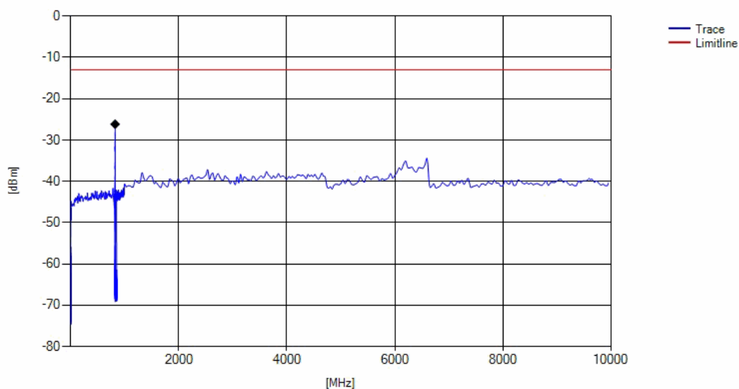
GSM850 Channel=low
