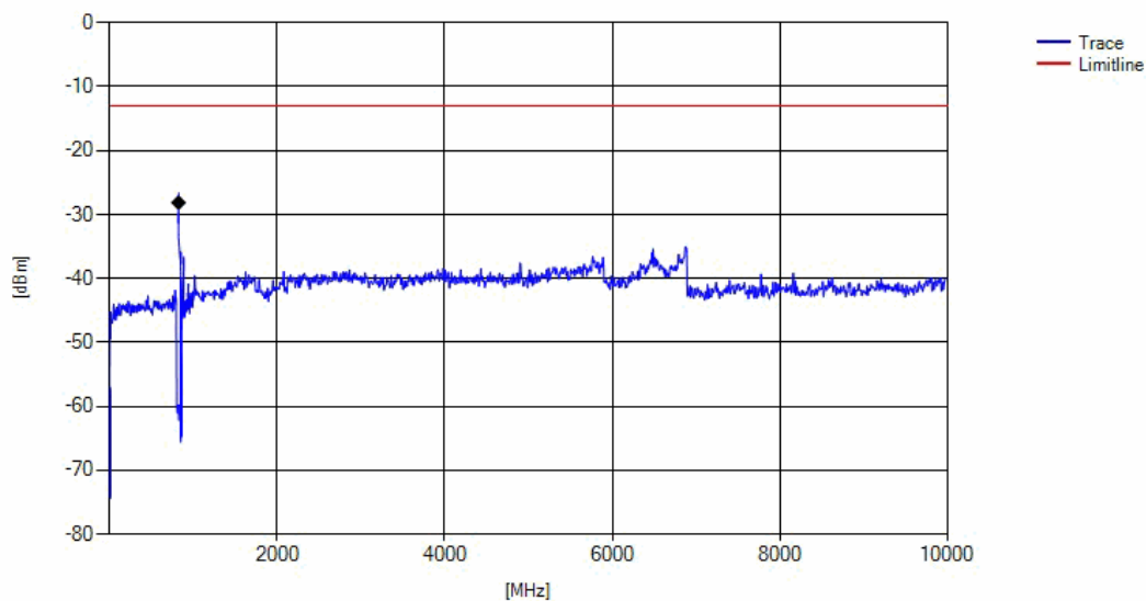
eFDD5 Channel=high
