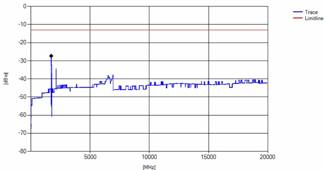
eFDD4 Channel=high
