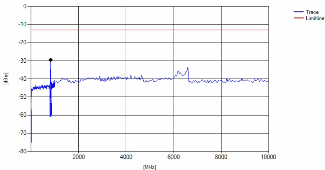
HSUPA Channel=low
