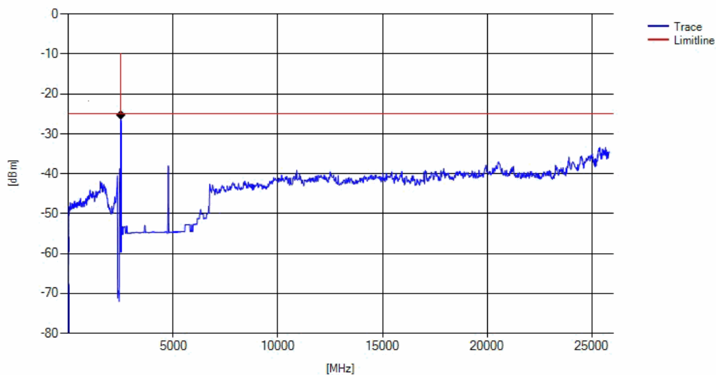
eFDD7 Channel=low
