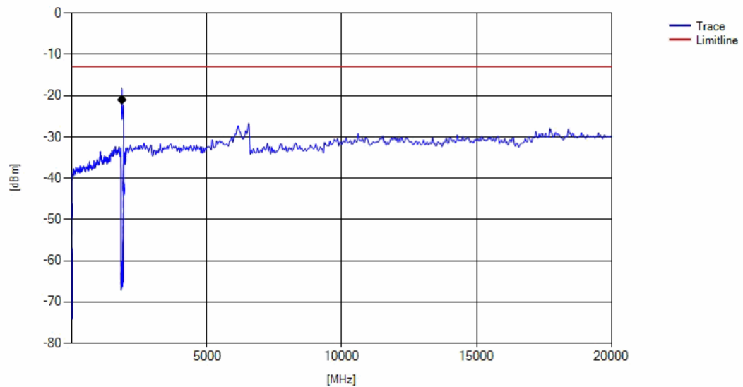
GSM1900 Channel=high
