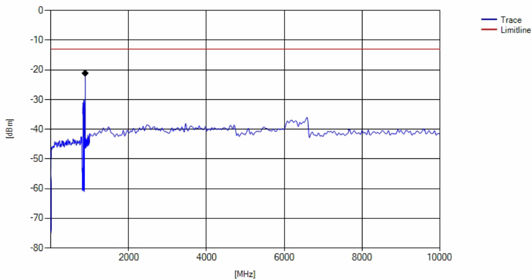
HSDPA Channel=High
