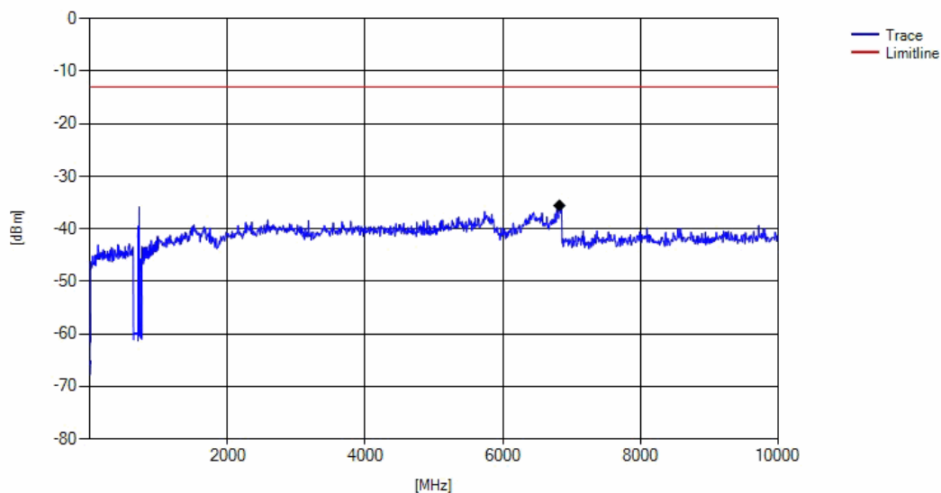
eFDD12 Channel=high
