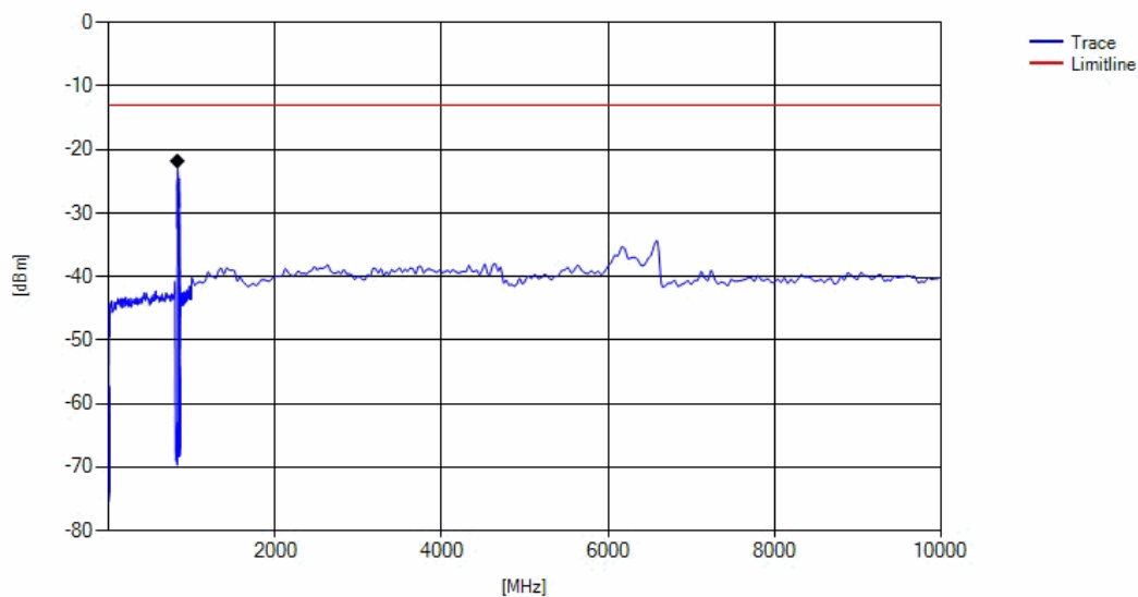
EDGE850 Channel=Low
