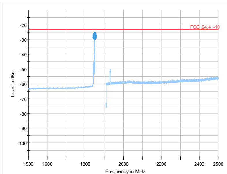
Final scan
