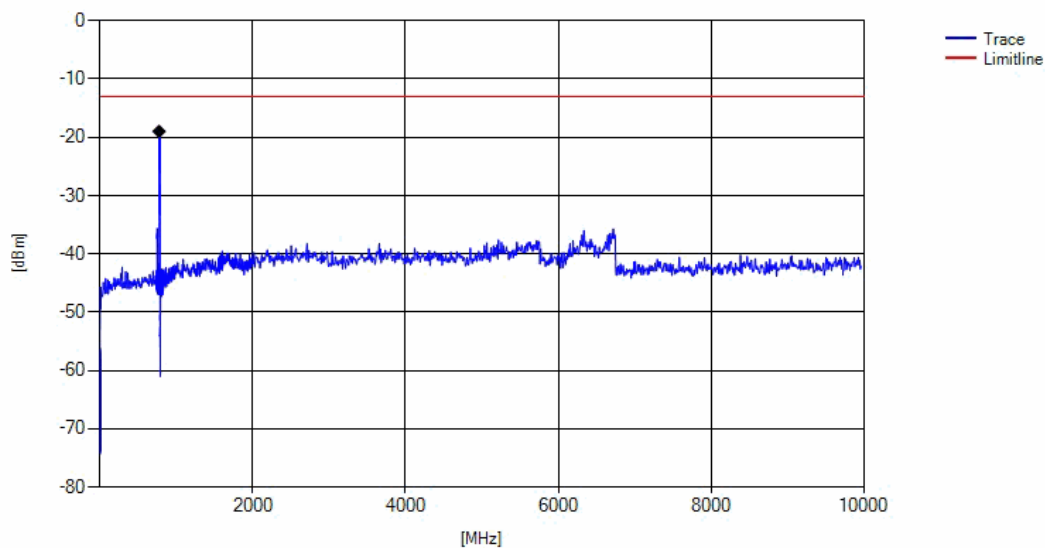
eFDD13 Channel=high
