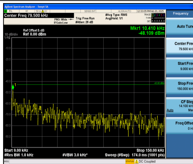
Band25_15MHz_16QAM_26365_1RB#0_0.009~0.15_0.009~0.15
