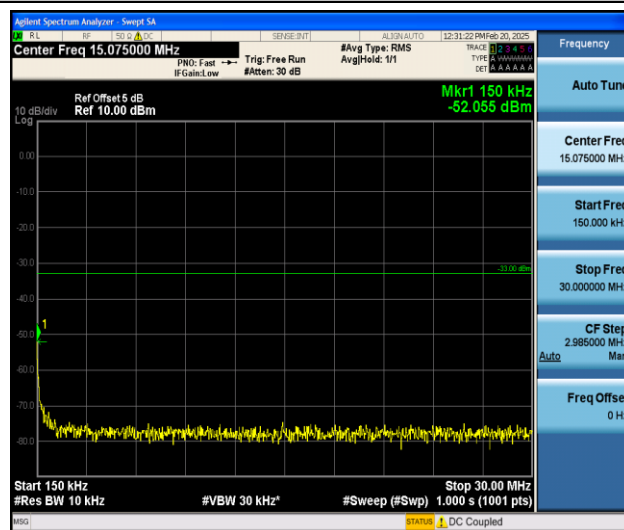
Band25_15MHz_16QAM_26115_1RB#0_0.15~30_0.15~30
