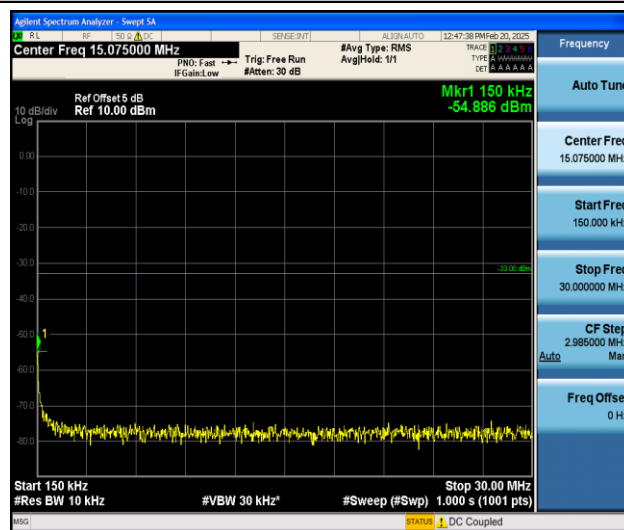
Band25_20MHz_16QAM_26140_1RB#0_0.15~30_0.15~30
