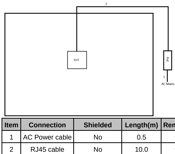
Test Setup Diagram - Radiated Test _PoE mode
