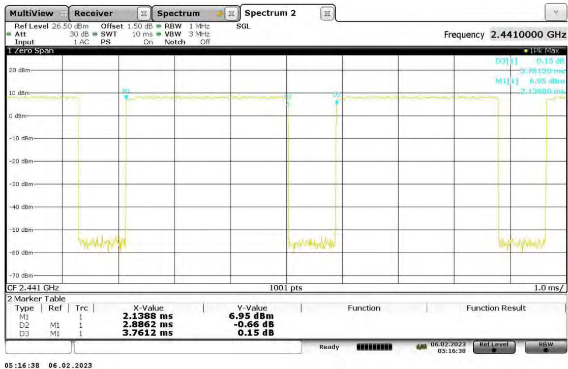
2DH5_Ant1_2441
