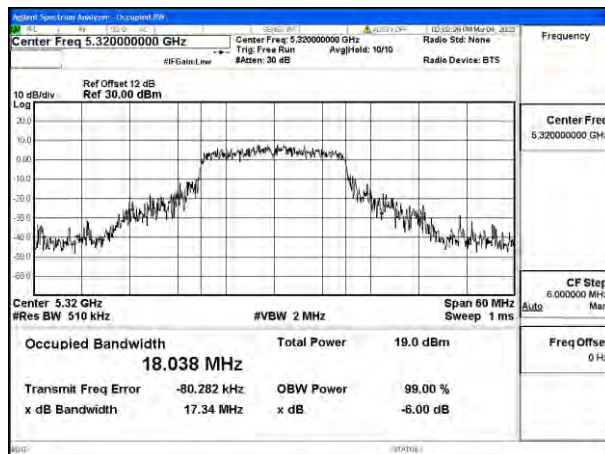
Mode:802.11n HT20 Frequency:5320MHz Ant:Chain0
