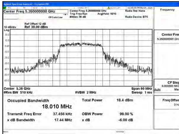
Mode:802.11n HT20 Frequency:5260MHz Ant:Chain0
