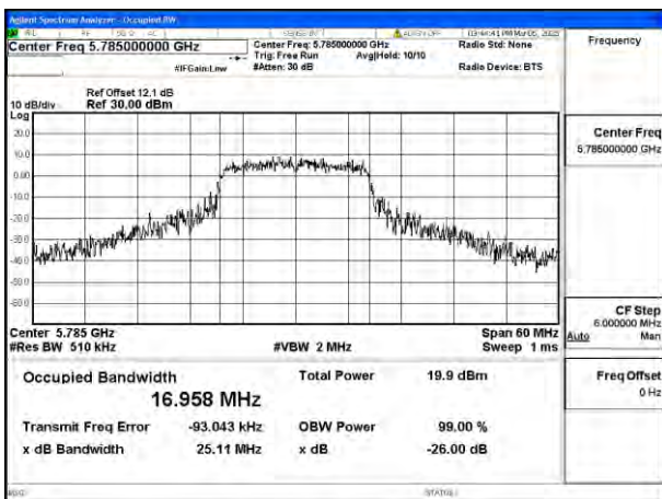
Mode:802.11a Frequency:5785MHz Ant:Chain1
