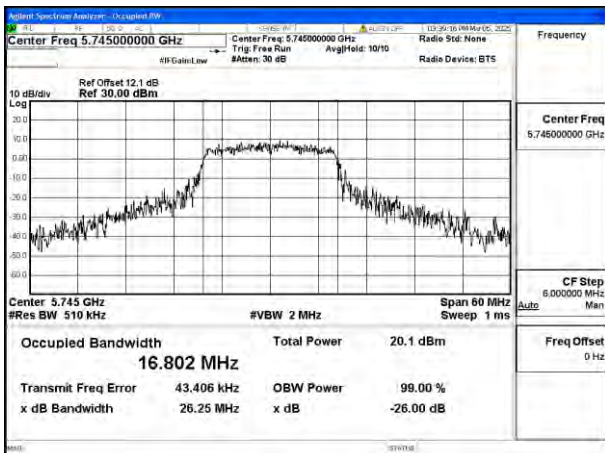
Mode:802.11a Frequency:5745MHz Ant:Chain0
