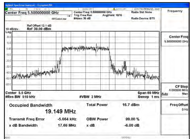
Mode:802.11ax HE20 Frequency:5500MHz Ant:Chain1
