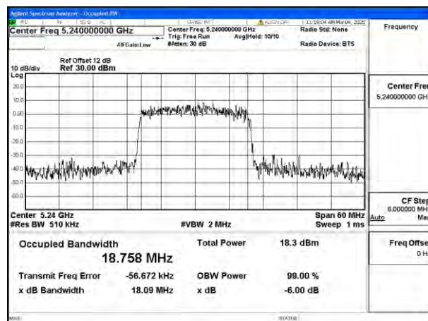
Mode:802.11ax HE20 Frequency:5240MHz Ant:Chain1
