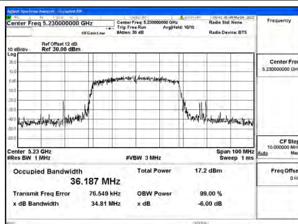
Mode:802.11n HT40 Frequency:5230MHz Ant:Chain0
