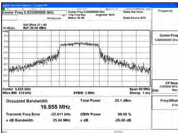
Mode:802.11a Frequency:5825MHz Ant:Chain0
