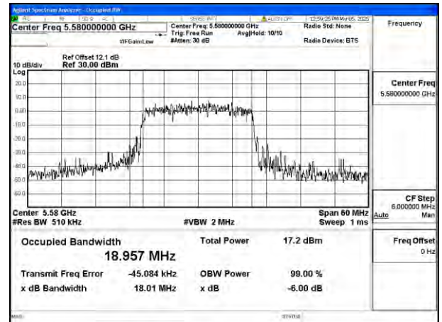
Mode:802.11ax HE20 Frequency:5580MHz Ant:Chain0
