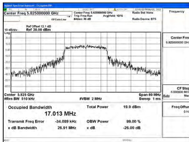
Mode:802.11a Frequency:5825MHz Ant:Chain1
